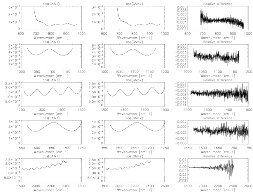
Figure 9 The same as Figure 6 but for a subsequent gain measurement.
