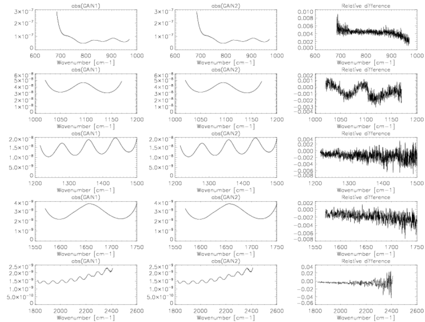
Figure 6 Relative variations of radiometric gain for consecutive disseminated gains in band A for the forward and reverse direction.
