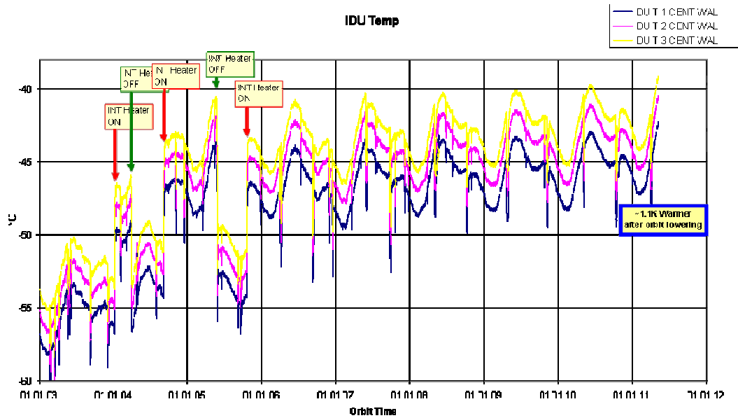
Figure 1 - IDU temperatures since November 2002 (courtesy of Astrium).
