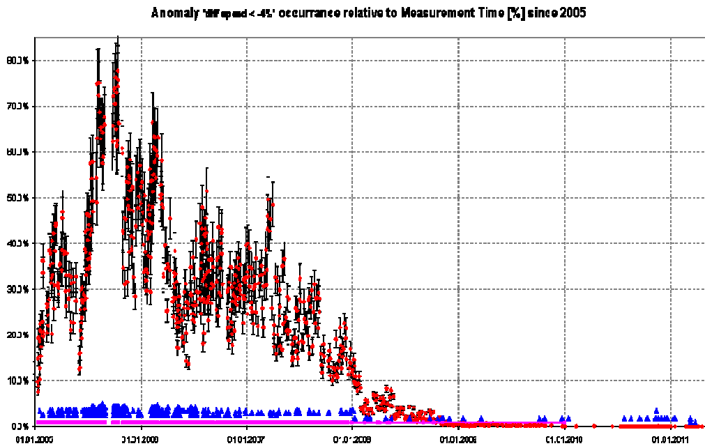
Figure 3 Occurrence of -4% differential speed error relative to measurement time since 2005 (courtesy of Astrium).
