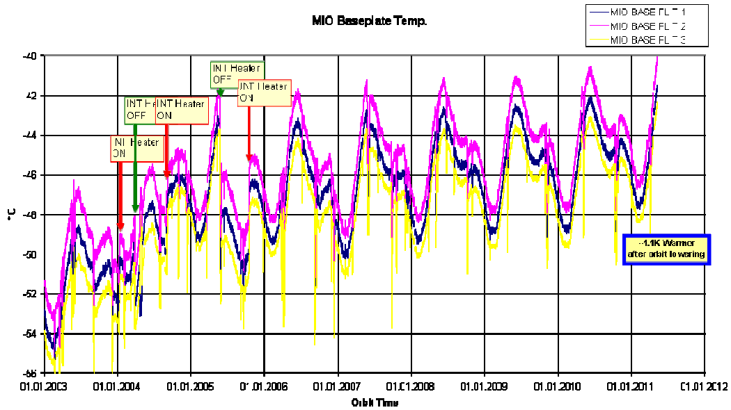
Figure 2 - MIO base plate temperatures since November 2002 (courtesy of Astrium).
