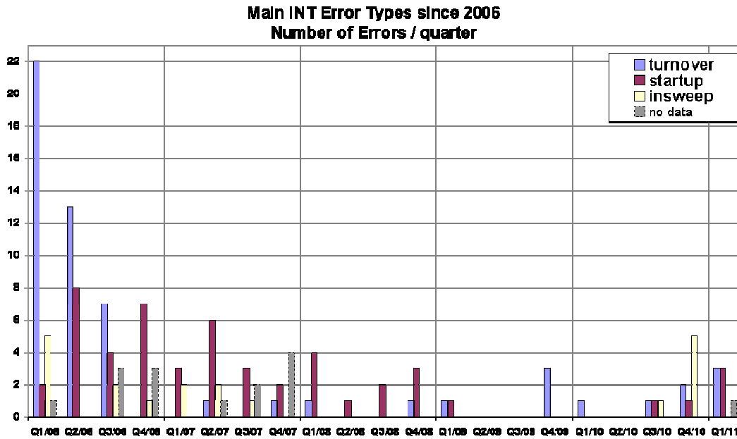
Figure 4 Main INT error types since 2006 (courtesy of Astrium).
