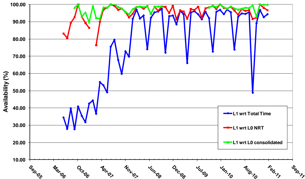
Figure 12 – MIPAS L1 off-line data at D-PAC: long term statistics since Jun 2006.
