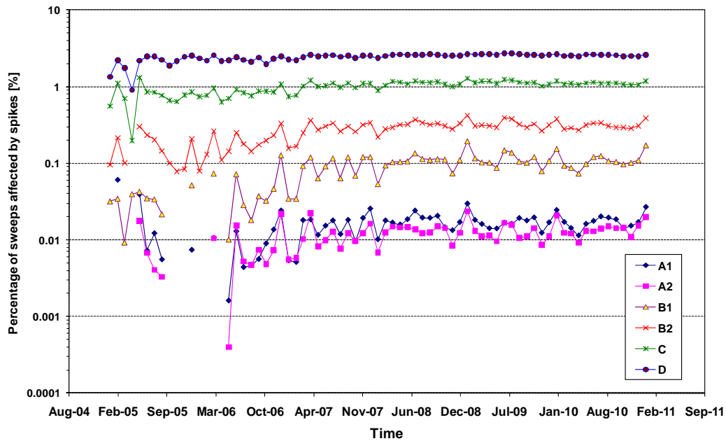
Figure 19 MIPAS long-term monitoring of spikes: percentage of spike-affected sweeps.
