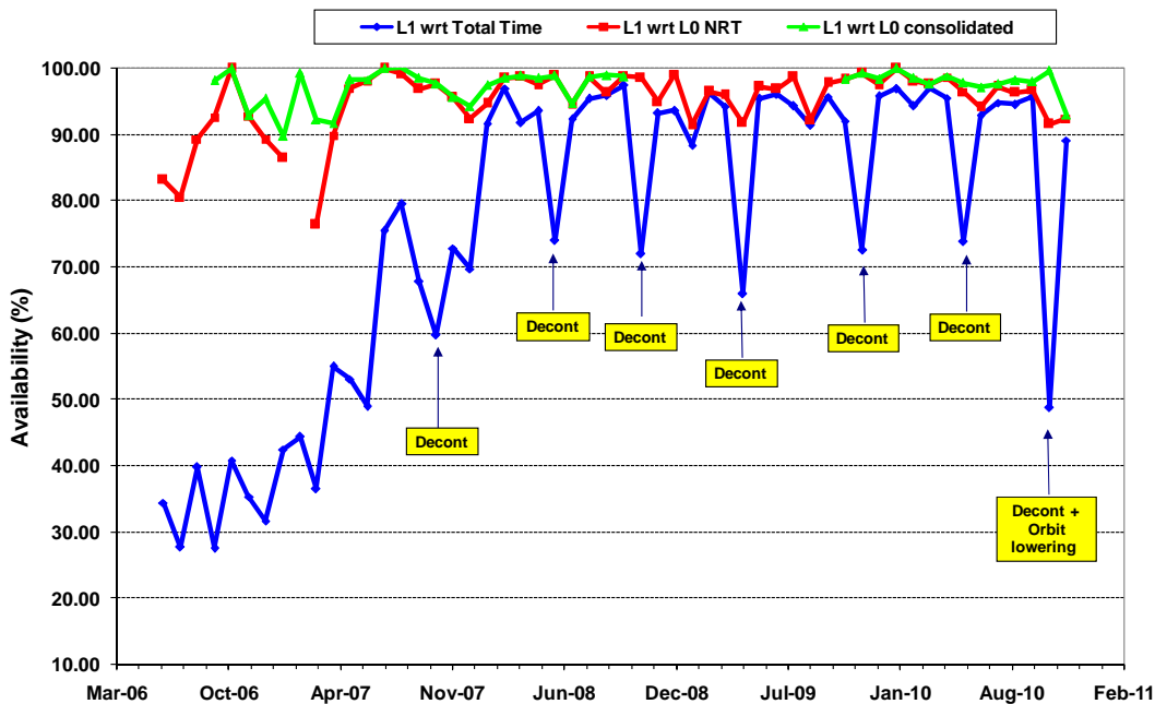
Figure 12 – MIPAS L1 off-line data at D-PAC: long term statistics since Jun 2006.
