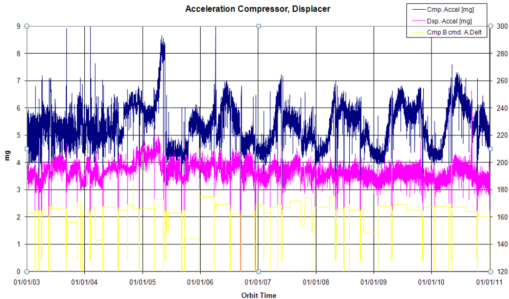
Figure 5 Cooler Displacer and Compressor vibration level, historical trend since 2005 (courtesy of Astrium).
