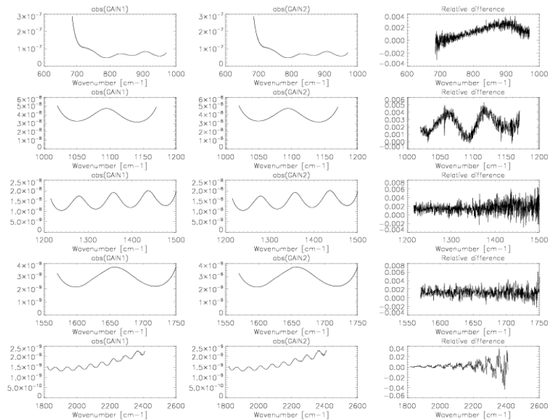
Figure 6 Relative variations of radiometric gain for consecutive disseminated gains in band A for the forward and reverse direction. The first two plots in each row are the complex modulus of the gain for each of the 5 MIPAS bands, the third plot is the ratio: [abs(GAIN2)-abs(GAIN1)]/abs(GAIN1) .
