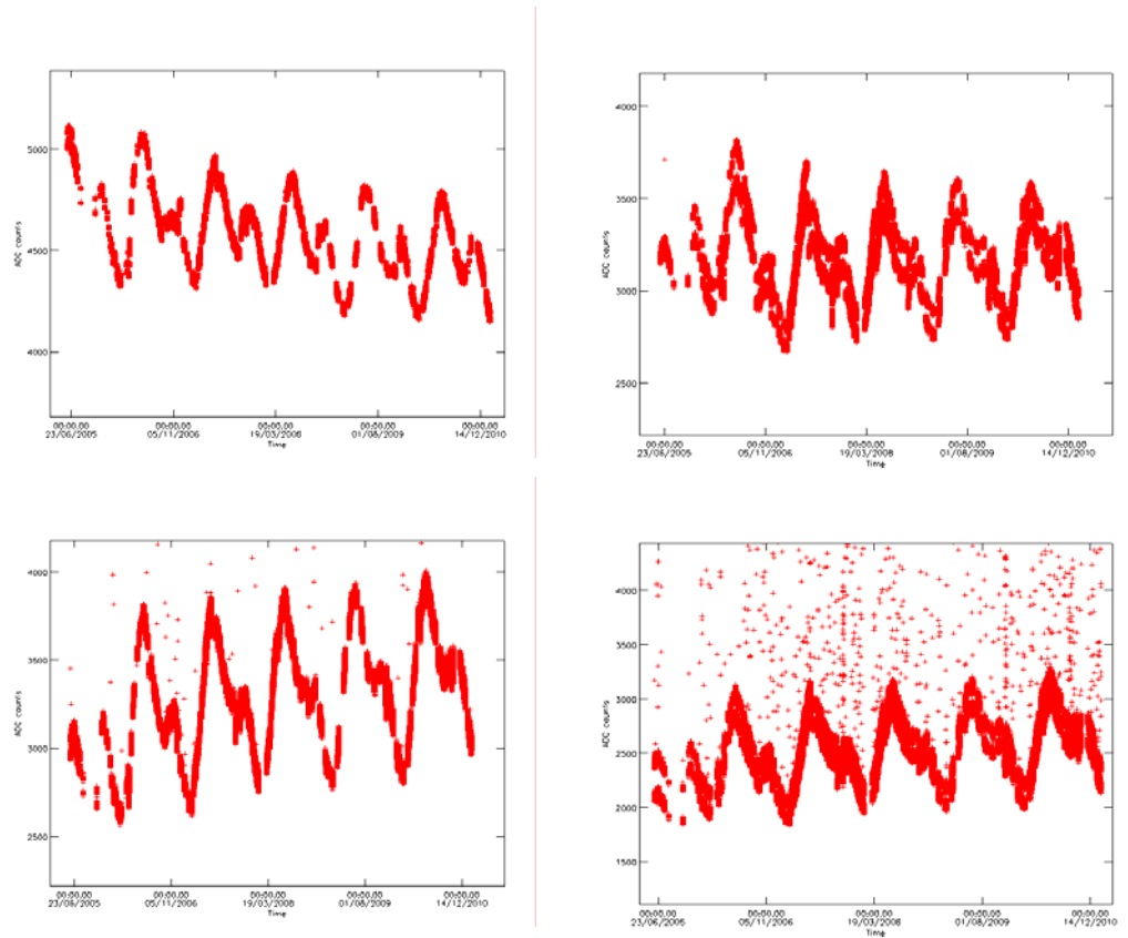
Figure 18 ADC max counts in channel A2, B2, C2 and D2 during DS measurements since June 2005.
