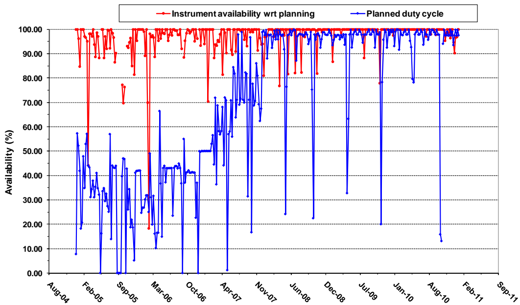
Figure 11 – MIPAS instrument availability w.r.t. planning and planned duty cycle.
