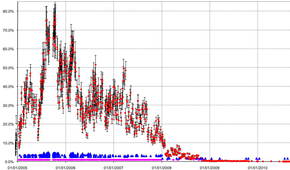
Figure 3 Occurrence of -4% differential speed error relative to measurement time since 2005 (courtesy of Astrium).
