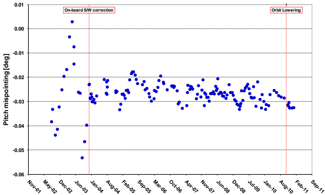
Figure 15 MIPAS long-term pointing error as a function of time since September 2002.
