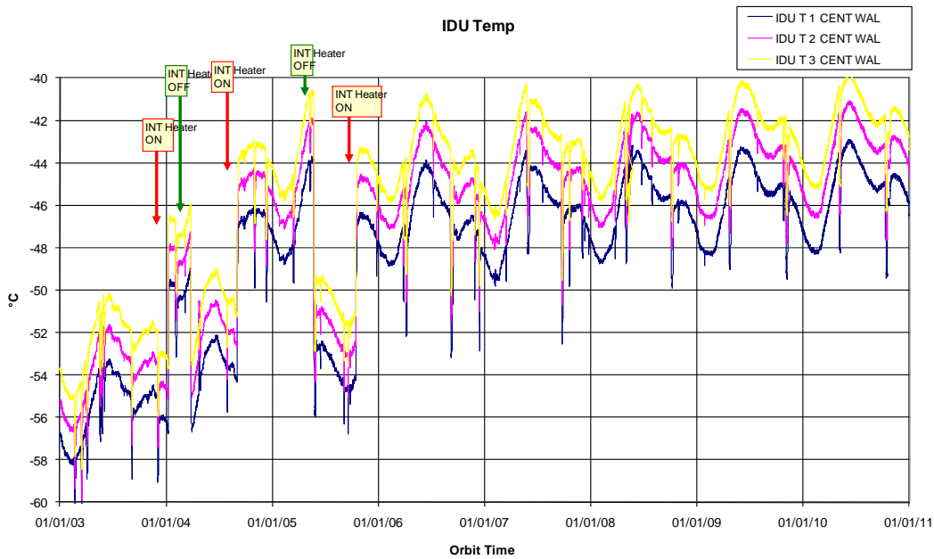
Figure 1 - IDU temperatures since November 2002 (courtesy of Astrium).
