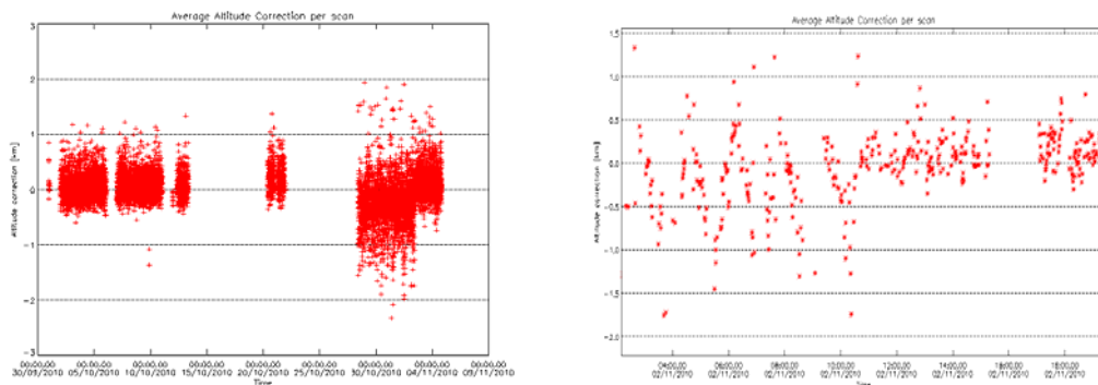
Figure 23 – MIPAS altitude correction in the Level 2 processing averaged over a scan during October 2010 and zoom at the time when the ENVISA SYSM was resumed after the orbit lowering.
