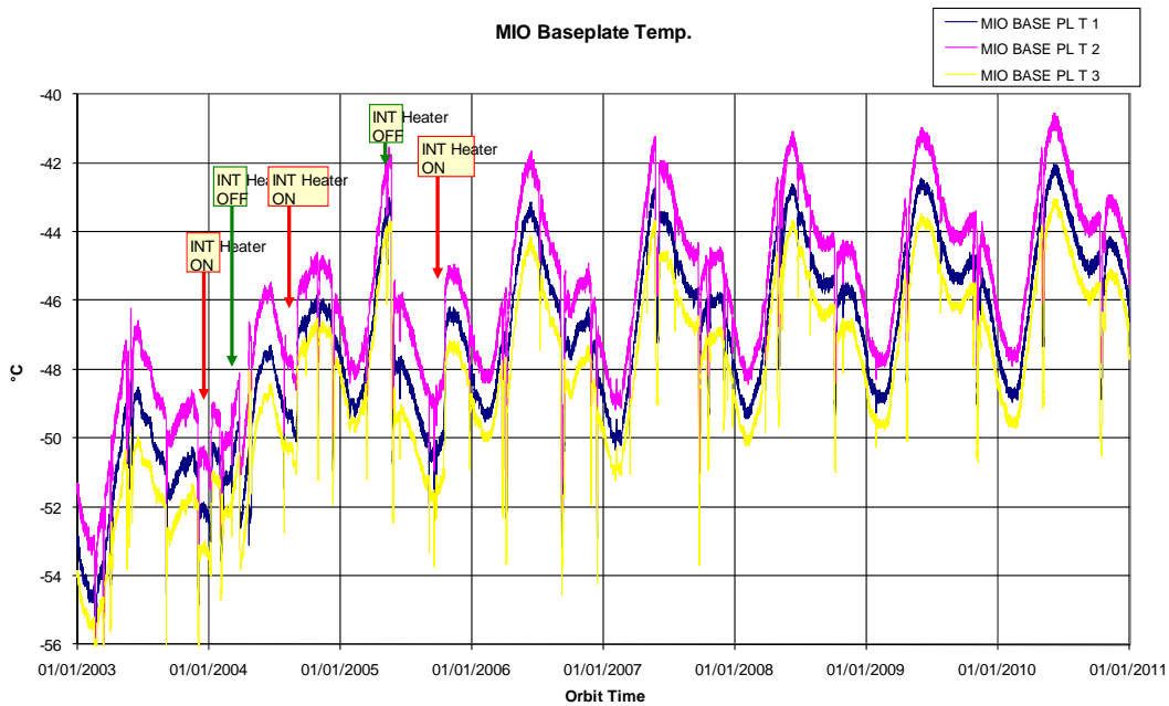
Figure 2 - MIO base plate temperatures since November 2002 (courtesy of Astrium).
