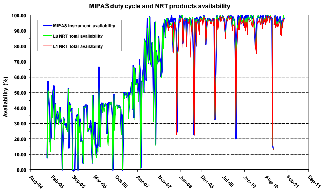
Figure 10 – MIPAS L0 NRT long term statistics since Jan 2005.
