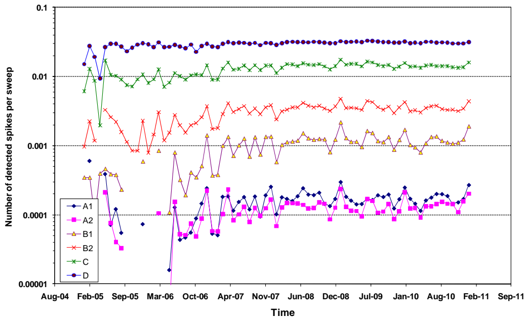
Figure 20 MIPAS long-term monitoring of spikes: number of detected spikes per sweep.
