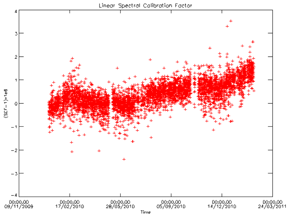
Figure 16 MIPAS Spectral Calibration Factor (SCF) since Jan 2010.
