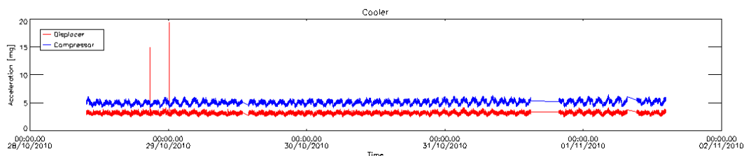
Figure 22 – MIPAS cooler acceleration level after the ENVISAT orbit lowering.
