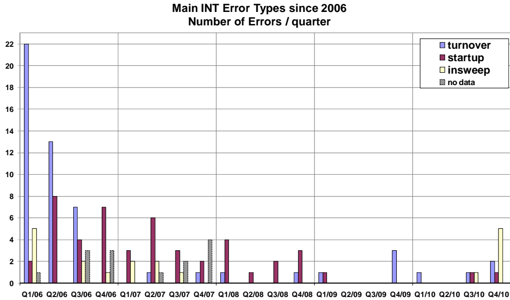
Figure 4 Main INT error types since 2006 (courtesy of Astrium).
