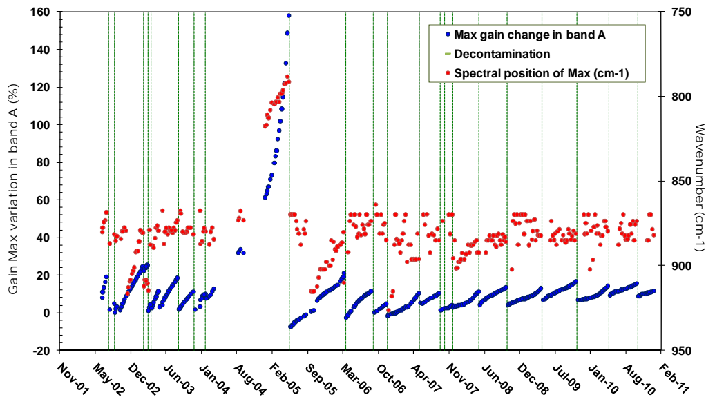
Figure 14 Gain accumulation increase since January 2005.
