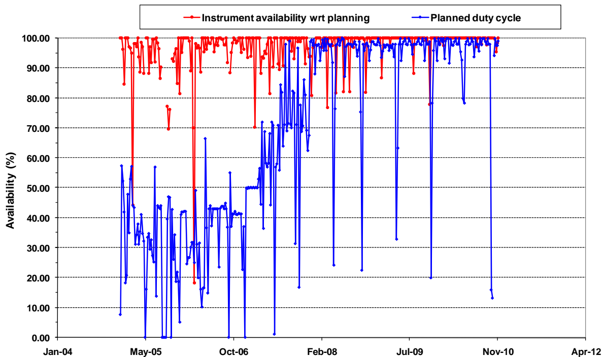
Figure 5 – MIPAS instrument availability w.r.t. planning and planned duty cycle.
