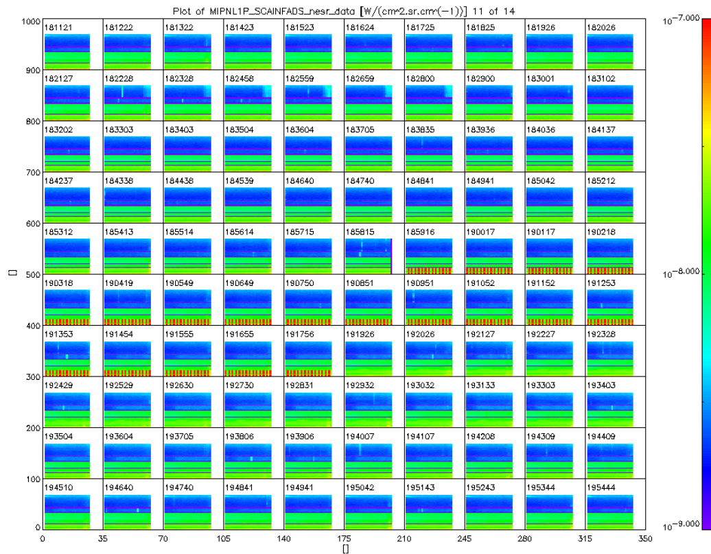
Figure 40 NESR value during 23 Jun 2008. The red stripes show the anomalous high NESR values in band A for orbit 33019.
