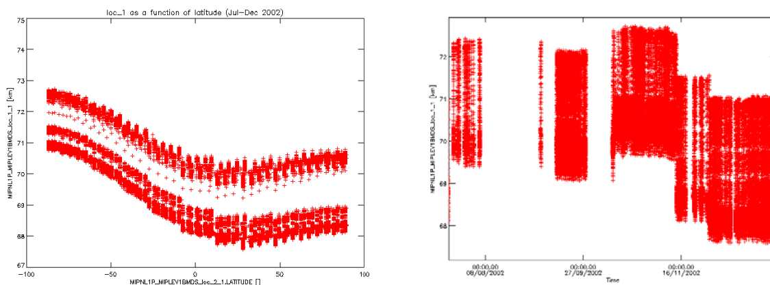
Figure 46 MIPAS engineering tangent altitude as written in the L1b files (loc_1 field) as a function of latitude and time.
