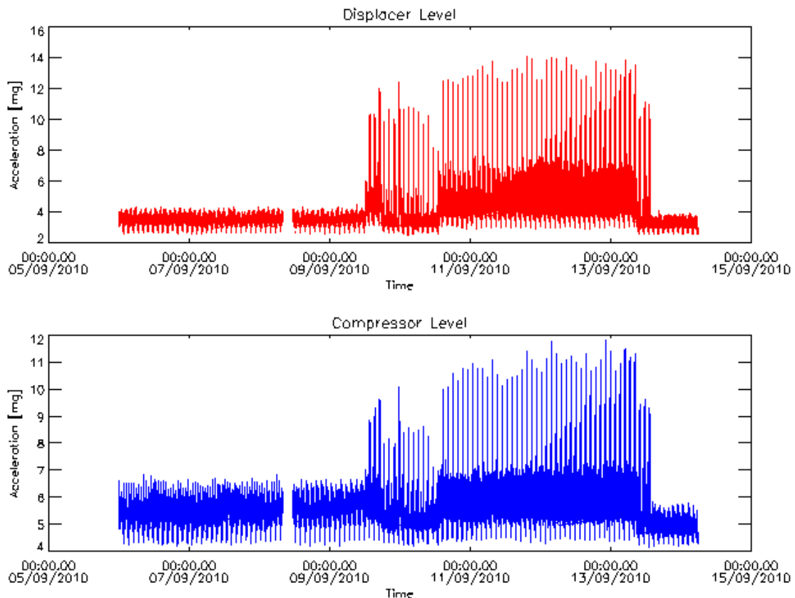
Figure 9 Anomaly on the Cooler Displacer and Compressor vibration level during Sep 2010.
