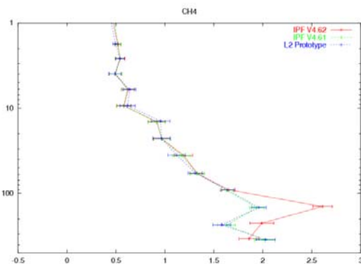
Figure 43 Temperature N 2 O and CH 4 profiles as a function of pressure retrieved with IPF 4.62 and 4.61 compared to the prototype for seq. 16 of orbit 2975. The 4.61 profile is the reference, validated by a IMK balloon flight.
