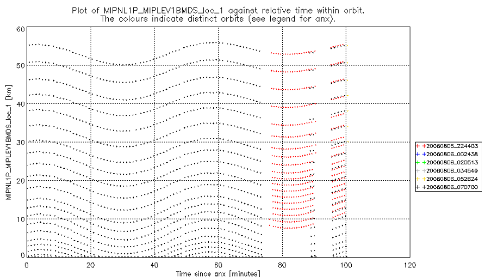
Figure 39 Altitude scan as a function of ANX for the orbit measured on 8 Jun 2006.
