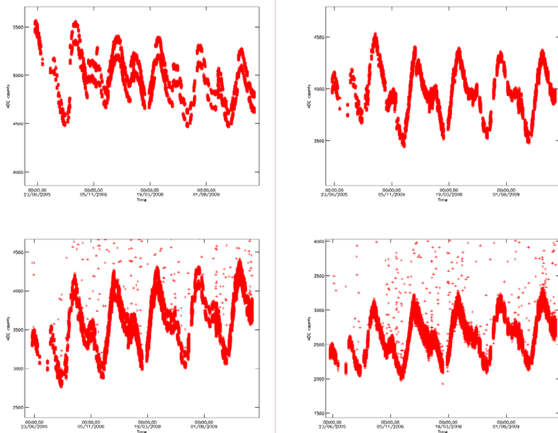
Figure 10 ADC max counts in channel A1, B1, C1 and D1 during DS measurements since June 2005.
