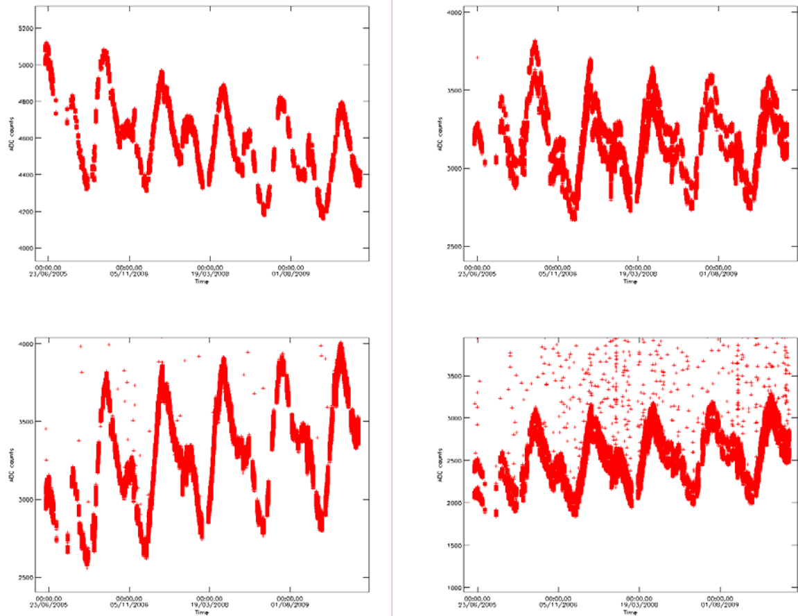
Figure 11 ADC max counts in channel A2, B2, C2 and D2 during DS measurements since June 2005.
