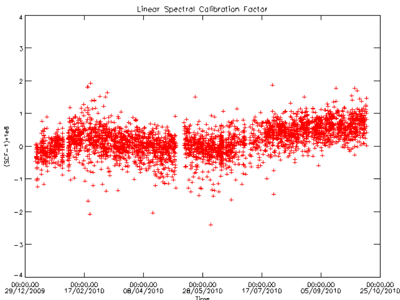
Figure 12 MIPAS Spectral Calibration Factor (SCF) since Jan 2010.
