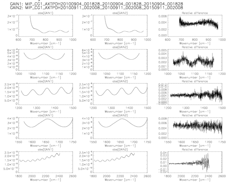
Figure 14 The same as Figure 13 but for a gain measured on 10 Sep 2010.
