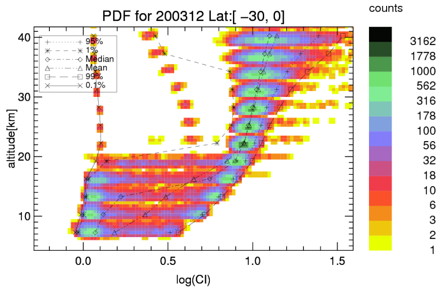
Figure 42 Cloud Index in band A for MIPAS L1b radiances of Dec 2003. Above 20 km we noticed unrealistic low CI.
