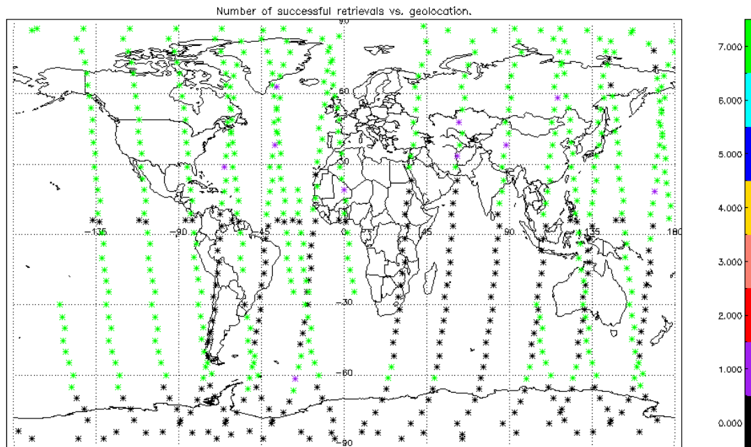
Figure 45 MIPAS number of successful retrieval for 25 July 2002. Note that 7 is the nominal value corresponding to the target species of the ESA MIPAS products. Zero value means that the retrieval fails already at the p-T stage.
