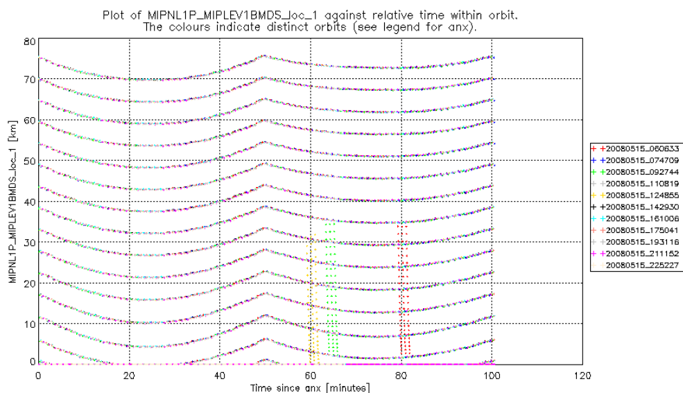
Figure 38 Altitude scan as a function of ANX for the orbit measured on 15 May 2008. The three series of scans in the figure are the volcanic emission mode measured during this day.
