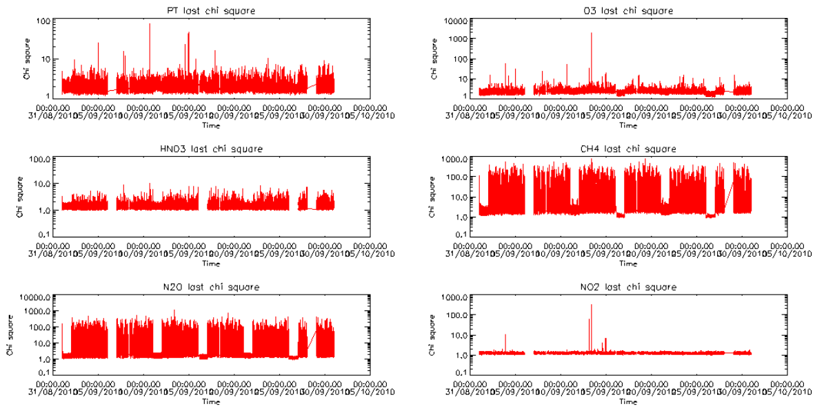
Figure 25 MIPAS last chi square values for NRT retrieval parameters.
