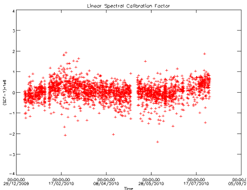
Figure 11 MIPAS Spectral Calibration Factor (SCF) since Jan 2010.
