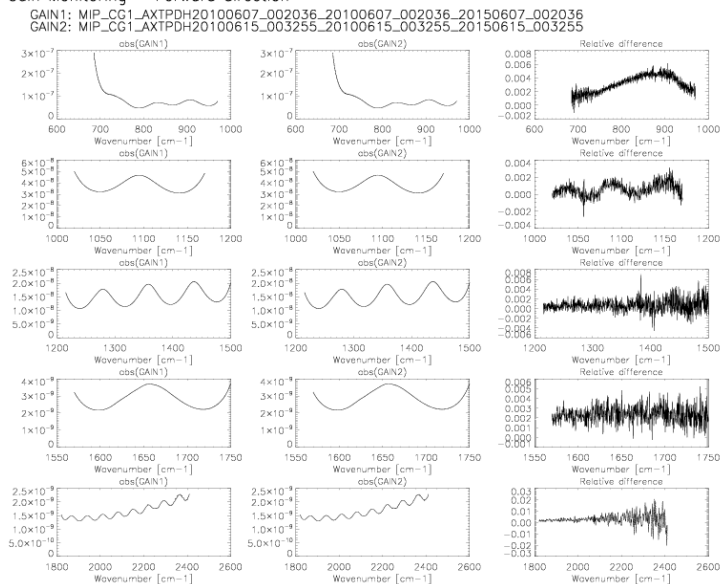
Figure 13 The same as Figure 12 but for a gain measured on 14 Jun 2010.
