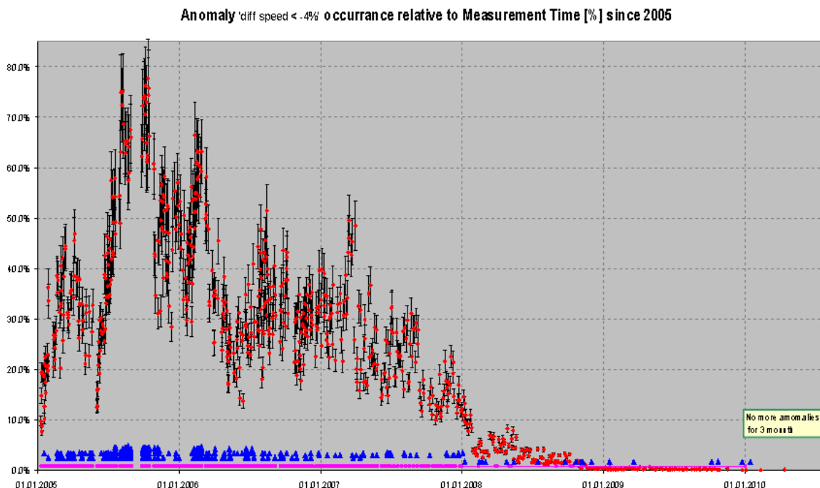
Figure 6 Occurrence of -4% differential speed error relative to measurement time since 2005 (courtesy of Astrium).
