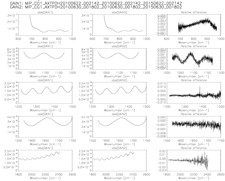
Figure 15 The same as Figure 12 but for a gain measured on 29 Jun 2010.
