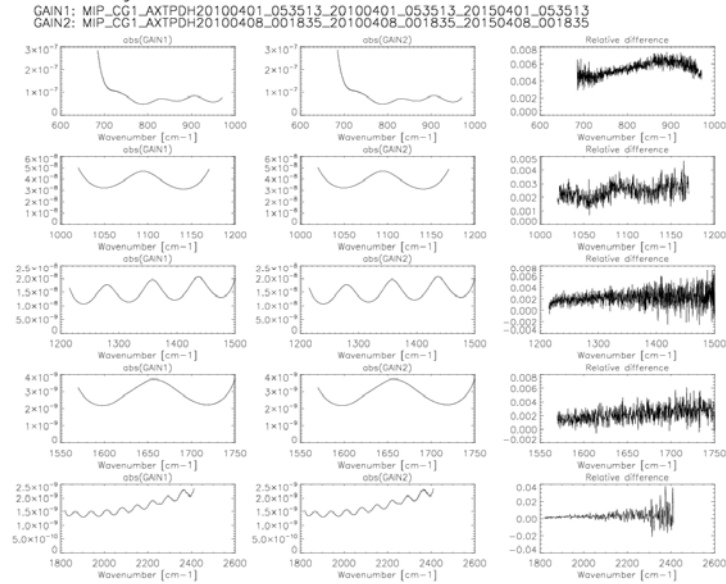
Figure 13 The same as Figure 12 but for a gain measured on 7 Apr 2010.
