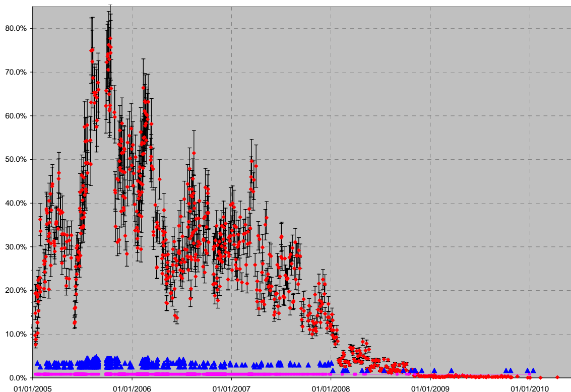
Figure 6 Occurrence of -4% differential speed error relative to measurement time since 2005 (courtesy of Astrium).
