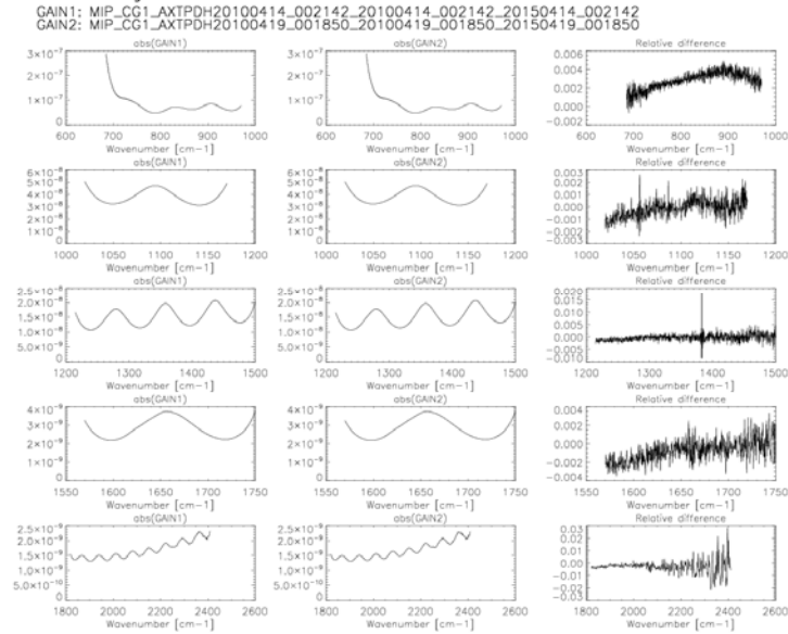
Figure 15 The same as Figure 12 but for a gain measured on 18 Apr 2010.
