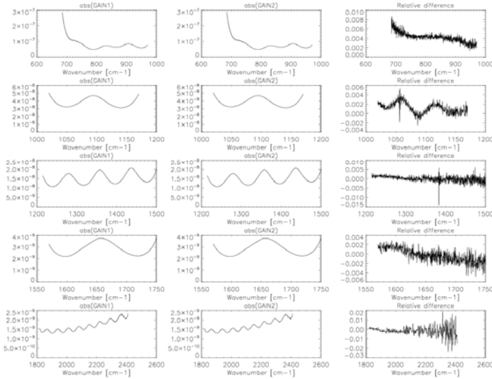
Figure 14 The same as Figure 12 but for a gain measured on 13 Apr 2010.
