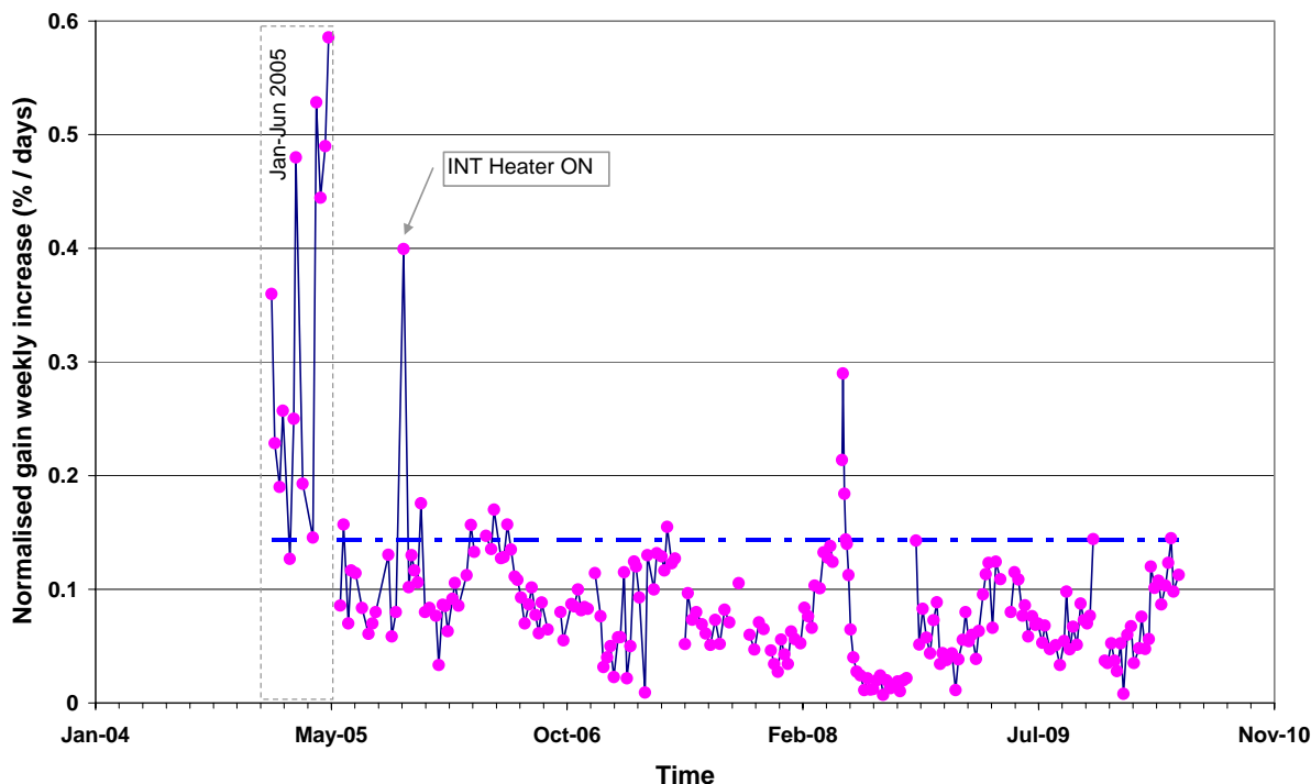
Figure 17 Gain maximum increase normalized to the time difference between consecutive disseminated gains since January 2005. The blue line represents the expected gain increase (1%/week).
