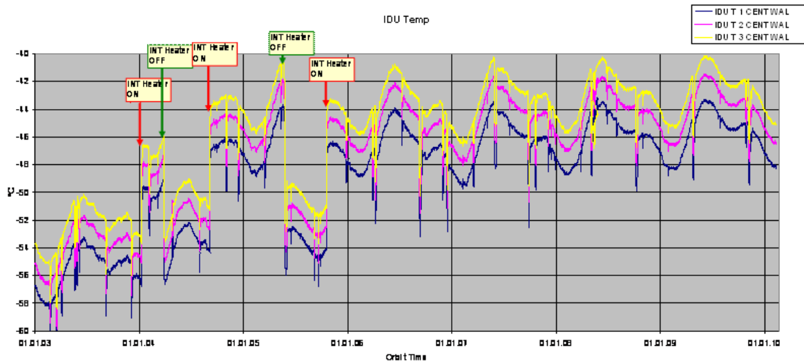
Figure 4 - IDU temperatures as a function of time since November 2002 (courtesy of Astrium).
