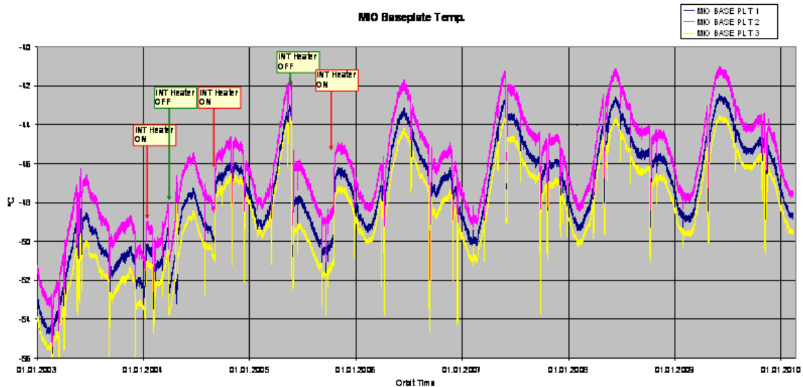
Figure 5 - MIO base plate temperatures as a function of time since November 2002 (courtesy of Astrium).
