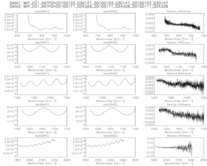
Figure 12 The same as Figure 11 but for a gain measured on 10 Jan 2010.
