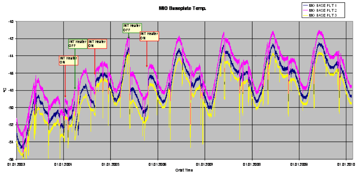
Figure 5 - MIO base plate temperatures as a function of time since November 2002 (courtesy of Astrium).
