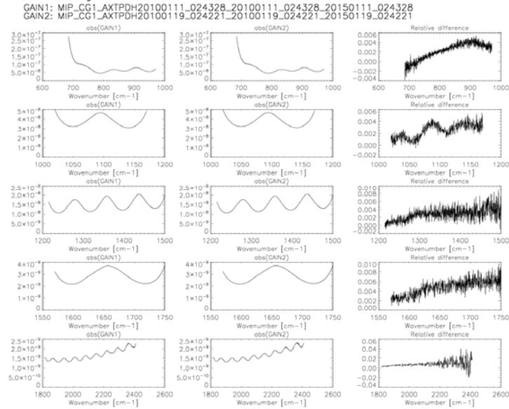
Figure 13 The same as Figure 11 but for a gain measured on 18 Jan 2010.
