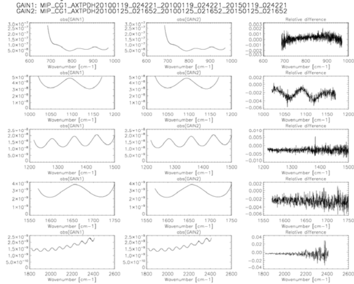
Figure 14 The same as Figure 11 but for a gain measured on 24 Jan 2010.
