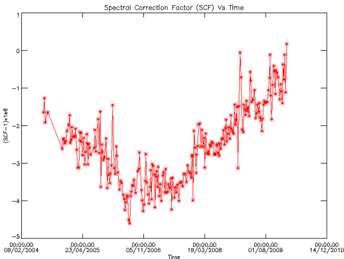
Figure 10 MIPAS Spectral Calibration Factor (SCF) since August 2004.
