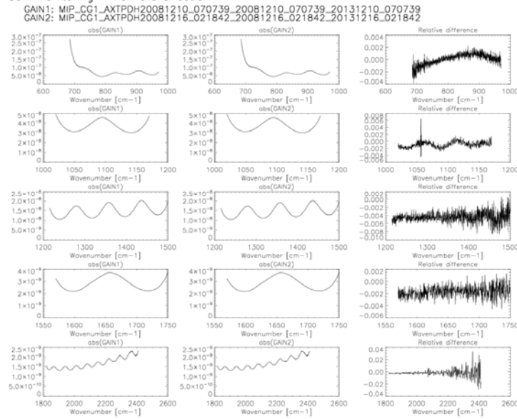
Figure 14 The same as Figure 12 but for a gain measured on 16 Dec 2008.
