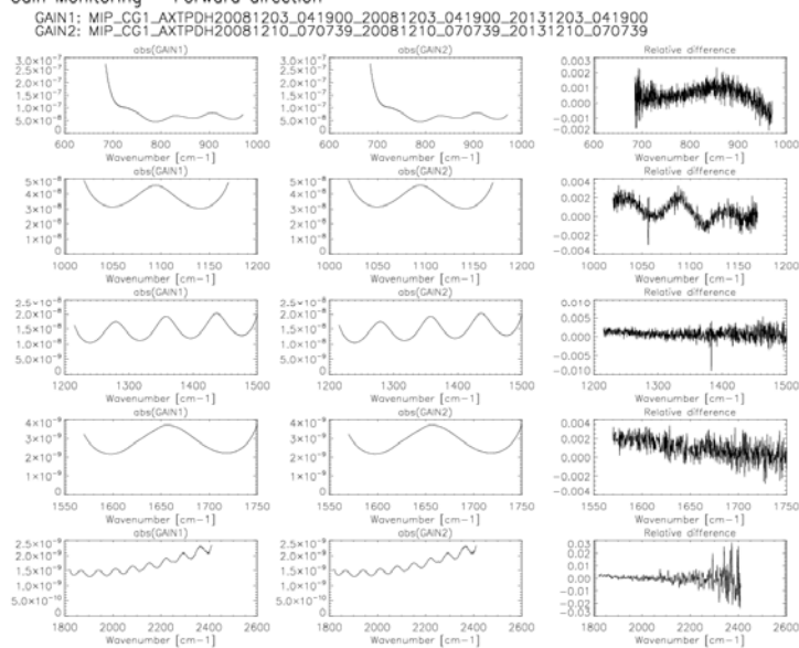
Figure 13 The same as Figure 12 but for a gain measured on 10 Dec 2008.
