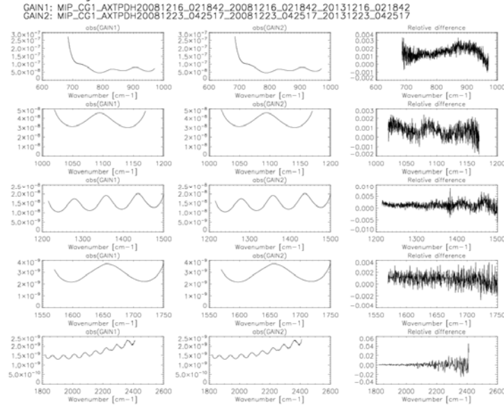
Figure 15 The same as Figure 12 but for a gain measured on 23 Dec 2008.
