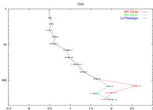
Figure 40 Temperature N2O and CH4 profiles as a function of pressure retrieved with IPF 4.62 and 4.61 compared to the prototype for seq. 16 of orbit 2975. The 4.61 profile is the reference, validated by a IMK balloon flight.
