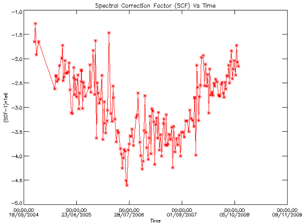
Figure 11 MIPAS Spectral Calibration Factor (SCF) since August 2004.
