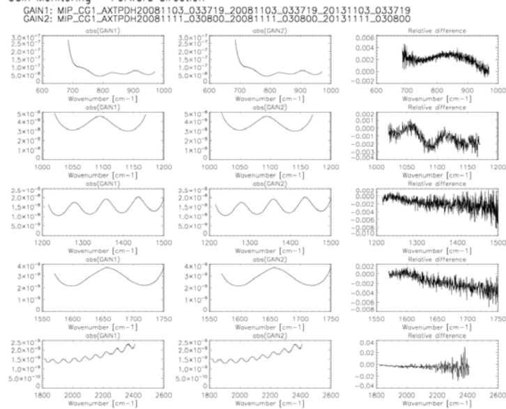
Figure 13 The same as Figure 12 but for a gain measured on 12 Oct 2008.
