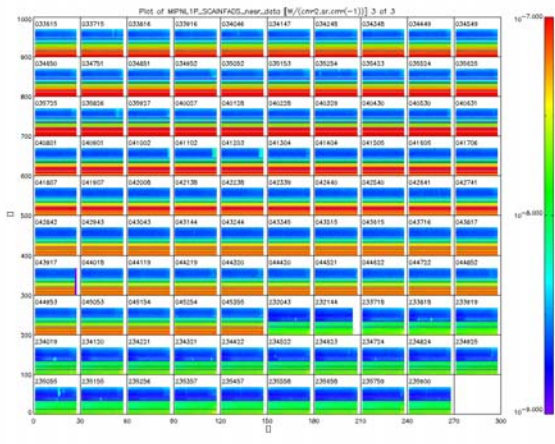
Figure 28 NESR level for different scan during 23 June 2005, each square is a scan made of 27 sweeps in nominal mode, the red lines show the anomaly of excessive high NESR, the anomaly stops when the correct ADF start to be used by the processor.
