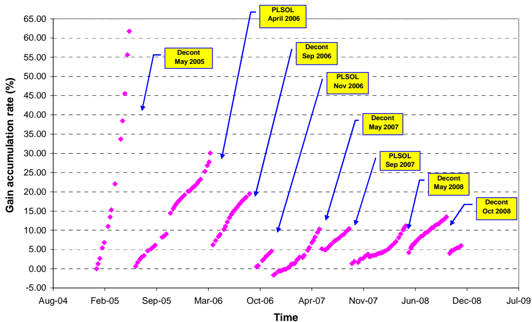
Figure 17 Gain accumulation increase since January 2005.
