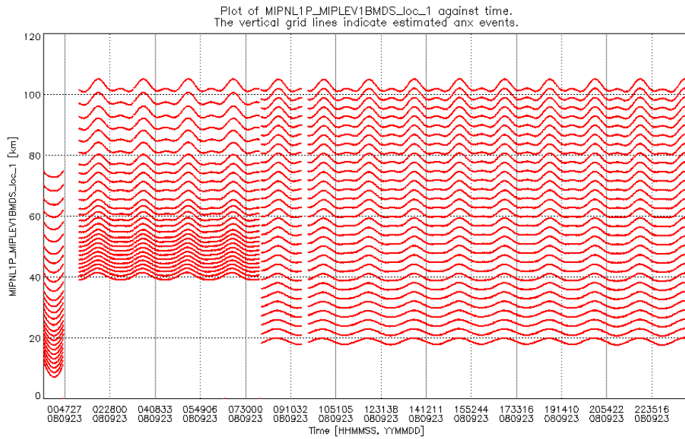
Figure 39 Tangent altitude measured by MIPAS during 23 September 2008.
