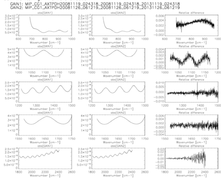
Figure 15 The same as Figure 12 but for a gain measured on 26 Oct 2008.
