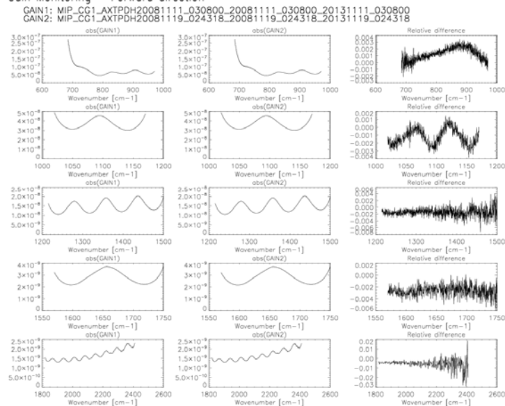
Figure 14 The same as Figure 12 but for a gain measured on 19 Oct 2008.
