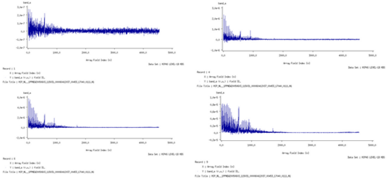
Figure 32 Example of correctly calibrated spectra obtained with the new ADFs.
