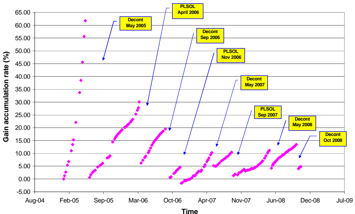
Figure 17 Gain accumulation increase since January 2005.
