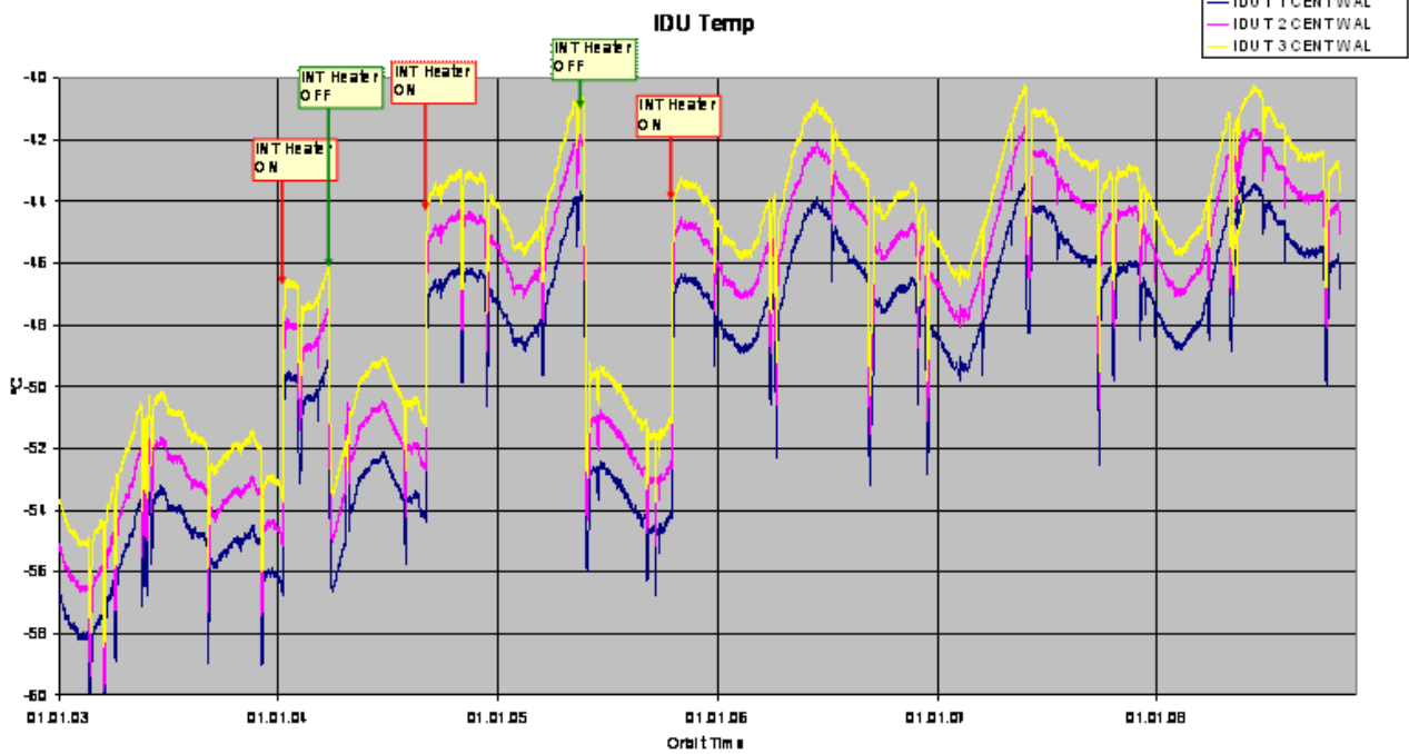
Figure 4 - IDU temperatures as a function of time since November 2002 (courtesy of Astrium).
