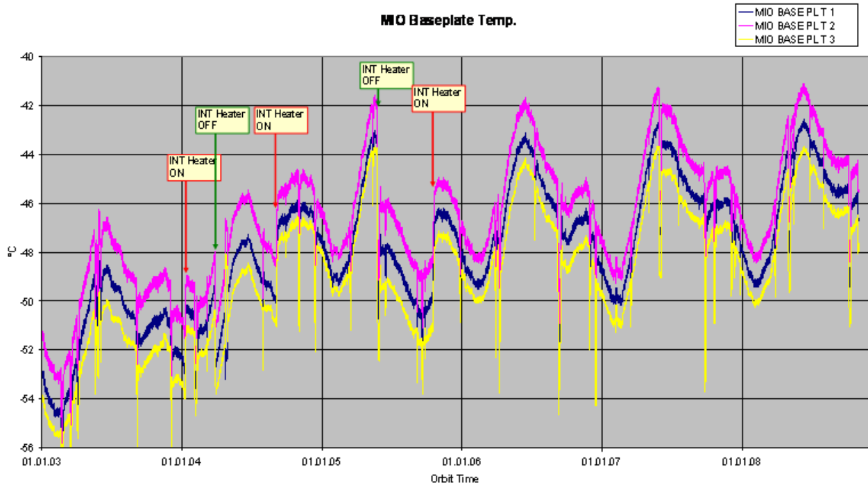
Figure 5 - MIO base plate temperatures as a function of time since November 2002 (courtesy of Astrium).
