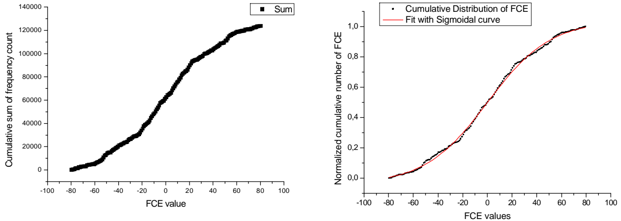
Figure 20 Cumulative distributions function of the FCE for one month of data. The fit with a sigmoid curve is reported on the right side.
