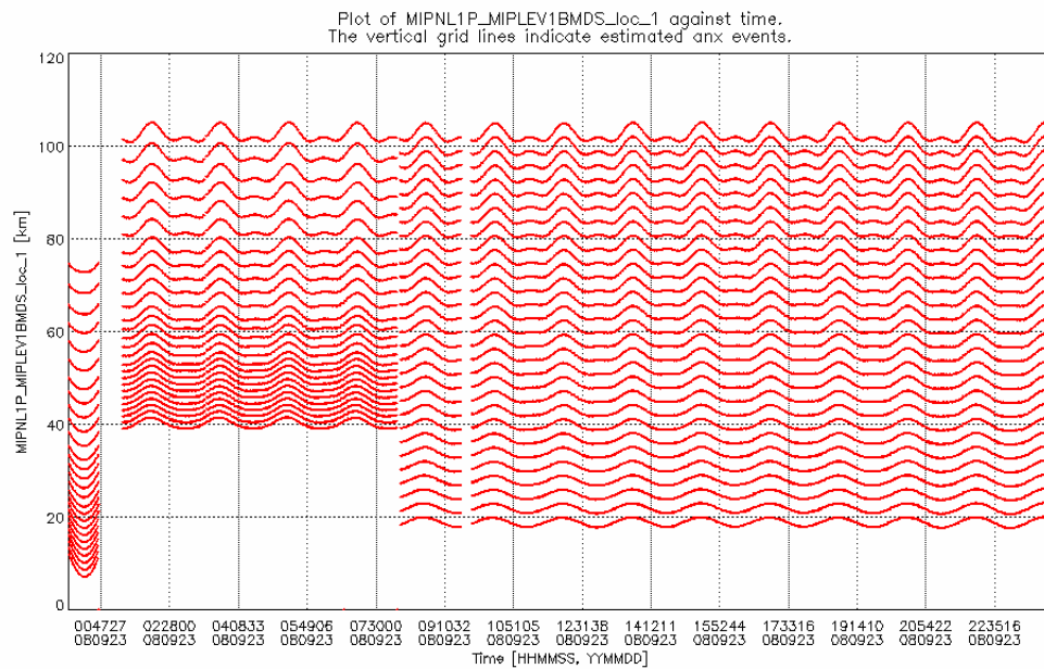
Figure 40 Tangent altitude measured by MIPAS during 23 September 2008.
