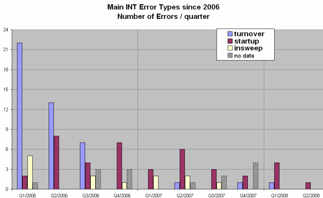
Figure 7 Main INT error types since 2006 (courtesy of Astrium).
