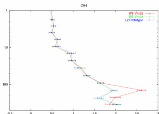
Figure 41 Temperature N 2 O and CH 4 profiles as a function of pressure retrieved with IPF 4.62 and 4.61 compared to the prototype for seq. 16 of orbit 2975. The 4.61 profile is the reference, validated by a IMK balloon flight.
