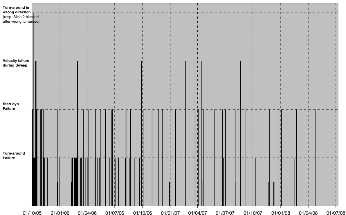
Figure 7 INT anomalies since Oct 2005 (courtesy of Astrium).
