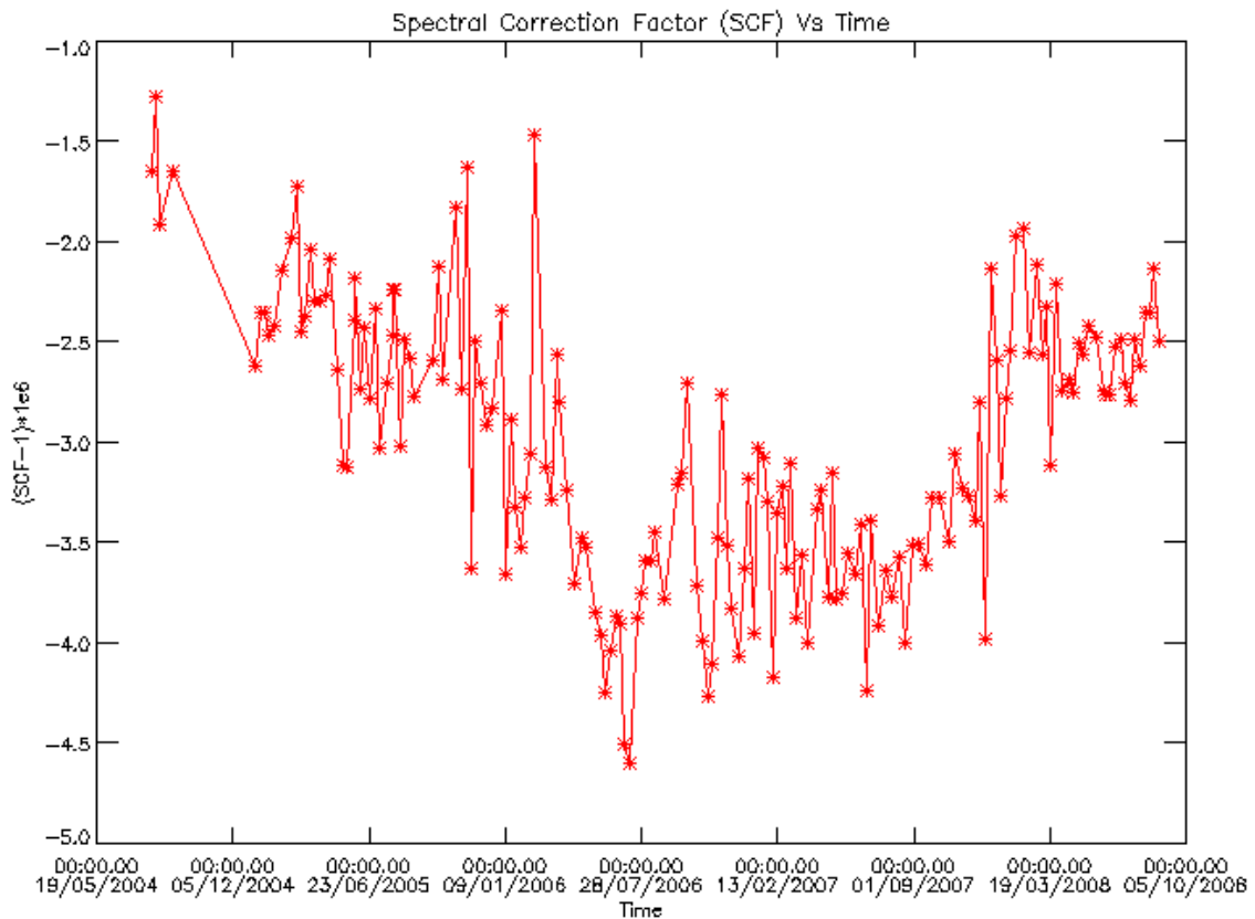
Figure 11 MIPAS Spectral Calibration Factor (SCF) since August 2004.
