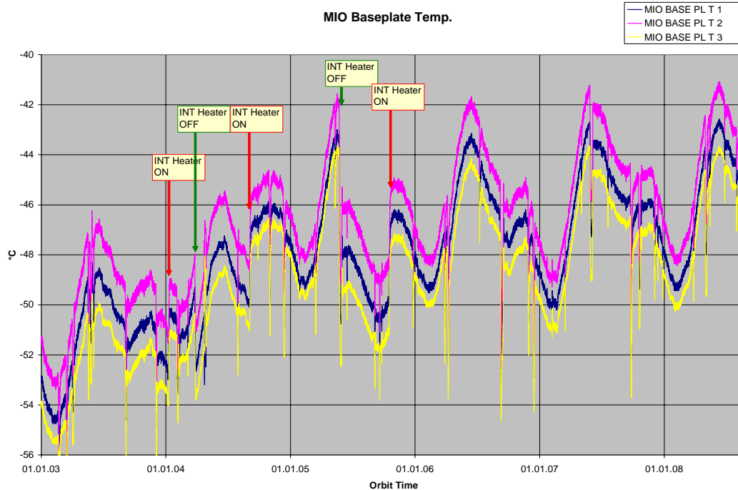
Figure 5 - MIO base plate temperatures as a function of time since November 2002 (courtesy of Astrium).
