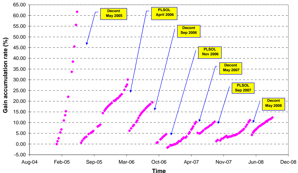
Figure 17 Gain accumulation increase since January 2005.
