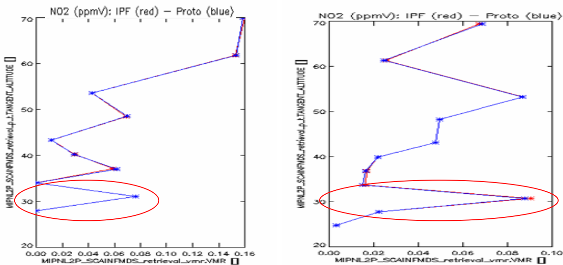
Figure 40 NO2 profiles obtained with the IPF and prototype for two particular scan of 6 June 2003 in Antarctic winter condition, highlighted in red are the region around 30 km with sudden increase of NO2 value, which has no physical meaning. Note the degraded profile shape, namely the zigzag and the zero value.
