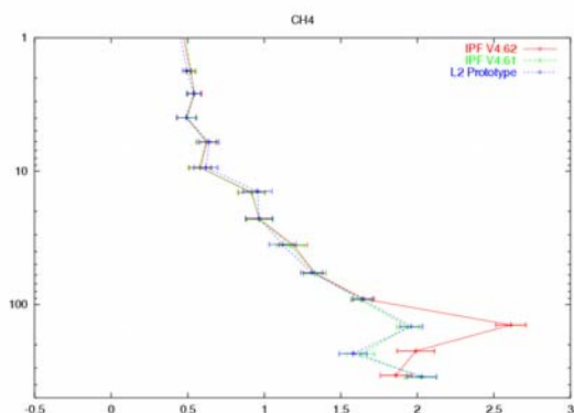
Figure 39 Temperature N 2 O and CH 4 profiles as a function of pressure retrieved with IPF 4.62 and 4.61 compared to the prototype for seq. 16 of orbit 2975. The 4.61 profile is the reference, validated by a IMK balloon flight.
