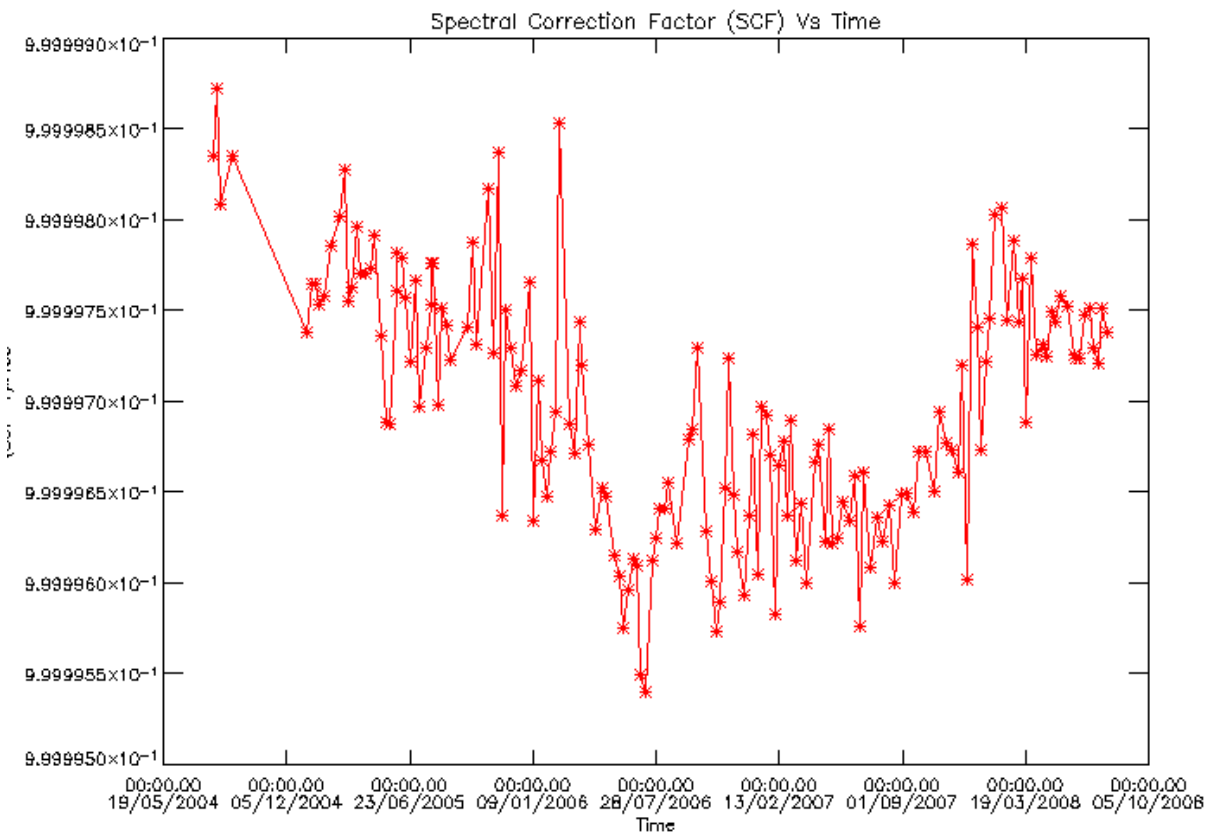
Figure 11 MIPAS Spectral Calibration Factor (SCF) since August 2004.
