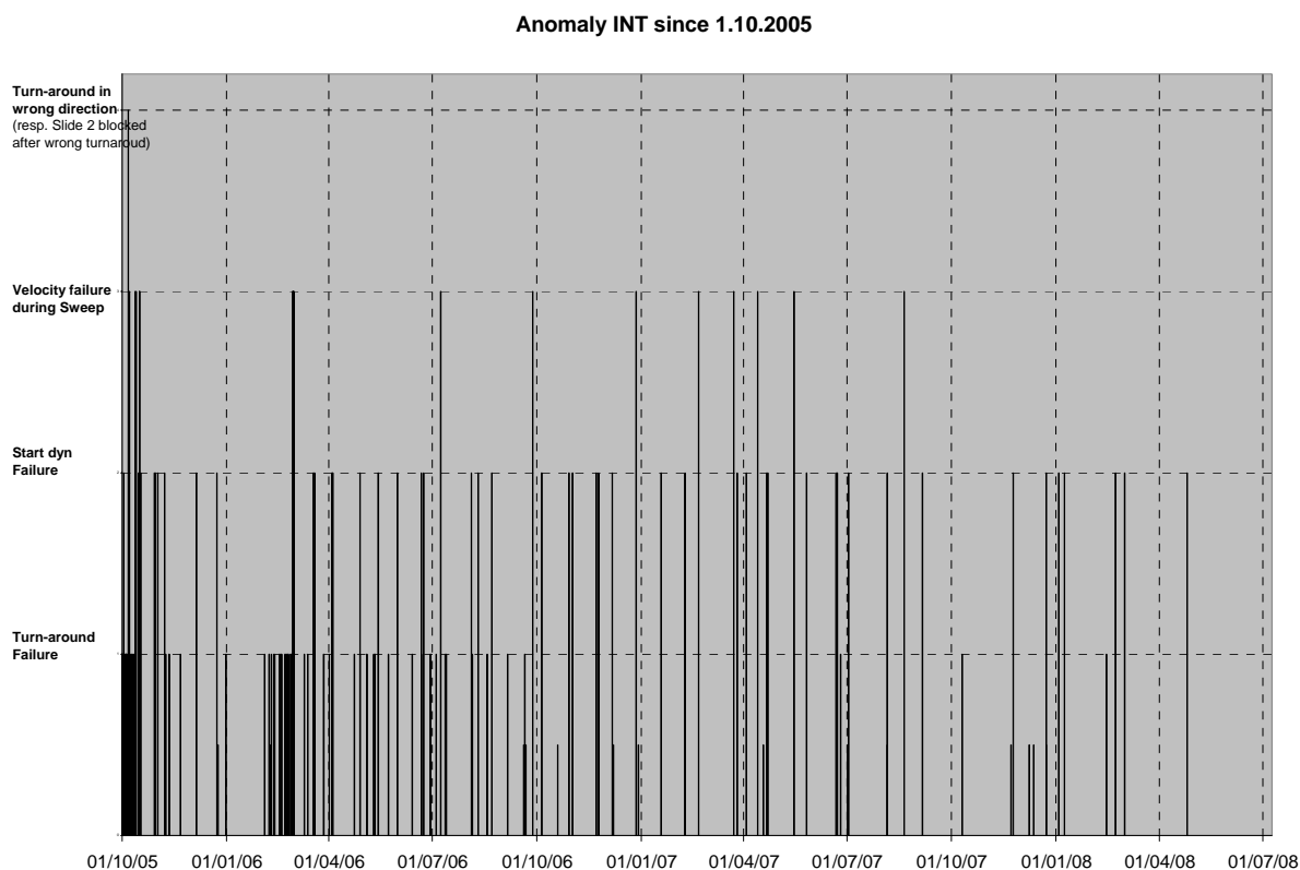
Figure 7 INT anomalies since Oct 2005 (courtesy of Astrium).
