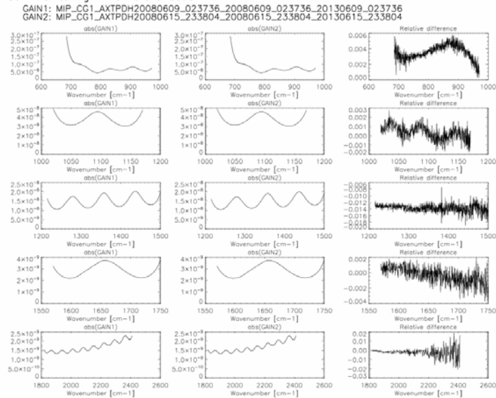
Figure 14 The same as Figure 12 but for a gain measured on 15 June 2008.
