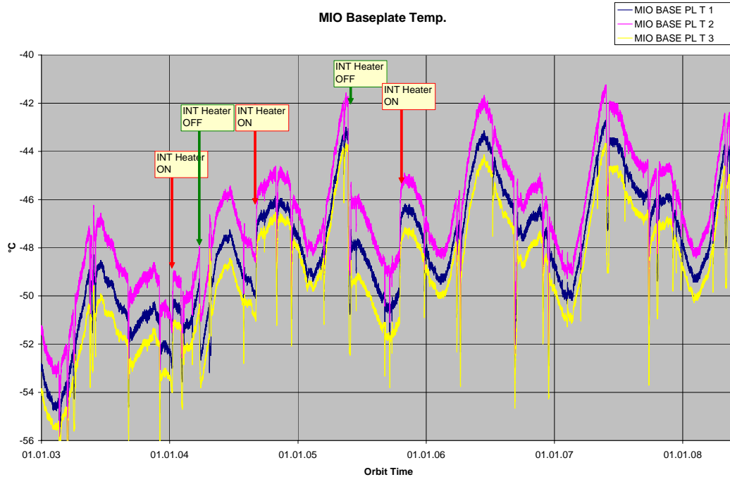
Figure 5 - MIO base plate temperatures as a function of time since November 2002 (courtesy of Astrium).
