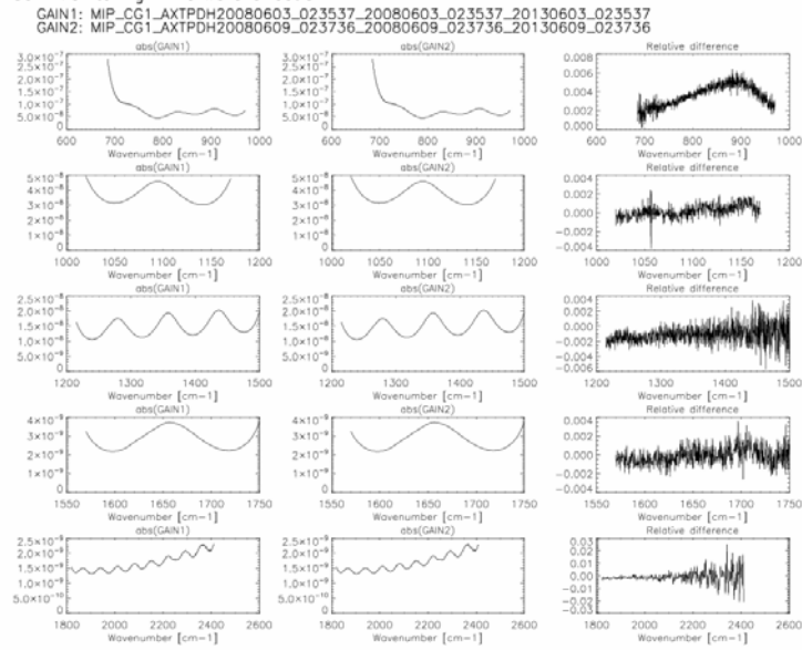
Figure 13 The same as Figure 12 but for a gain measured on 8 June 2008.
