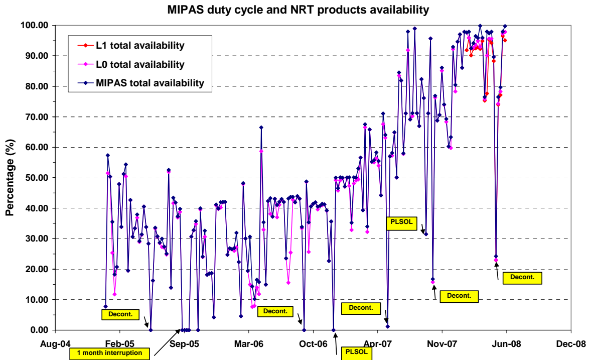
Figure 2 – MIPAS L0 NRT long term statistics since Jan 2005.
