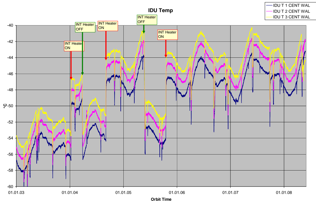
Figure 5 - IDU temperatures as a function of time since November 2002 (courtesy of Astrium).
