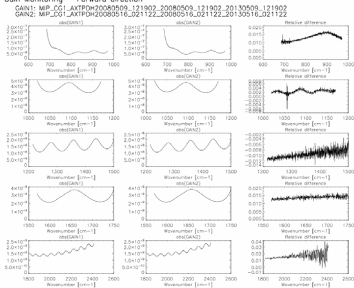
Figure 14 The same as Figure 13 but for a gain measured on 15 May 2008.
