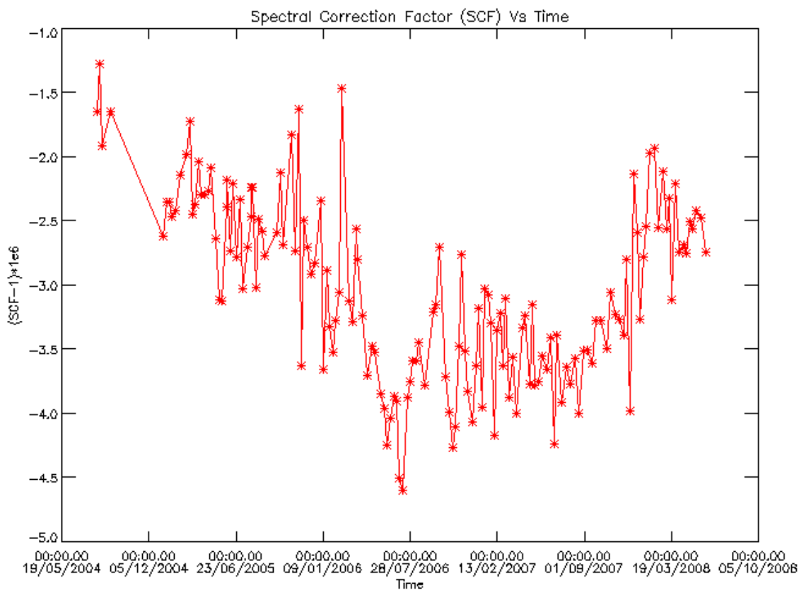
Figure 12 MIPAS Spectral Calibration Factor (SCF) since August 2004.
