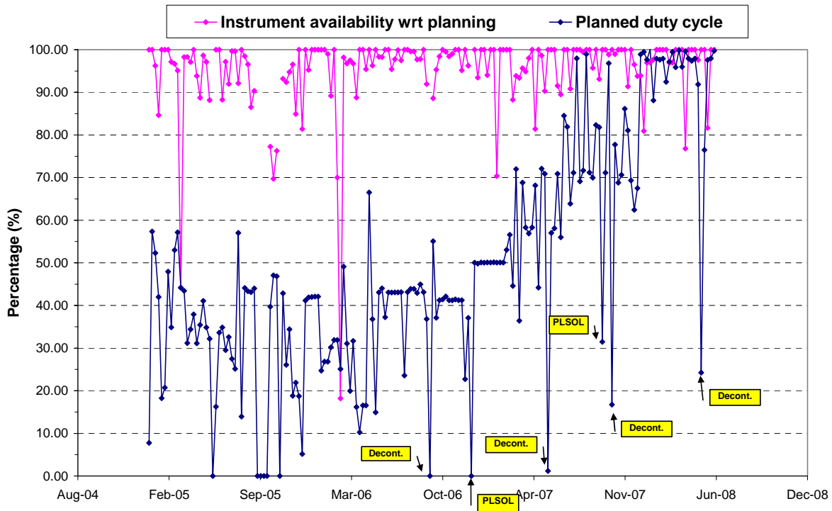
Figure 3 – MIPAS instrument availability wrt planning and planned duty cycle.
