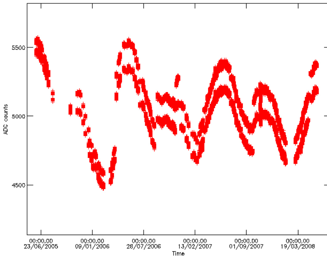
Figure 10 ADC max counts in channel A1 during DS measurements since June 2005.
