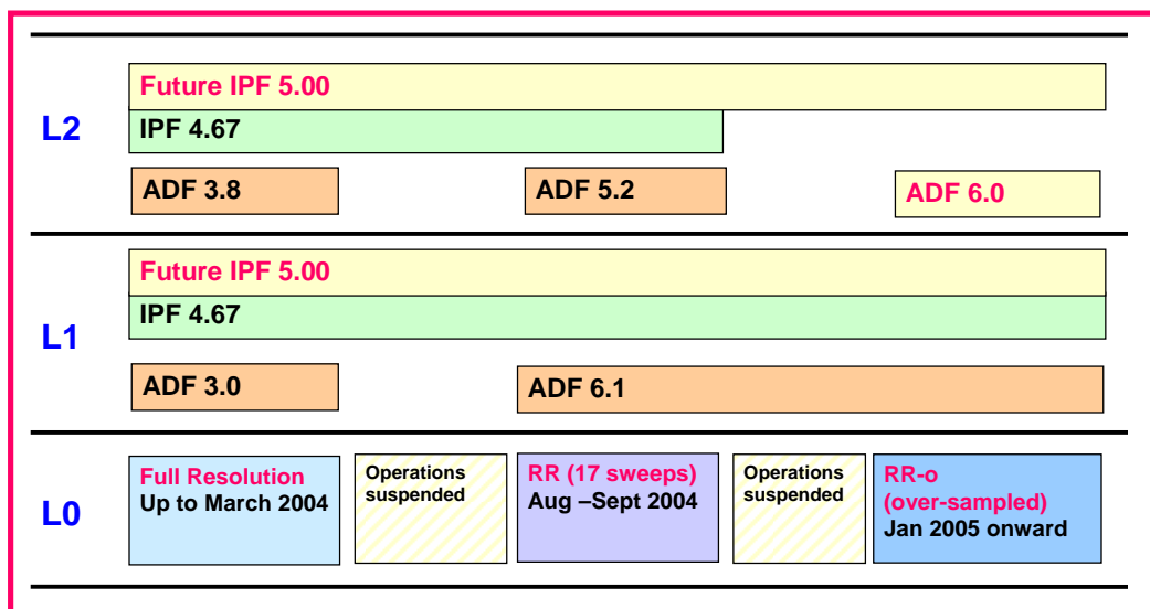
Figure 11 IPF and ADF validity for processing level 1 and level 2 products. IPF 4.62 – 4.61 were used for re-processing of FR mission, while the IPF 4.67 is now operational at D-PAC for OFL processing of RR mission. IPF 5.00 is the future IPF that will be used for OFL processing and for reprocessing of the whole mission. IPF 5.0 will be the only one able to process RR over-sampled measurements up to L2.
