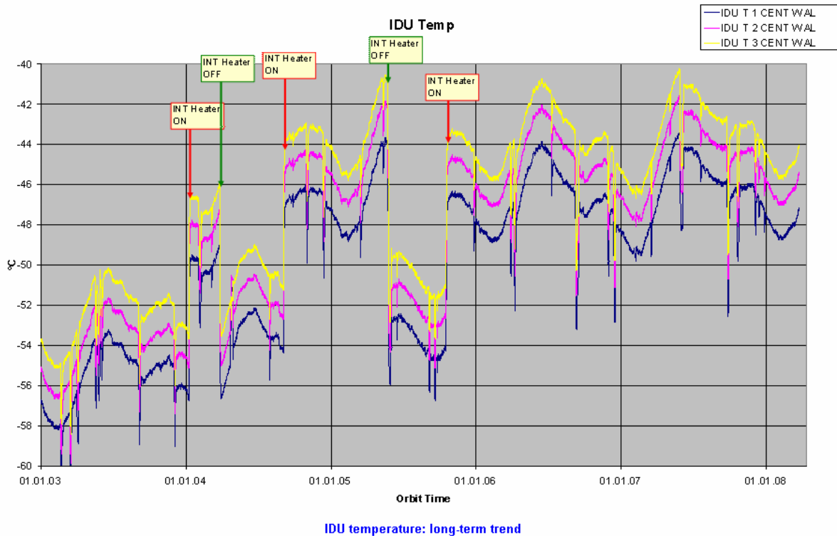
Figure 4 IDU temperatures as a function of time since November 2002 (courtesy of Astrium).
