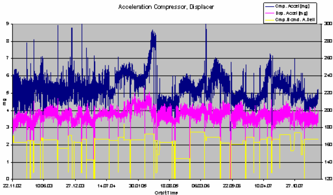
Cooler (FCA) Compressor / Displacer Acceleration
