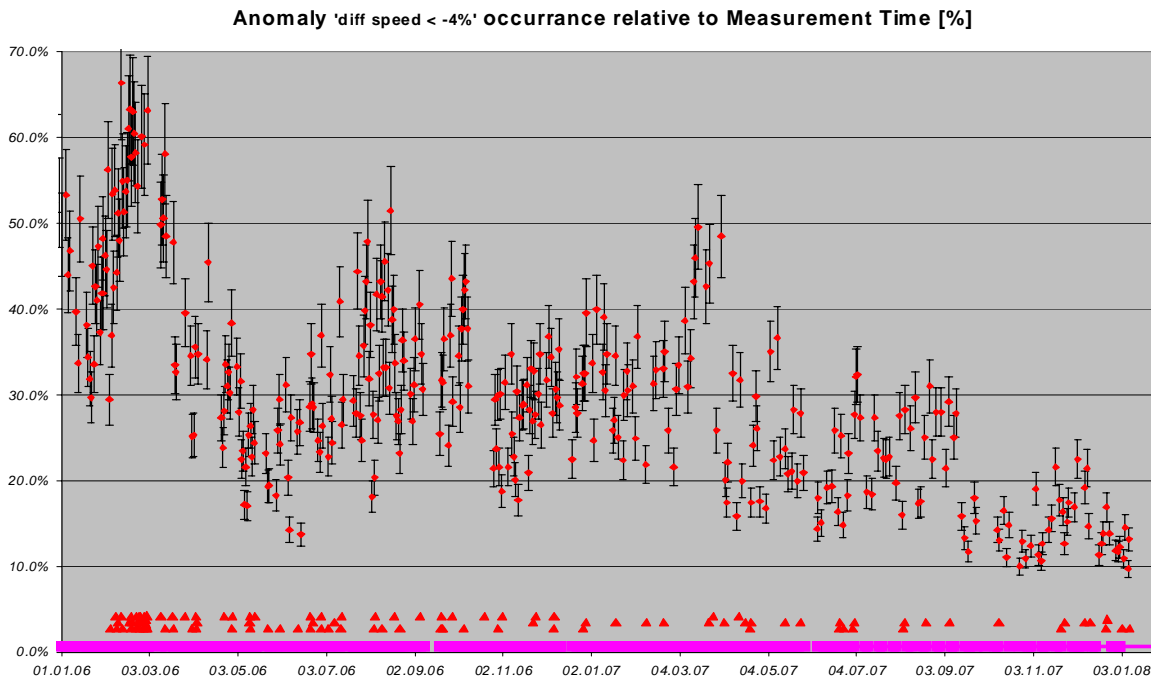
Figure 7 Occurrence of -4% differential speed error relative to measurement time since May 2005 (courtesy of Astrium).
