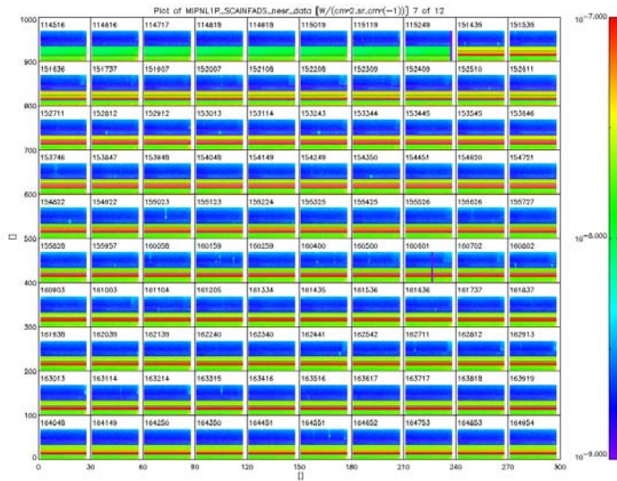
Figure 35 NESR value during 18 th Apr 2007. The red stripes show the anomaly consisting in excessive NESR values in the band AB and B.
