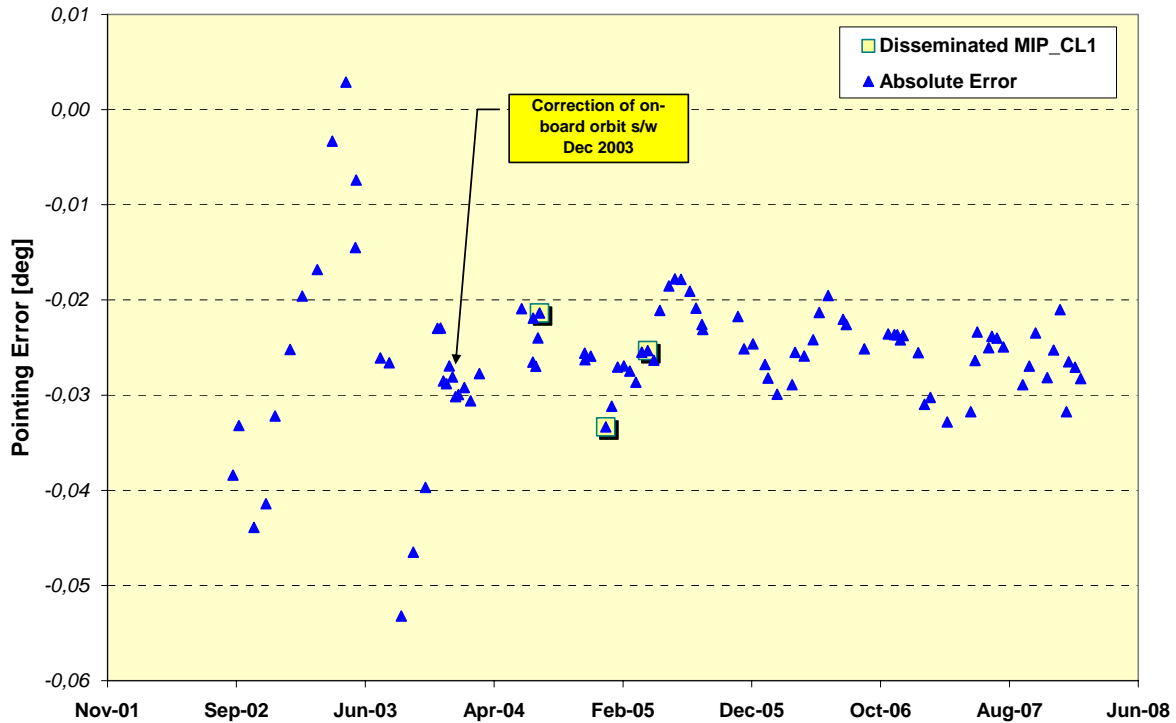
Figure 20 MIPAS long-term pointing error as a function of time since September 2002.
