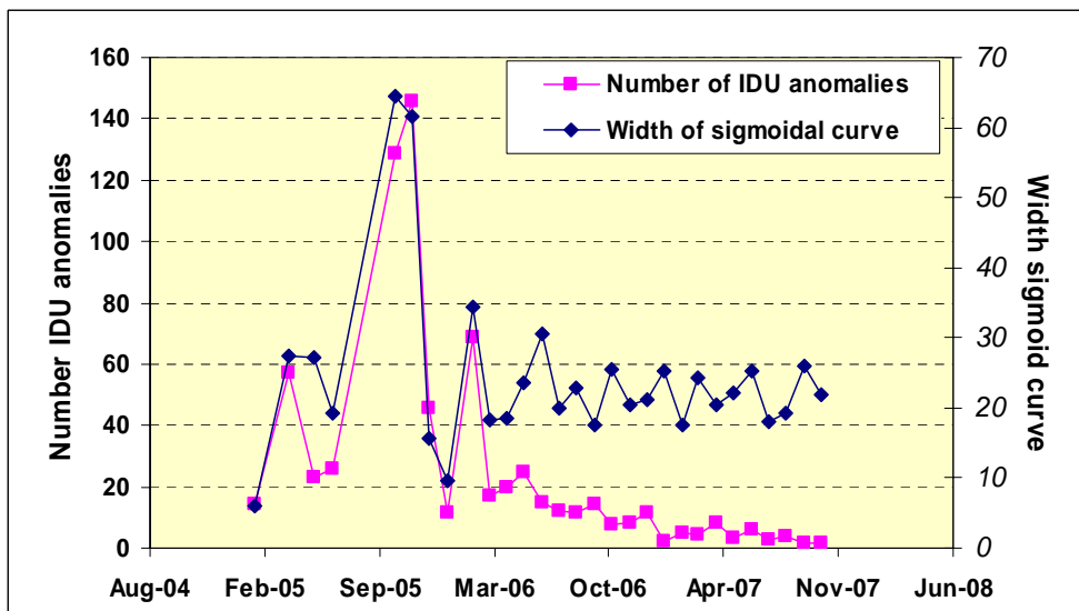
Figure 23 Width of the sigmoid curve (used to fit the FCE statistic distribution) plotted on a long term basis together with the number of IDU errors.
