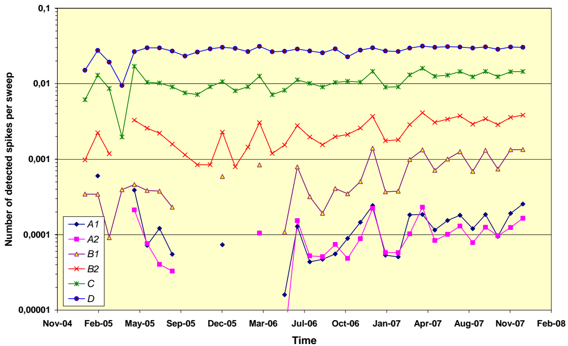
Figure 25 MIPAS long-term monitoring of spikes: number of detected spikes per sweep.
