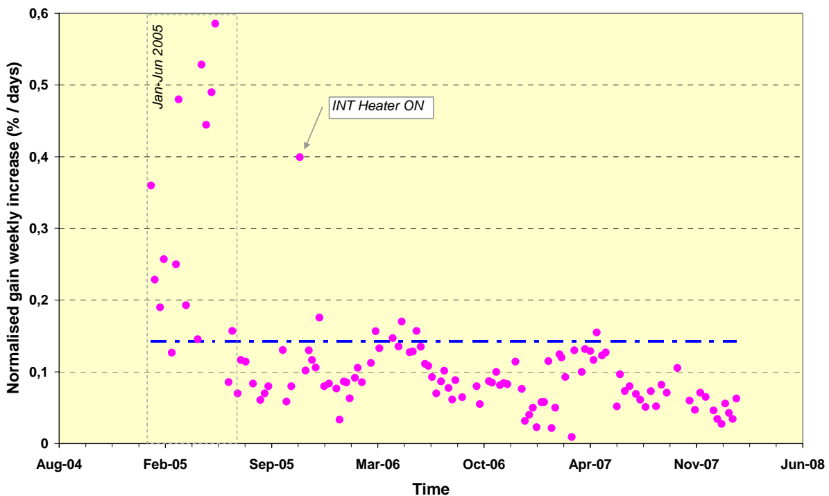
Figure 18 Gain maximum increase normalized to the time difference between consecutive disseminated gains since January 2005.
