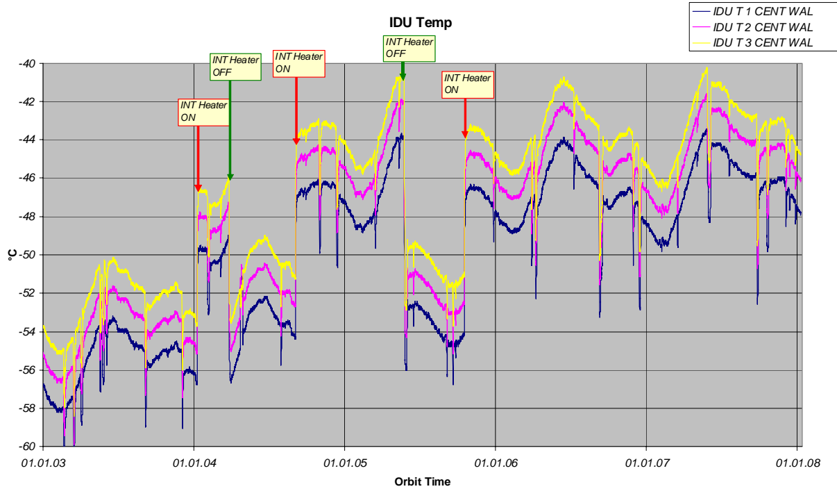
Figure 4 MIO base plate temperatures as a function of time since November 2002 (courtesy of Astrium).
