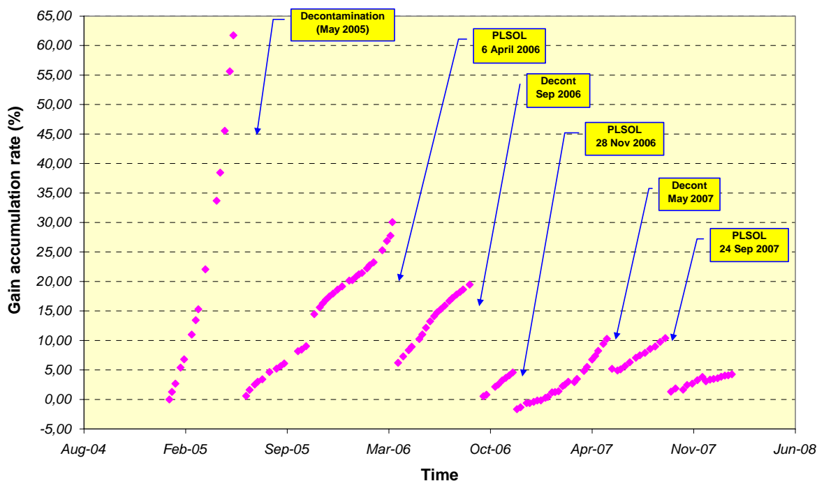
Figure 19 Gain accumulation increase since January 2005.
