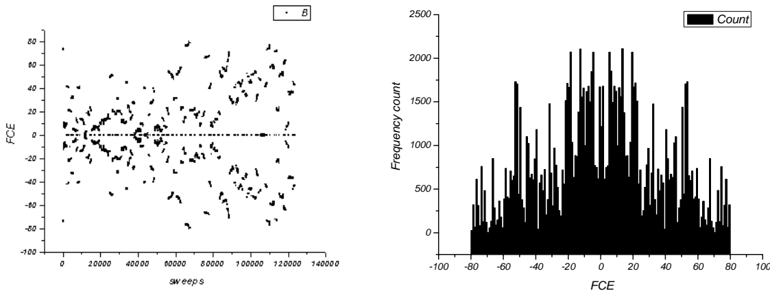
Figure 21 FCE values for one month of measurements and corresponding frequency distribution,
