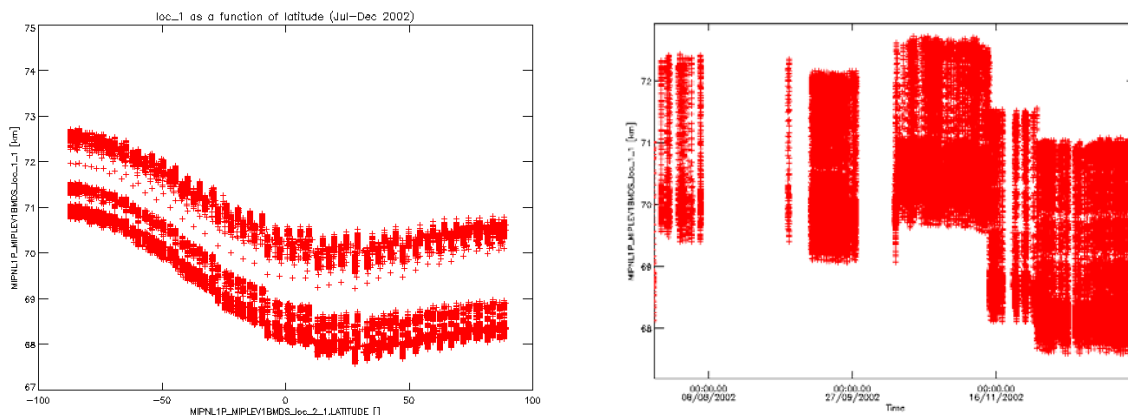
Figure 41 MIPAS engineering tangent altitude as written in the L1b files (loc_1 field) as a function of latitude and time.
