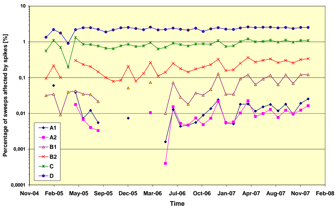
Figure 24 MIPAS long-term monitoring of spikes: percentage of spike-affected sweeps.
