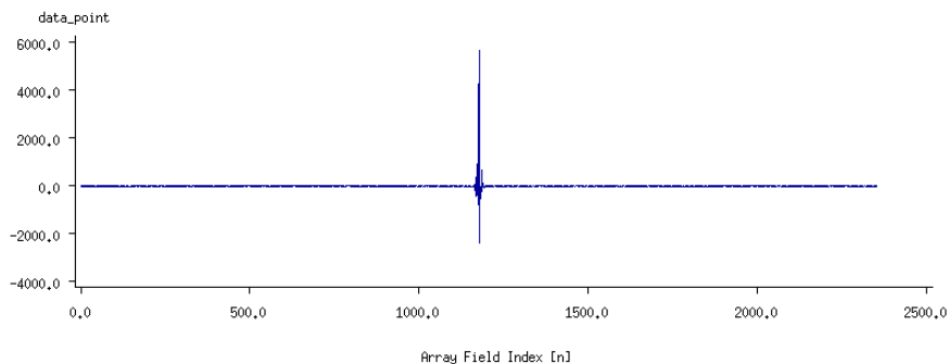
Figure 33 IGM recorded in the deep space measurement and stored in the new correct ADF.
