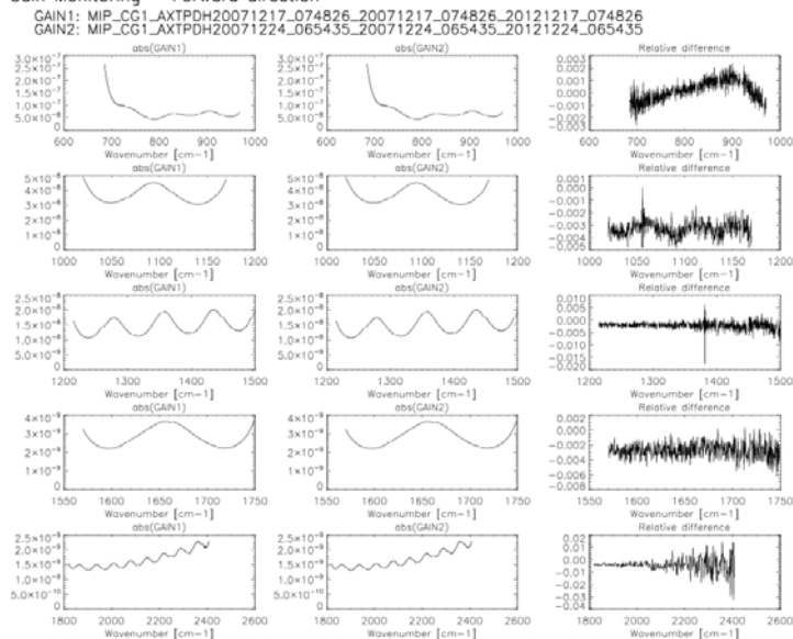
Figure 17 The same as Figure 14 but for a gain measured on 23 Dec 2007.
