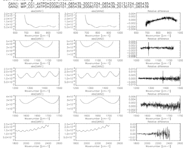
Figure 18 The same as Figure 14 but for a gain measured on 31 Dec 2007.
