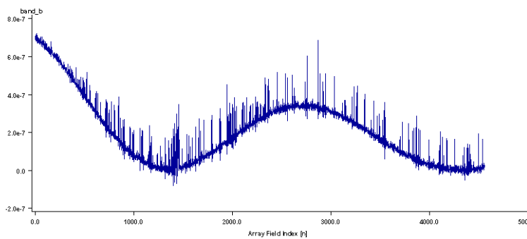
Figure 37 Band B spectrum for orbit 26839 measured on 19 th April 2007.
