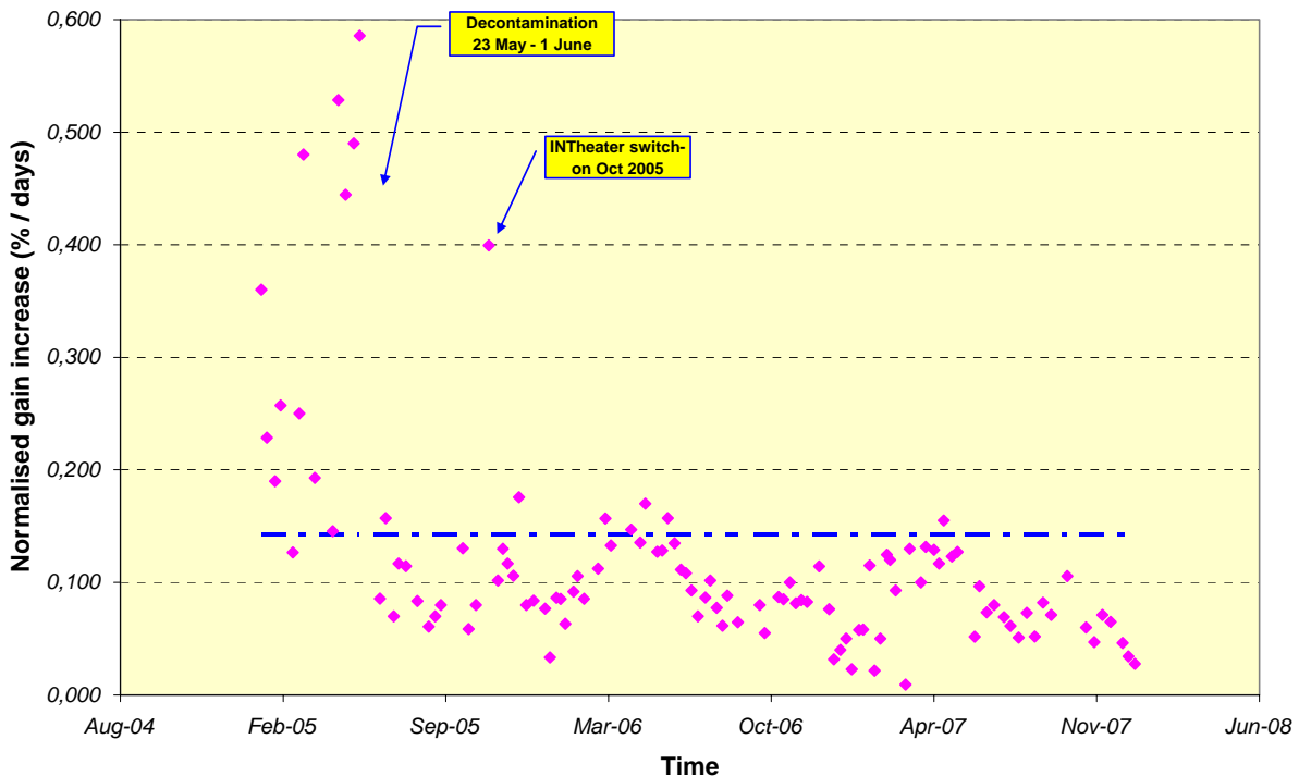
Figure 19 Gain maximum increase normalized to the time difference between consecutive disseminated gains since January 2005.
