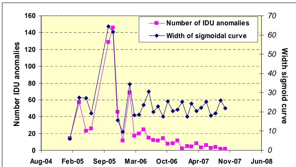
Figure 24 Width of the sigmoid curve (used to fit the FCE statistic distribution) plotted on a long term basis together with the number of IDU errors.
