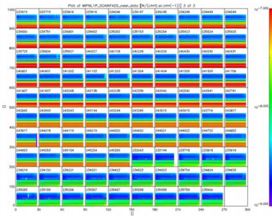
Figure 31 NESR level for different scan during 23 June 2005, each square is a scan made of 27 sweeps in nominal mode, the red lines show the anomaly of excessive high NESR, the anomaly stops when the correct ADF start to be used by the processor.
