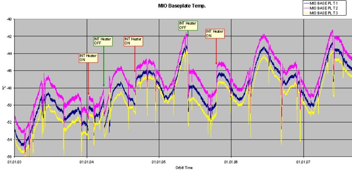
Figure 3 MIO base plate temperatures as a function of time since November 2002 (courtesy of Astrium).
