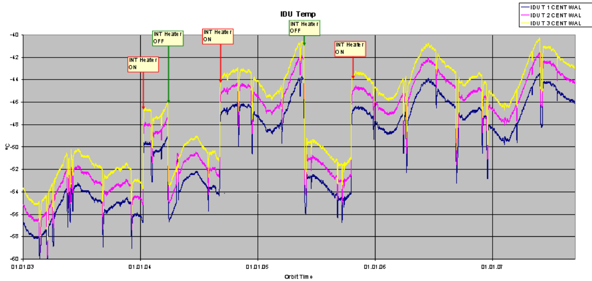
Figure 2 IDU temperatures as a function of time since November 2002 (courtesy of Astrium).
