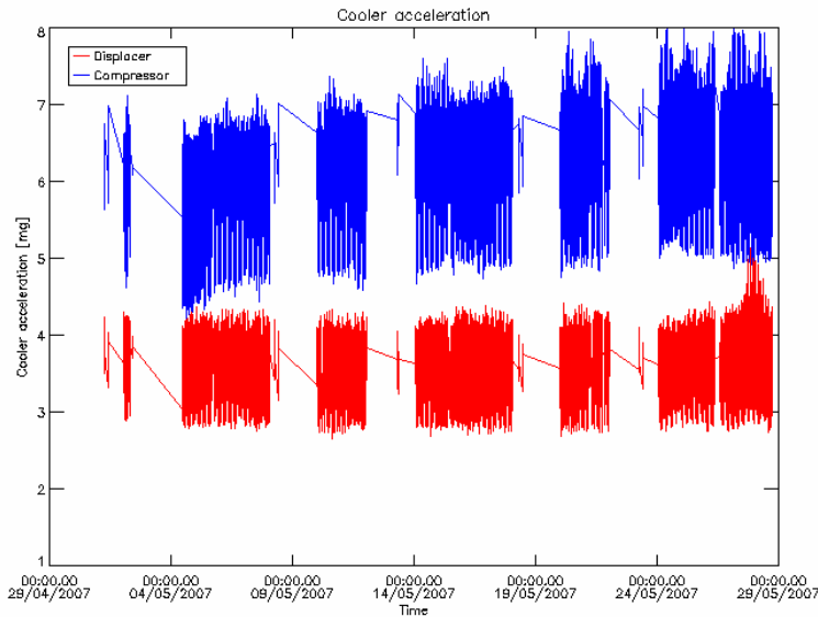
Figure 8 May 2007: Cooler Displacer and Compressor vibration level.
