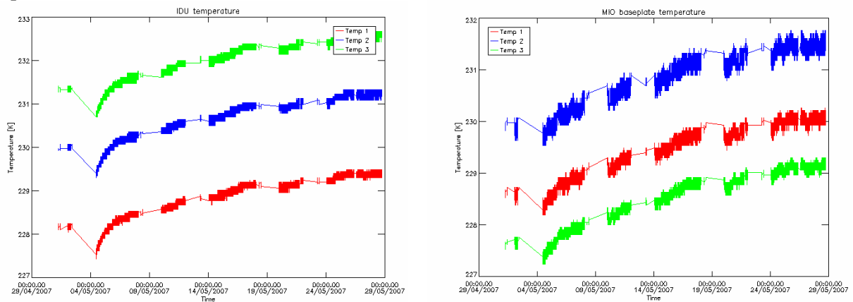
Figure 3 IDU and MIO Base-Plate temperature during reporting period: May 2007.
