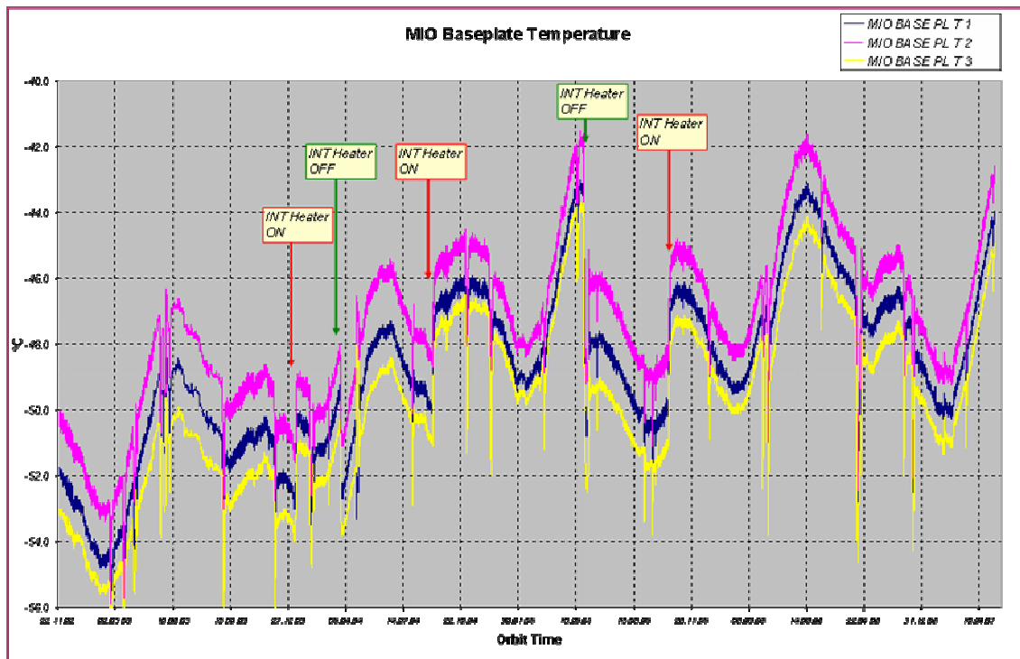
Figure 2 MIO base plate temperatures as a function of time: November 2002 – May 2007 (courtesy of Astrium).
