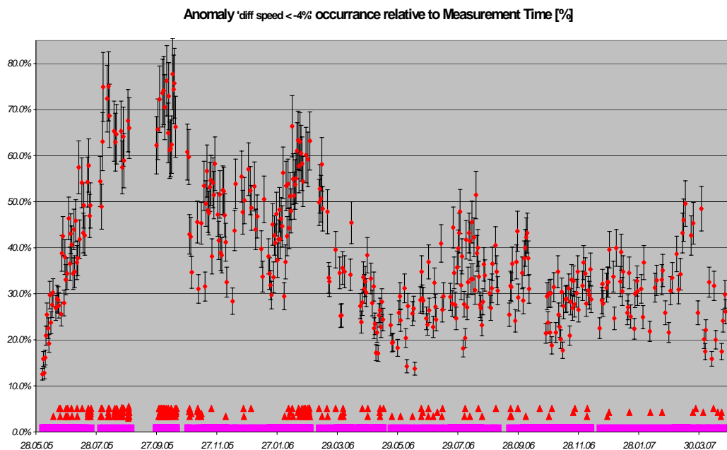
Figure 5 Occurrence of -4% differential speed error relative to measurement time since May 2005 (courtesy of Astrium).
