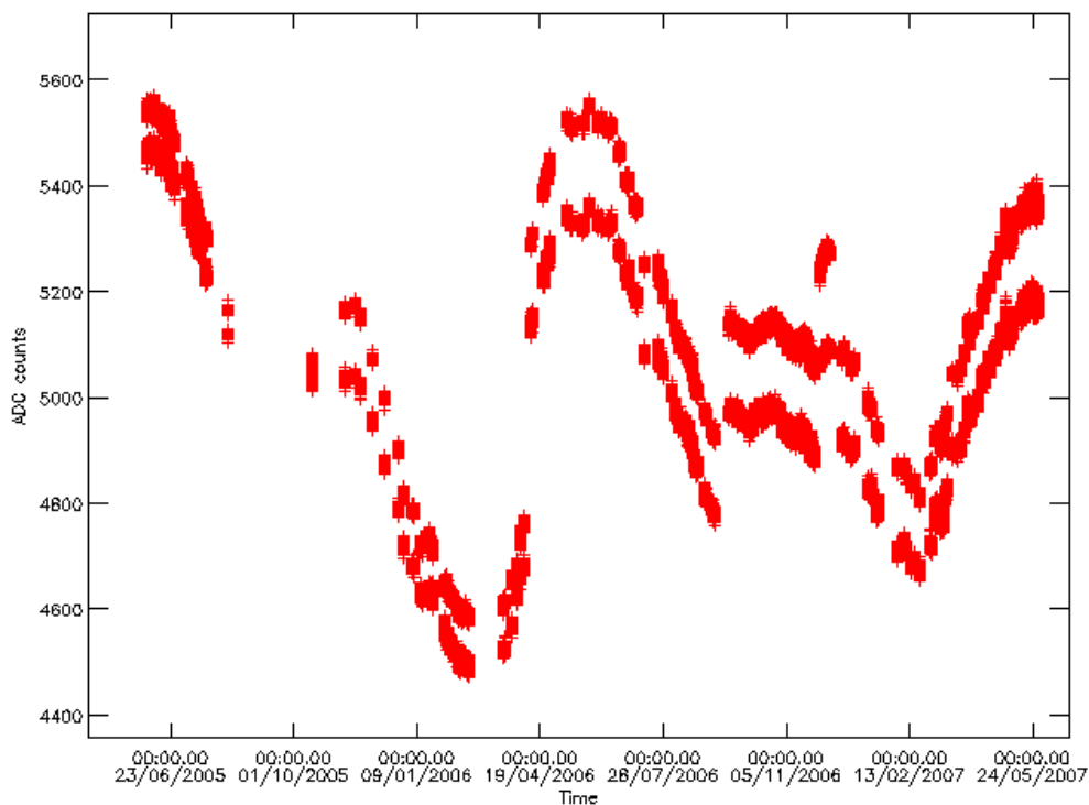
Figure 9 ADC max counts in channel A1 during DS measurements from June 2005 to May 2007.
