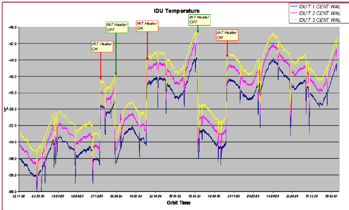
Figure 1 IDU temperatures as a function of time: November 2002 – May 2007 (courtesy of Astrium).
