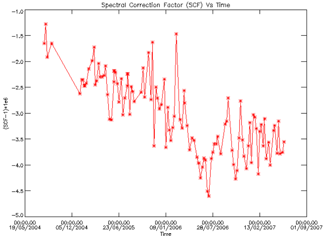
Figure 11 MIPAS Spectral Calibration Factor (SCF) during RR ops updated to end of May 2007.
