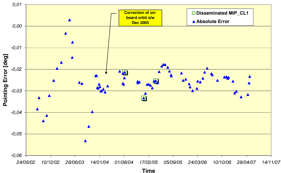
Figure 18 MIPAS long-term pointing error as a function of time: September 2002 – May 2007.
