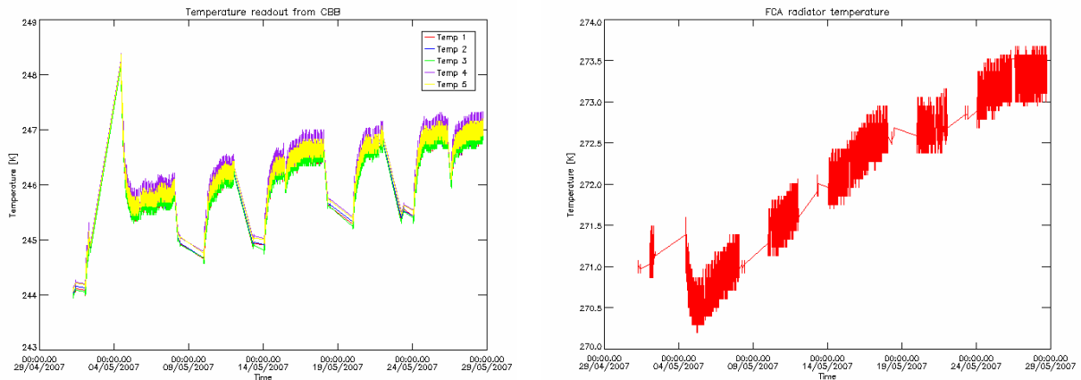
Figure 4 CBB and FCA radiator temperature during reporting period: May 2007.
