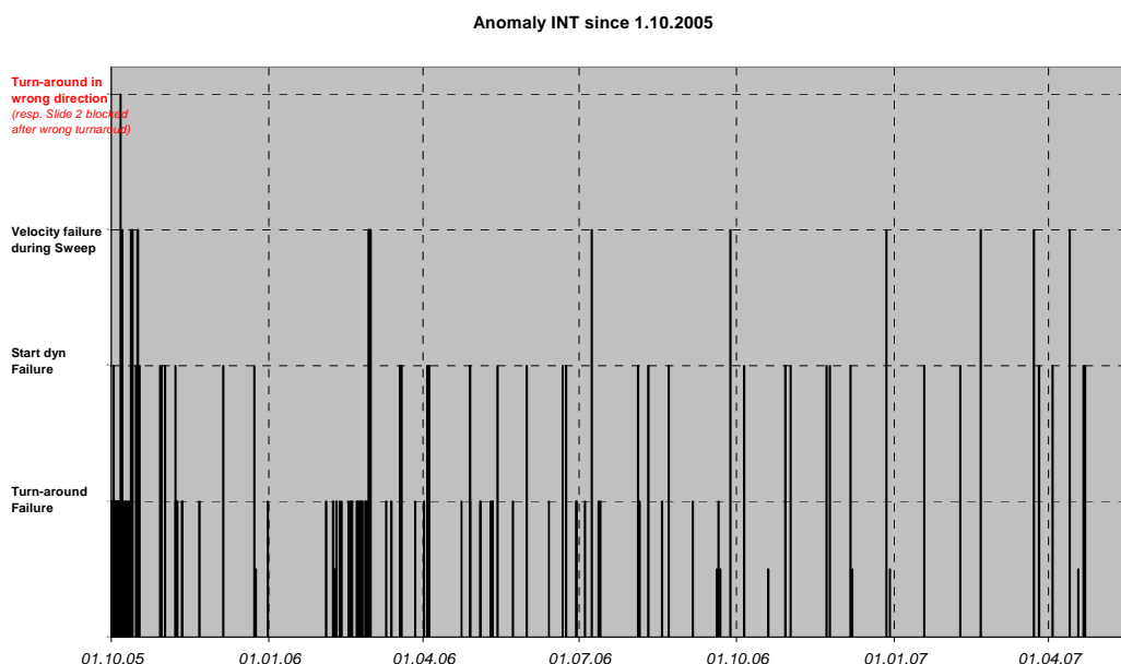
Figure 6 INT anomalies since Oct 2005 (courtesy of Astrium).
