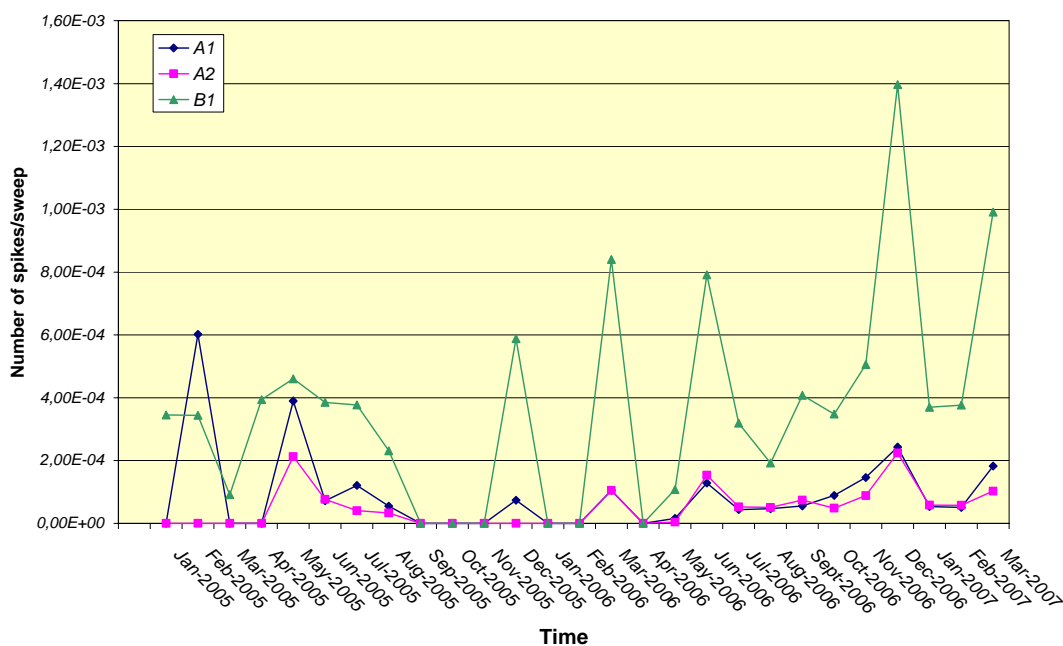
Figure 21 MIPAS long-term monitoring of number of detected/corrected spikes in the detectors A1, A2, B1. In the y-axis is reported the monthly average of detected spikes for each measured sweep.
