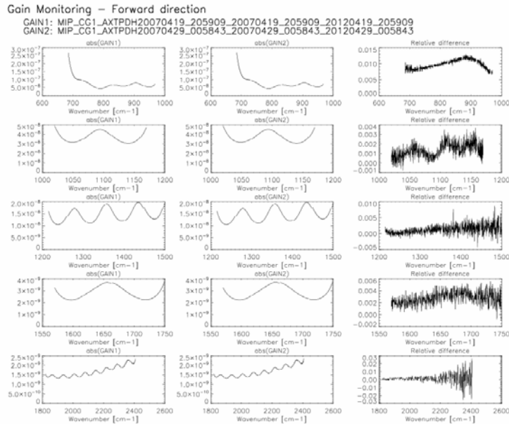
Figure 14 The same as Figure 12 but for a gain measured on 28 Apr 2007.
