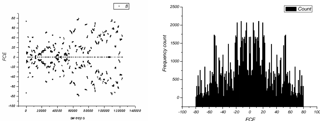
Figure 18 FCE values for one month of measurements and corresponding frequency distribution,
