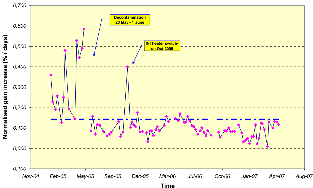
Figure 15 Gain maximum increase normalized to the time difference between consecutive disseminated gains since January 2005.
