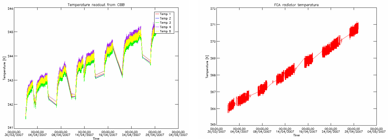
Figure 4 CBB and FCA radiator temperature during reporting period: April 2007.
