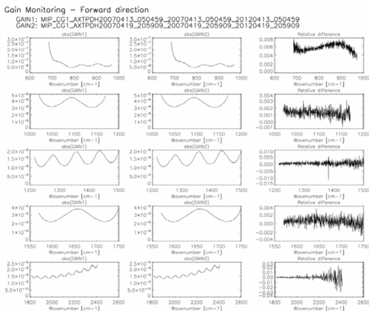
Figure 13 The same as Figure 12 but for a gain measured on 18 Apr 2007.
