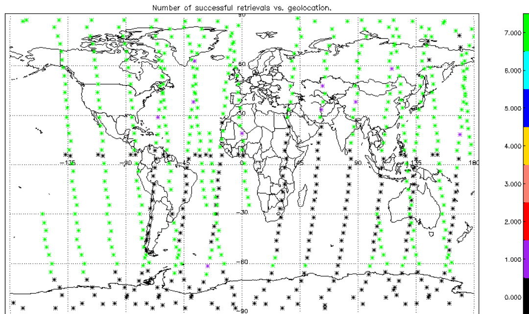
Figure 36 MIPAS number of successful retrieval for 25 July 2002. Note that 7 is the nominal value corresponding to the target species of the ESA MIPAS products. Zero value means that the retrieval fails already at the p-T stage.
