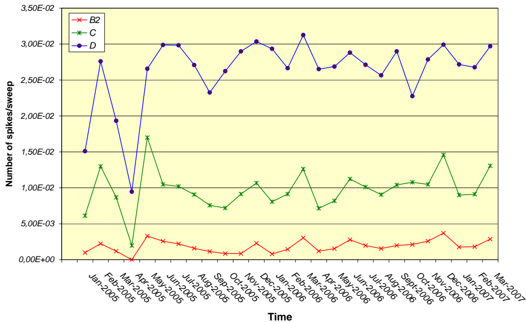
Figure 22 MIPAS long-term monitoring of number of detected/corrected spikes in the detectors B2, C and D. In the y-axis is reported the monthly average of detected spikes for each measured sweep.
