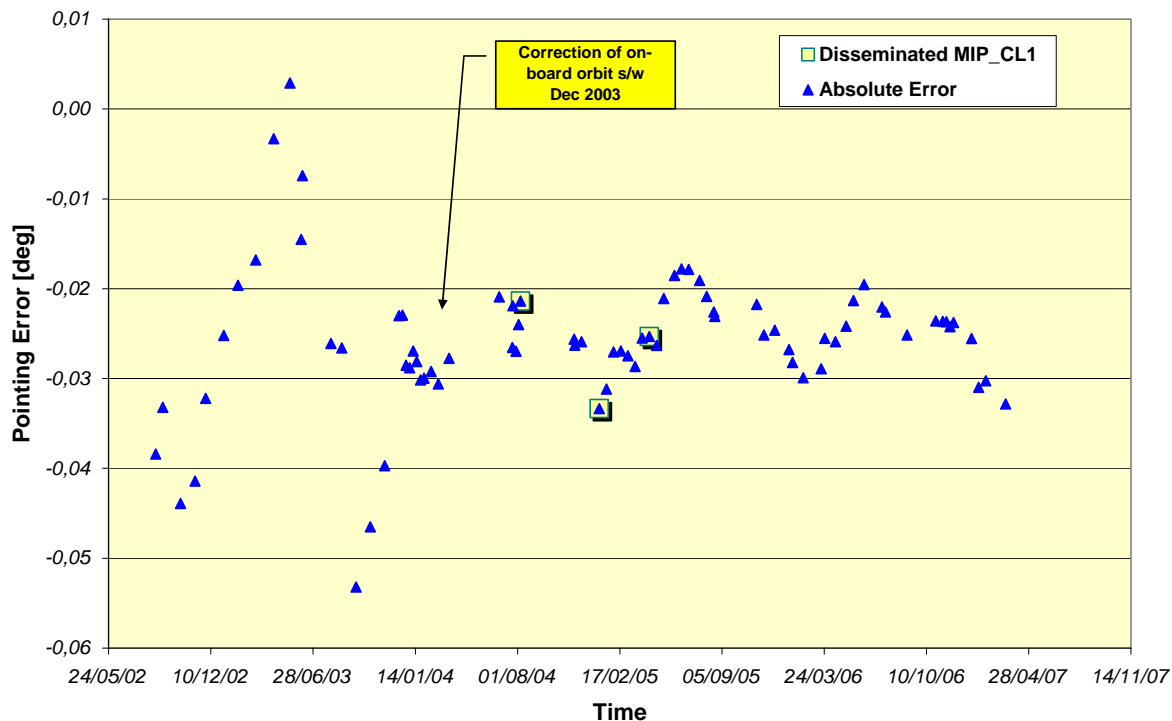
Figure 17 MIPAS long-term pointing error as a function of time: September 2002 – April 2007.
