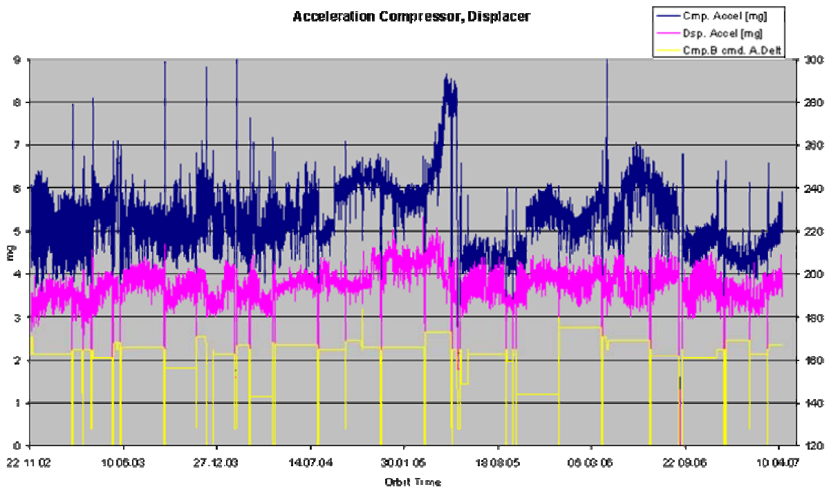
Figure 7 Cooler Displacer and Compressor vibration level, historical trend since 2002 (courtesy of Astrium).
