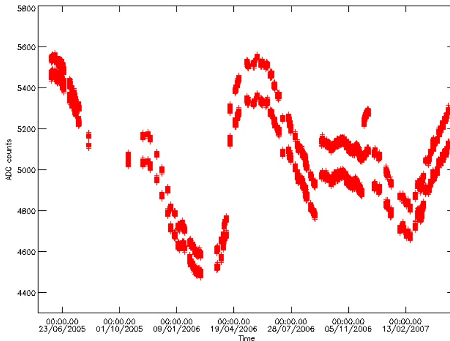
Figure 9 ADC max counts in channel A1 during DS measurements from June 2005 to April 2007.
