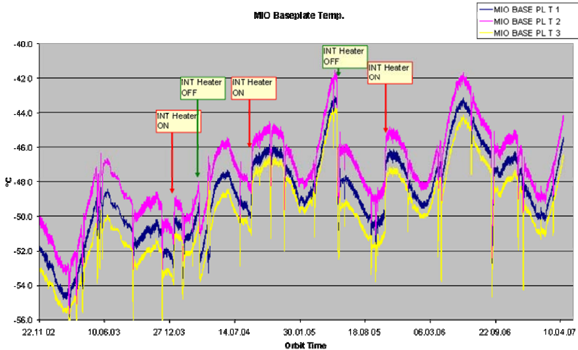
Figure 2 MIO base plate temperatures as a function of time: November 2002 – April 2007 (courtesy of Astrium).
