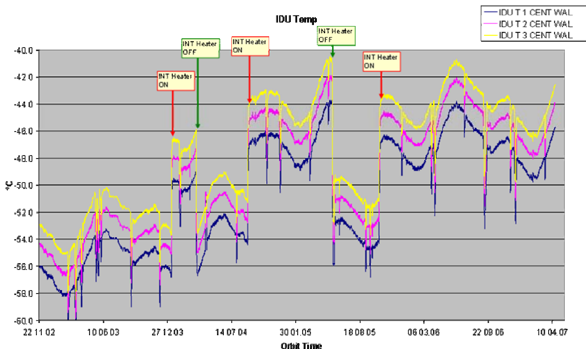
Figure 1 IDU temperatures as a function of time: November 2002 – April 2007 (courtesy of Astrium).
