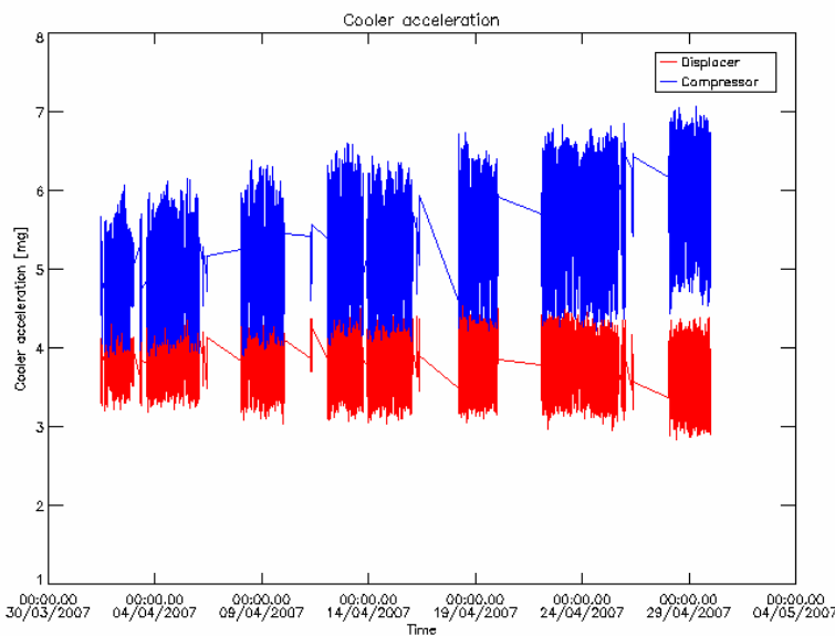
Figure 8 April 2007: Cooler Displacer and Compressor vibration level.
