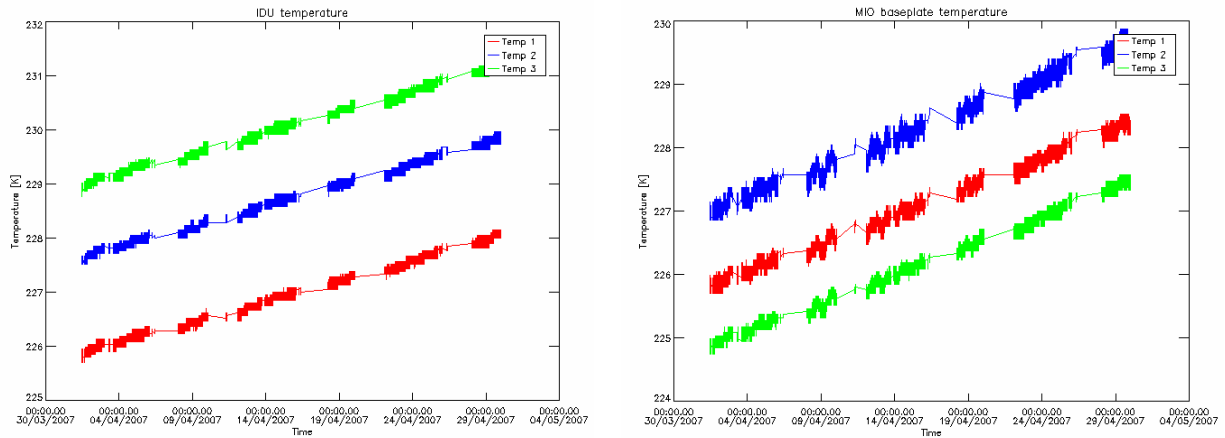
Figure 3 IDU and MIO Base-Plate temperature during reporting period: April 2007.
