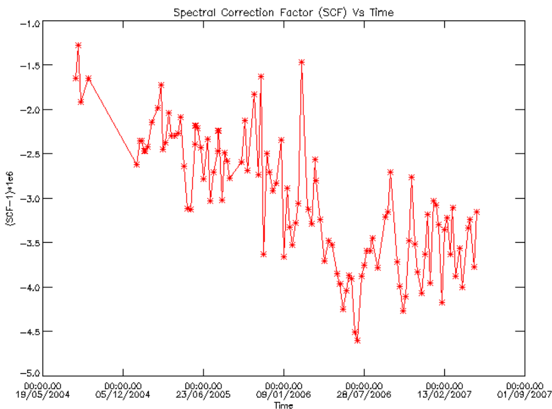
Figure 11 MIPAS Spectral Calibration Factor (SCF) during RR ops updated to end of April 2007.
