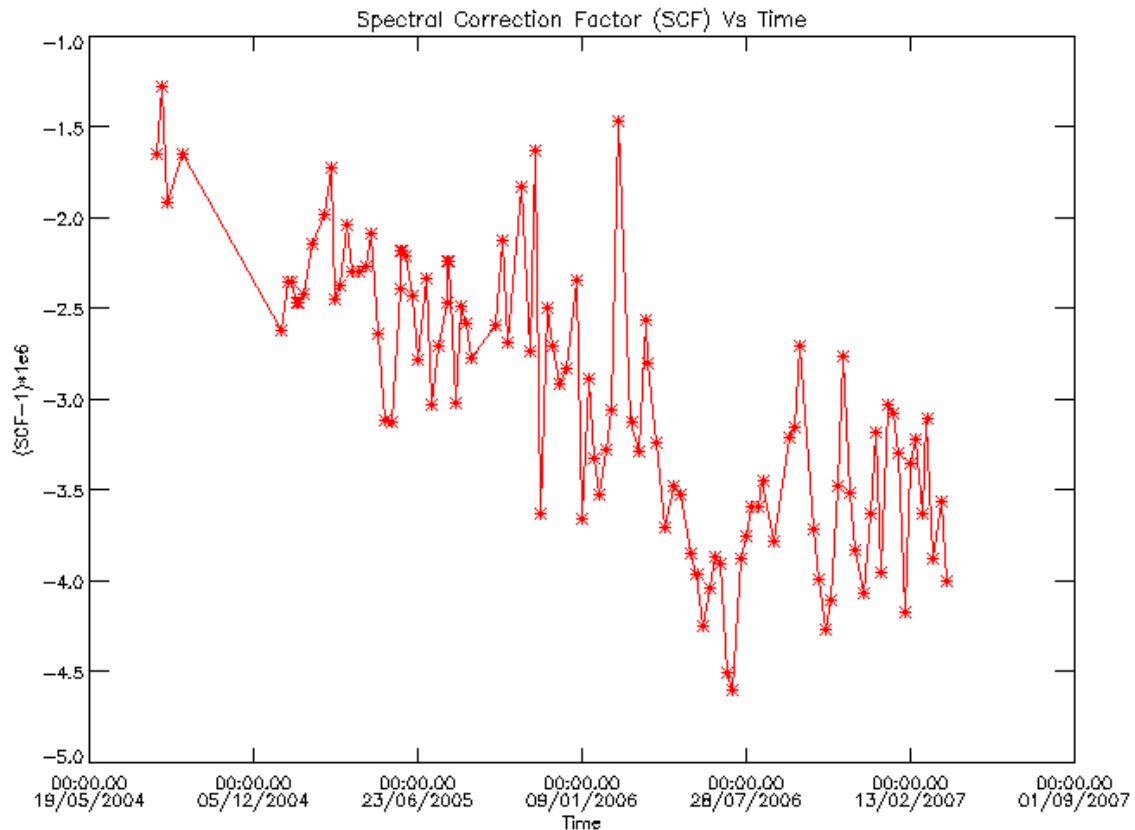
Figure 11 MIPAS Spectral Calibration Factor (SCF) during RR ops updated to end of March 2007.
