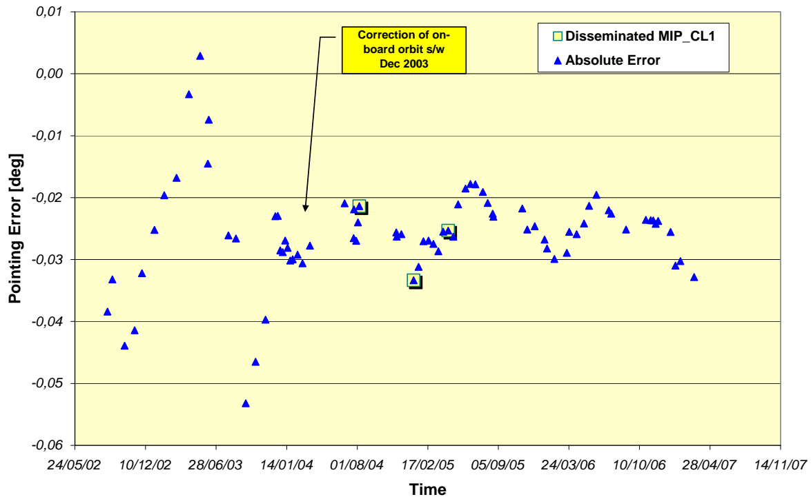
Figure 18 MIPAS long-term pointing error as a function of time: September 2002 – March 2007.
