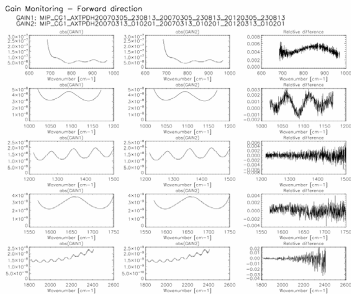
Figure 13 The same as Figure 12 but for a gain measured on 12 Mar 2007.
