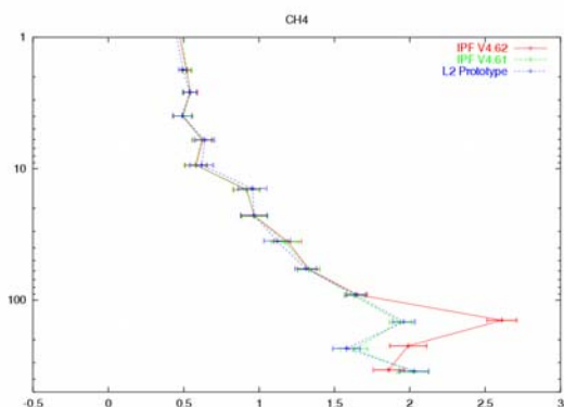
Figure 33 Temperature N 2 O and CH 4 profiles as a function of pressure retrieved with IPF 4.62 and 4.61 compared to the prototype for seq. 16 of orbit 2975. The 4.61 profile is the reference, validated by a IMK balloon flight.
