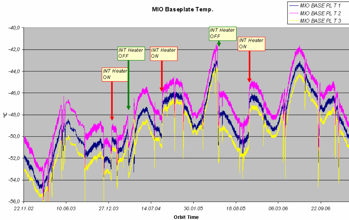
Figure 2 MIO base plate temperatures as a function of time: November 2002 – March 2007 (courtesy of Astrium).
