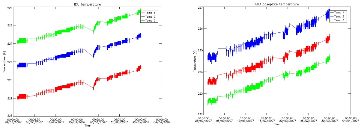
Figure 3 IDU and MIO Base-Plate temperature during reporting period: March 2007.
