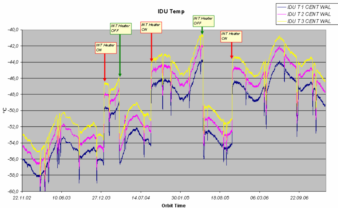
Figure 1 IDU temperatures as a function of time: November 2002 – March 2007 (courtesy of Astrium).
