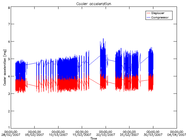
Figure 8 March 2007: Cooler Displacer and Compressor vibration level.
