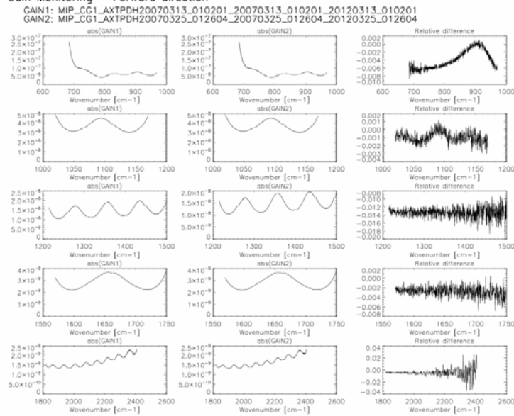
Figure 14 The same as Figure 12 but for a gain measured on 24 Mar 2007.
