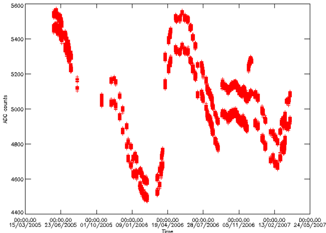
Figure 9 ADC max counts in channel A1 during DS measurements from June 2005 to March 2007.
