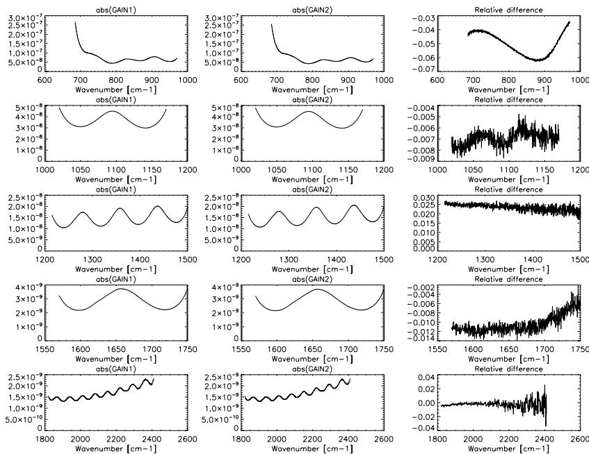
Figure 13 Relative variations of radiometric gain for consecutive disseminated gains in band A (forward direction). The first two plots in each row are the complex modulus of the gain for each of the 5 MIPAS bands, the third plot is the ratio: (abs(w2)-abs(w1))/abs(w1) . This plot refers to a gain measured on 1 Dec 2006.
