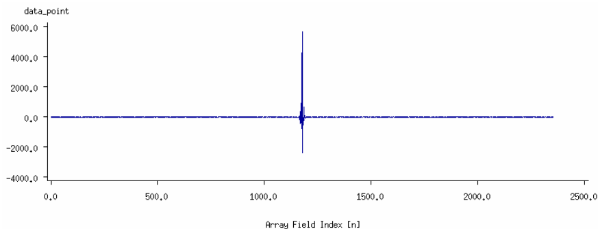
Figure 28 IGM recorded in the deep space measurement and stored in the new correct ADF.
