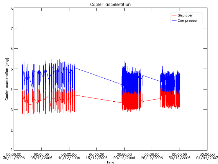
Figure 10 December 2006: Cooler Displacer and Compressor vibration level.
