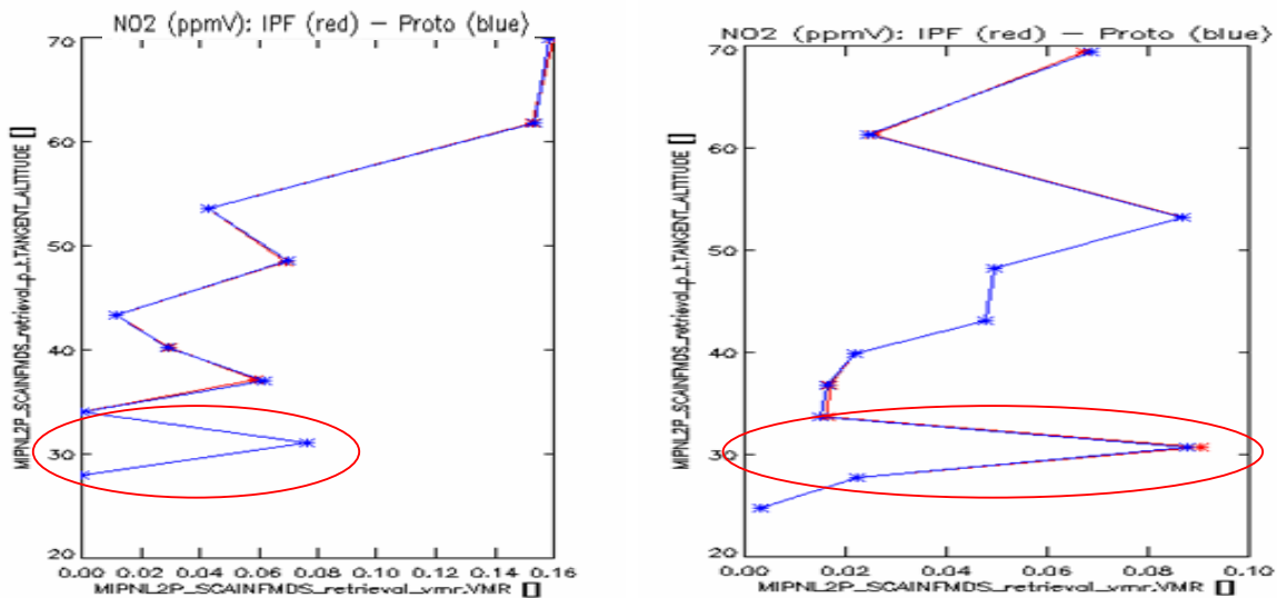
Figure 32 NO2 profiles obtained with the IPF and prototype for two particular scan of 6 June 2003 in Antarctic winter condition, highlighted in red are the region around 30 km with sudden increase of NO2 value, which has no physical meaning. Note the degraded profile shape, namely the zigzag and the zero value.
