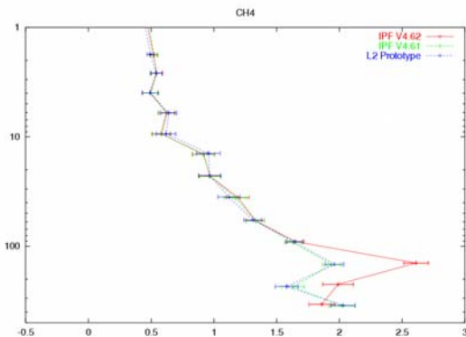
Figure 31 Temperature N2O and CH4 profiles as a function of pressure retrieved with IPF 4.62 and 4.61 compared to the prototype for seq. 16 of orbit 2975. The 4.61 profile is the reference, validated by a IMK balloon flight.
