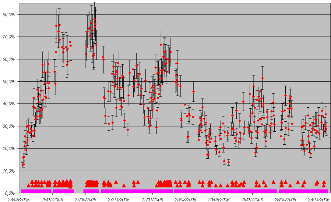
Figure 8 Occurrence of -4% differential speed error relative to measurement time since May 2005 (courtesy of Astrium).
