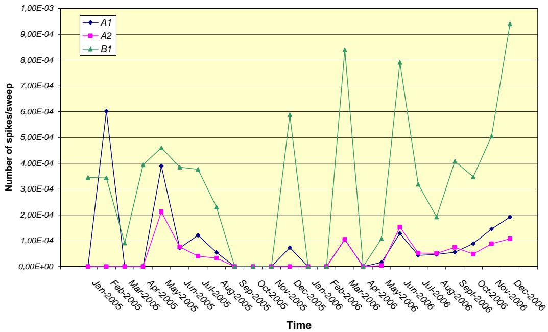
Figure 20 MIPAS long-term monitoring of number of detected/corrected spikes in the detectors A1, A2, B1. In the y-axis is reported the monthly average of detected spikes for each measured sweep.
