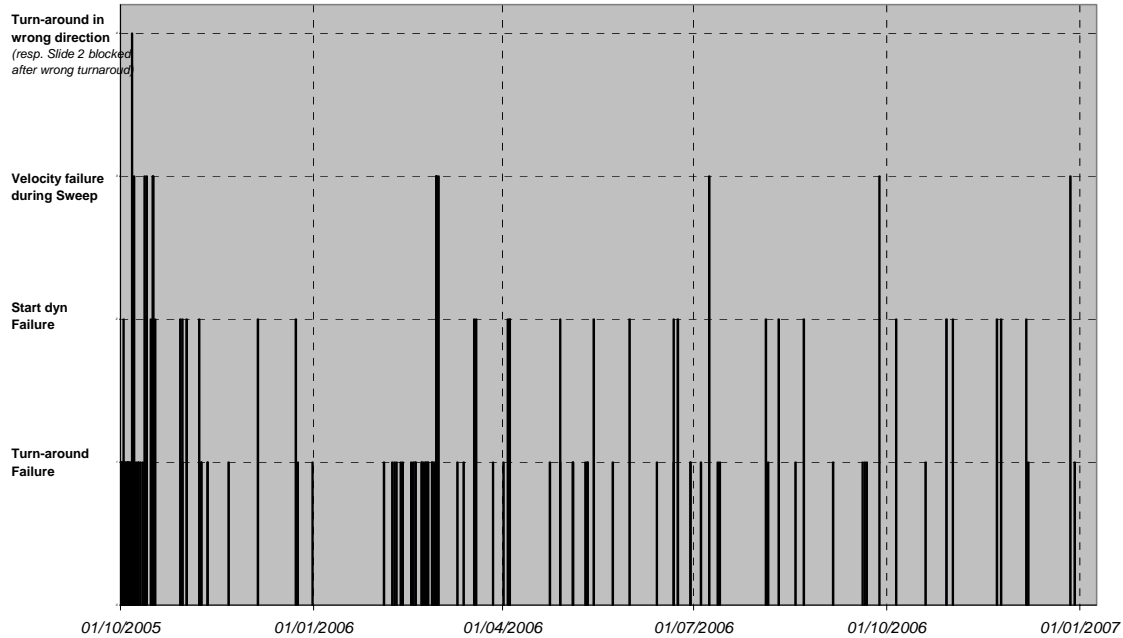
Figure 7 INT anomalies since Oct 2005 (courtesy of Astrium).
