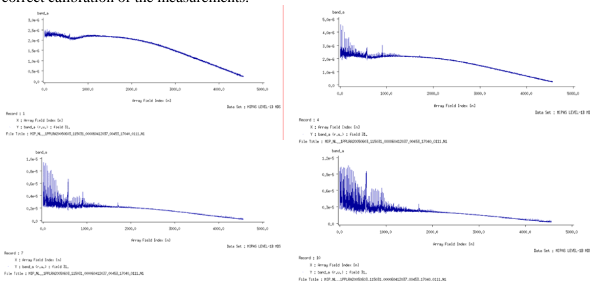
Figure 29 Example of badly calibrated spectra obtained with the old ADFs.
