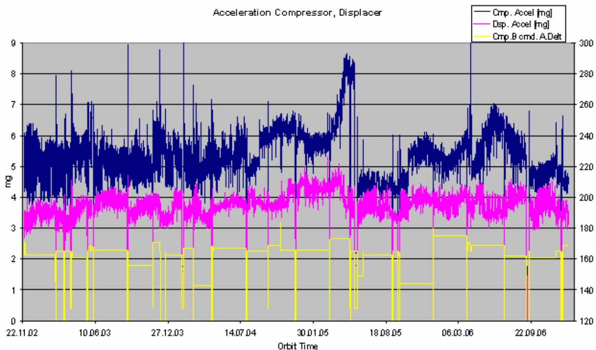
Figure 9 Cooler Displacer and Compressor vibration level, historical trend from 2002 (courtesy of Astrium).
