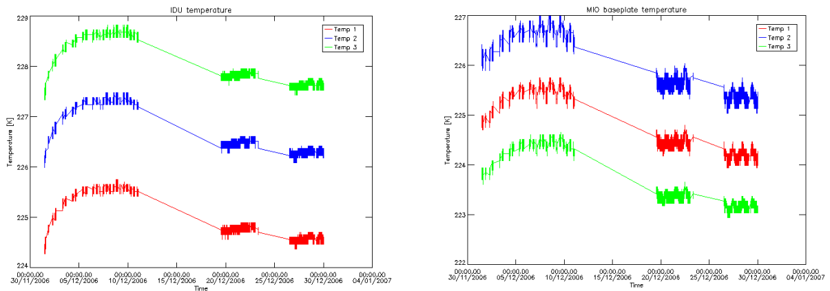
Figure 3 IDU and MIO Base-Plate temperature during reporting period: December 2006.
