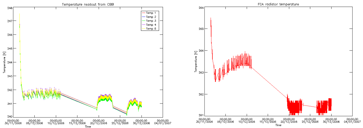
Figure 4 CBB and FCA radiator temperature during reporting period: December 2006.
