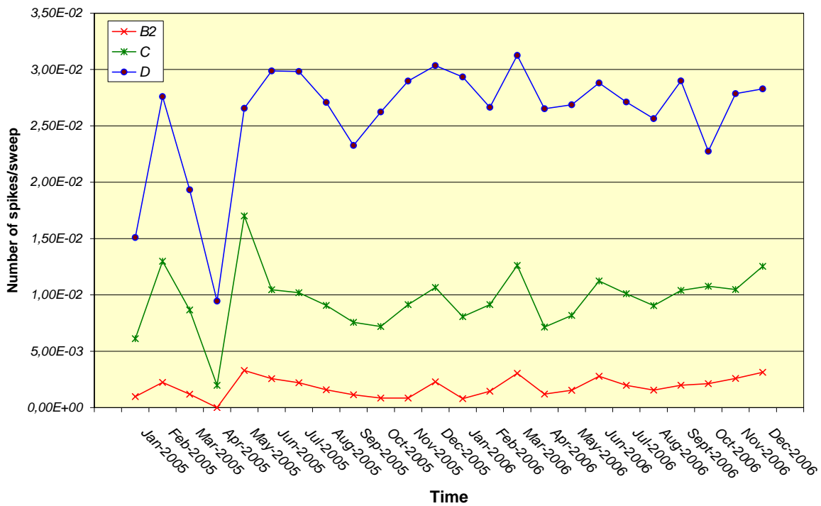
Figure 21 MIPAS long-term monitoring of number of detected/corrected spikes in the detectors B2, C and D. In the y-axis is reported the monthly average of detected spikes for each measured sweep.
