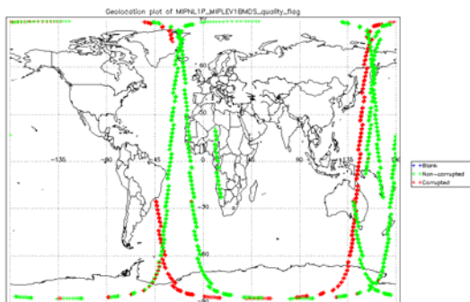
Figure 24 L1b PCD quality flag, corrupted sweep detected for 3 Oct 2005 L1b spectra
