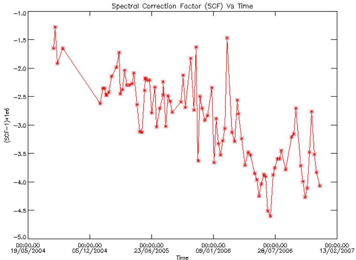
Figure 12 MIPAS Spectral Calibration Factor (SCF) during RR ops updated to end of December 2006.
