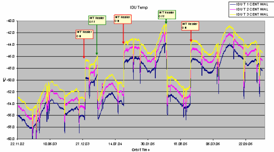
Figure 1 IDU temperatures as a function of time: November 2002 – December 2006 (courtesy of Astrium).
