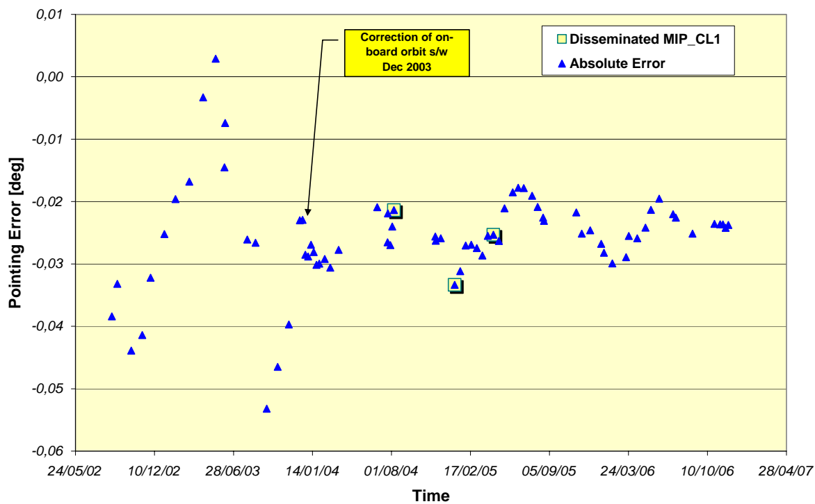
Figure 19 MIPAS long-term pointing error as a function of time: September 2002 – December 2006.
