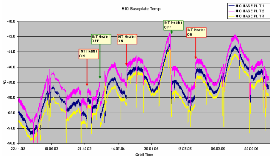
Figure 2 MIO base plate temperatures as a function of time: November 2002 – December 2006 (courtesy of Astrium).
