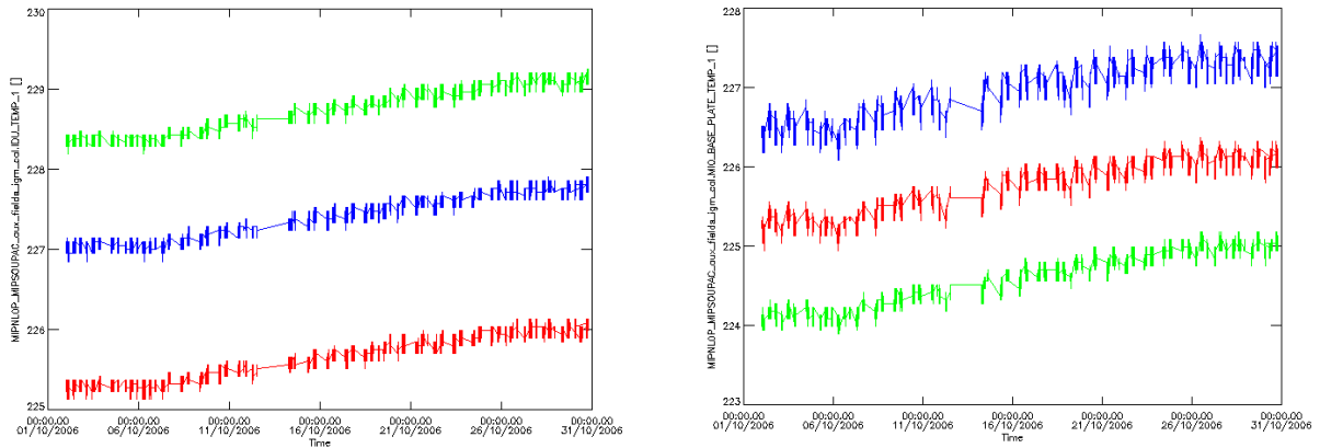
Figure 3 IDU and MIO Base-Plate temperature during reporting period: October 2006.
