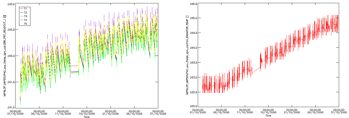
Figure 4 CBB and FCA radiator temperature during reporting period: October 2006.
