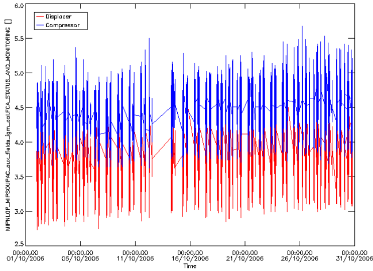
Figure 9 October 2006: Cooler Displacer and Compressor vibration level.
