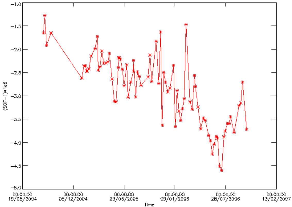
Figure 12 MIPAS Spectral Calibration Factor (SCF) during RR ops updated to end of October 2006.
