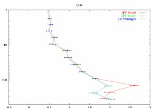
Figure 31 Temperature N2O and CH4 profiles as a function of pressure retrieved with IPF 4.62 and 4.61 compared to the prototype for seq. 16 of orbit 2975. The 4.61 profile is the reference, validated by a IMK balloon flight.
