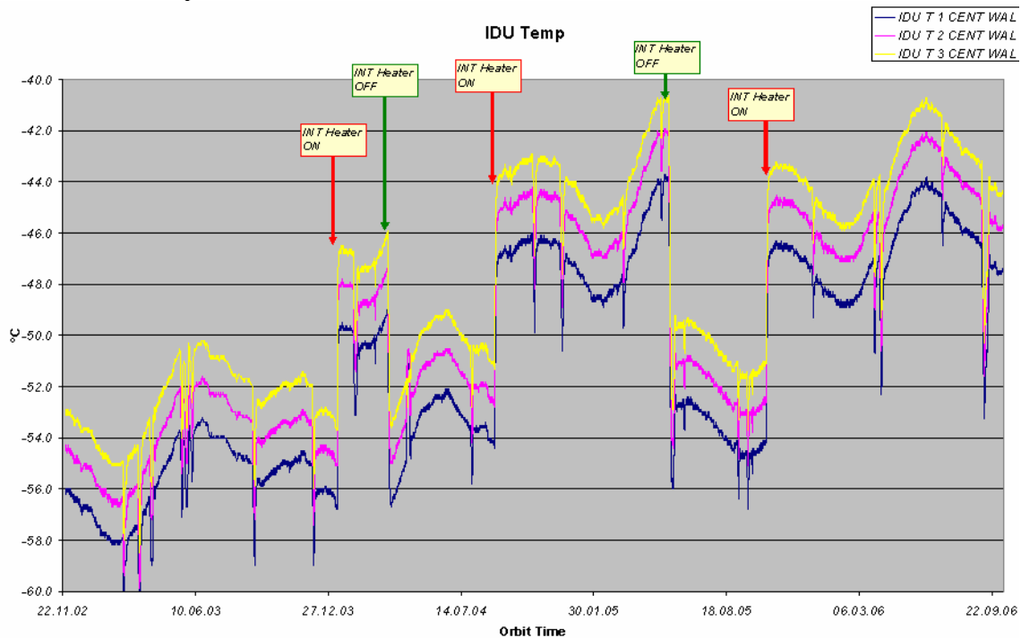
Figure 1 IDU temperatures as a function of time: November 2002 – October 2006 (courtesy of Astrium).
