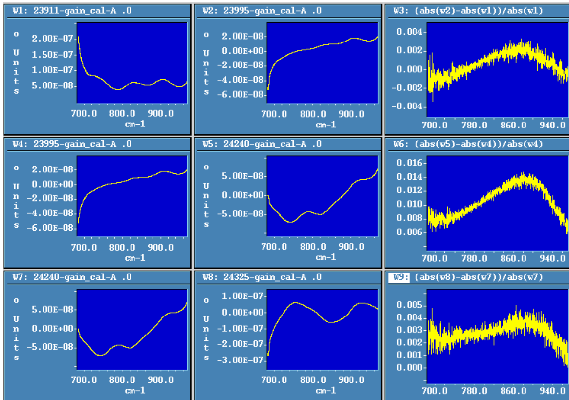
Figure 15 Relative variations of radiometric gain for consecutive disseminated gains in band A during October 2006 operations. The first two plots in each row are the real part of the gain plotted versus the wave-number, the third plot is the ratio: (abs(w2)-abs(w1))/abs(w1) , where abs is the complex modulus. The ratio gives the gain increase with respect to the reference w1 (last disseminated gain).
