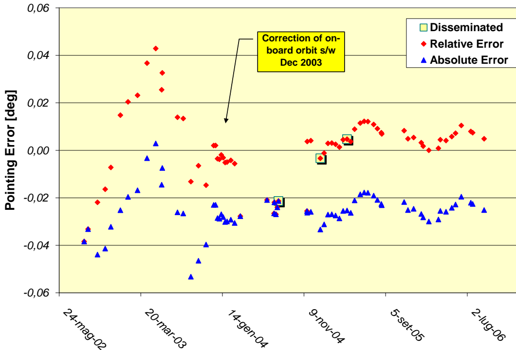
Figure 20 MIPAS long-term pointing error as a function of time: September 2002 – October 2006.
