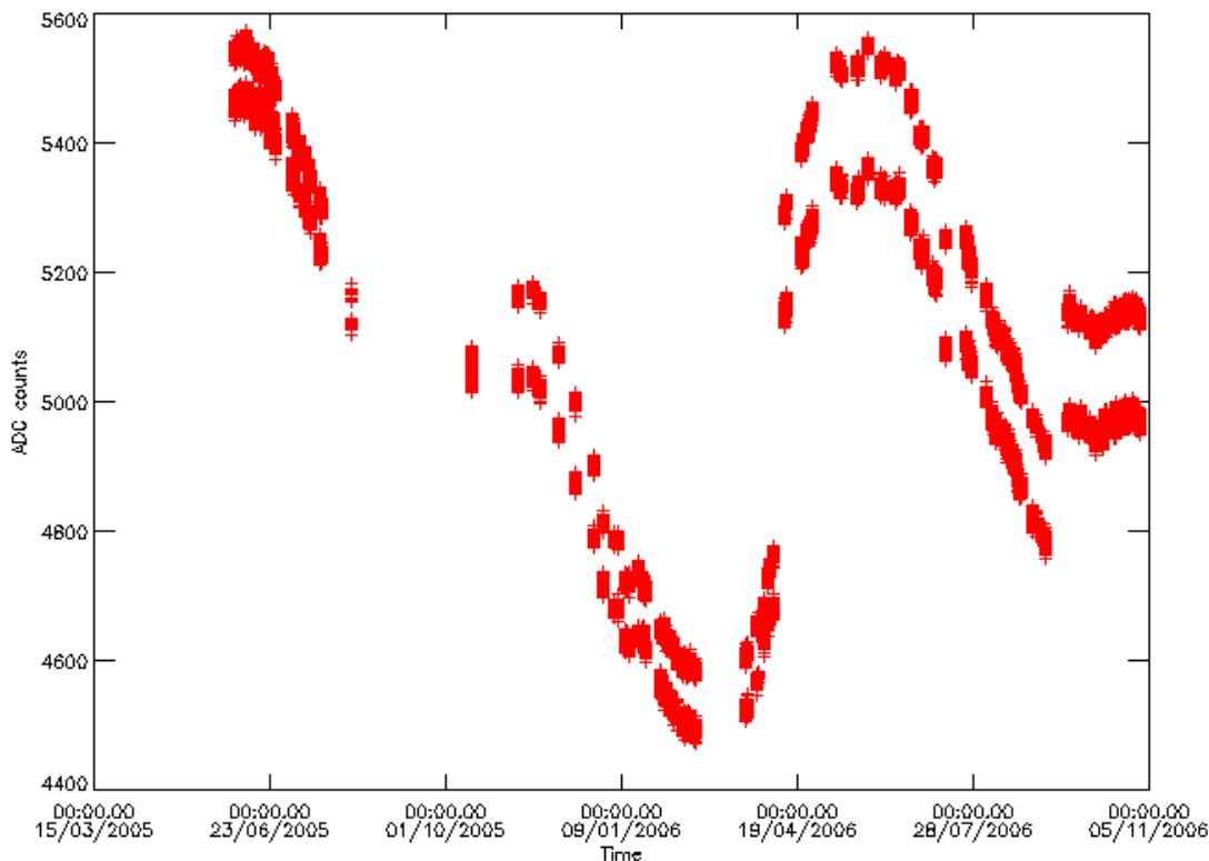
Figure 5 ADC max counts in channel A1 during DS measurements: from June 2005 to October 2006.
