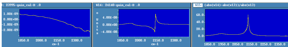
Figure 13 Corruption in band D observed for orbit 24140.
