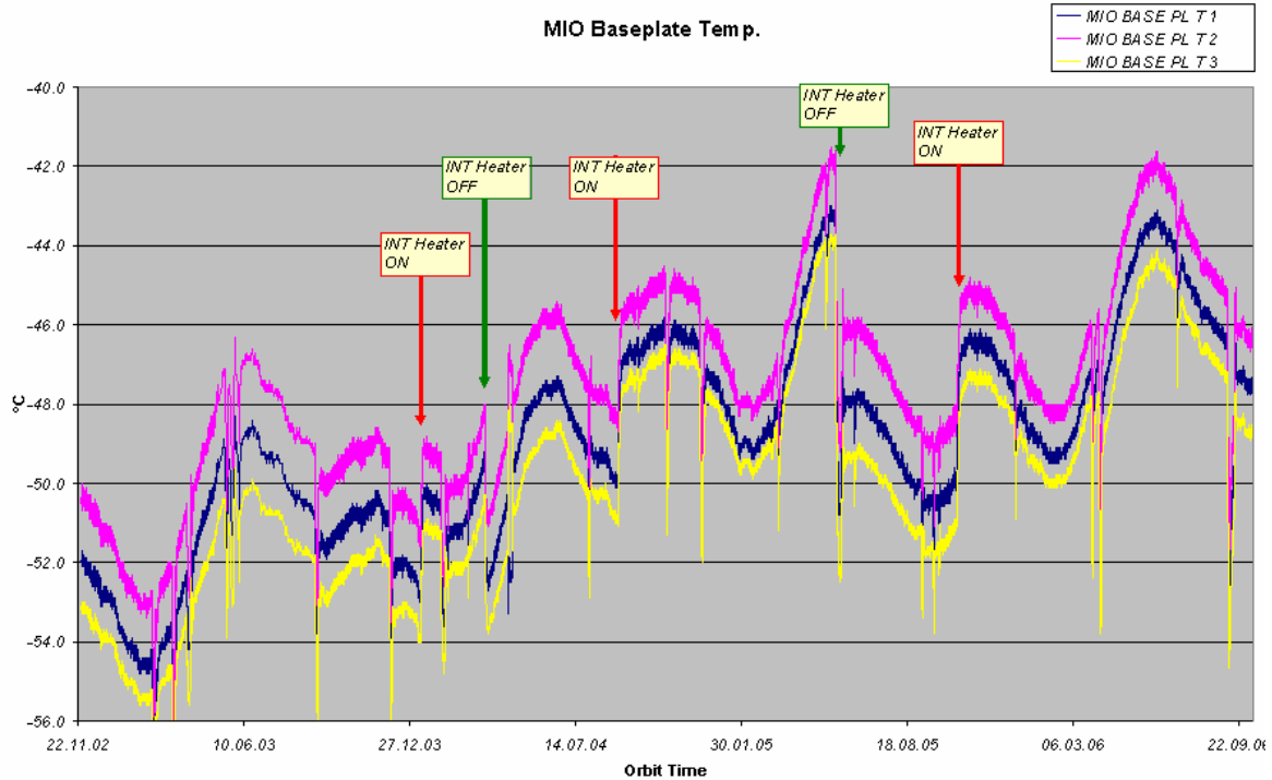
Figure 2 MIO base plate temperatures as a function of time: November 2002 – October 2006 (courtesy of Astrium).
