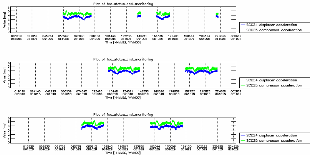
Figure 10 Cooler Displacer and Compressor vibration level observed on 6 th , 16 th and 29 th October 2006.
