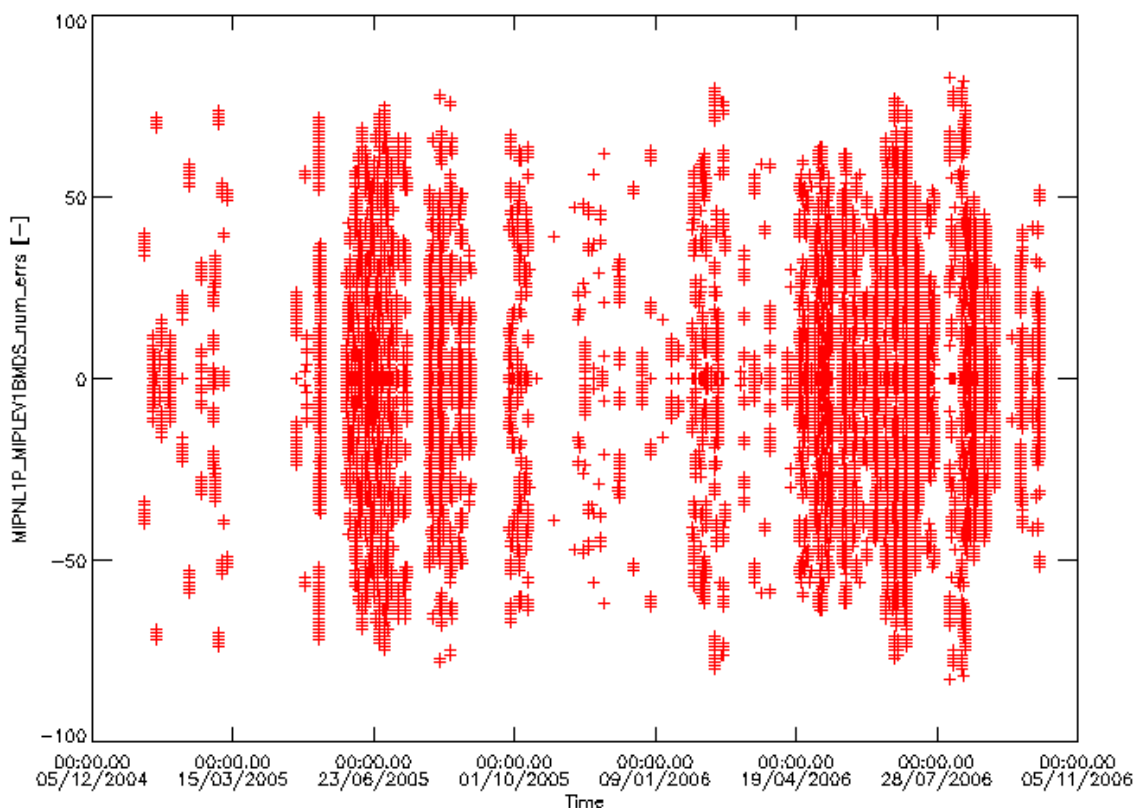
Figure 21 MIPAS long-term FCE values: January 2005 - October 2006.
