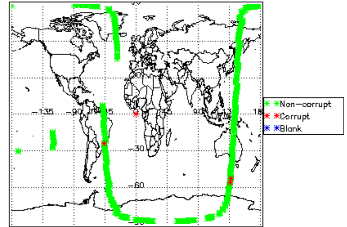
Geolocation plot of MIPNL1P_MIPLEV1BMDS_quality_flag
