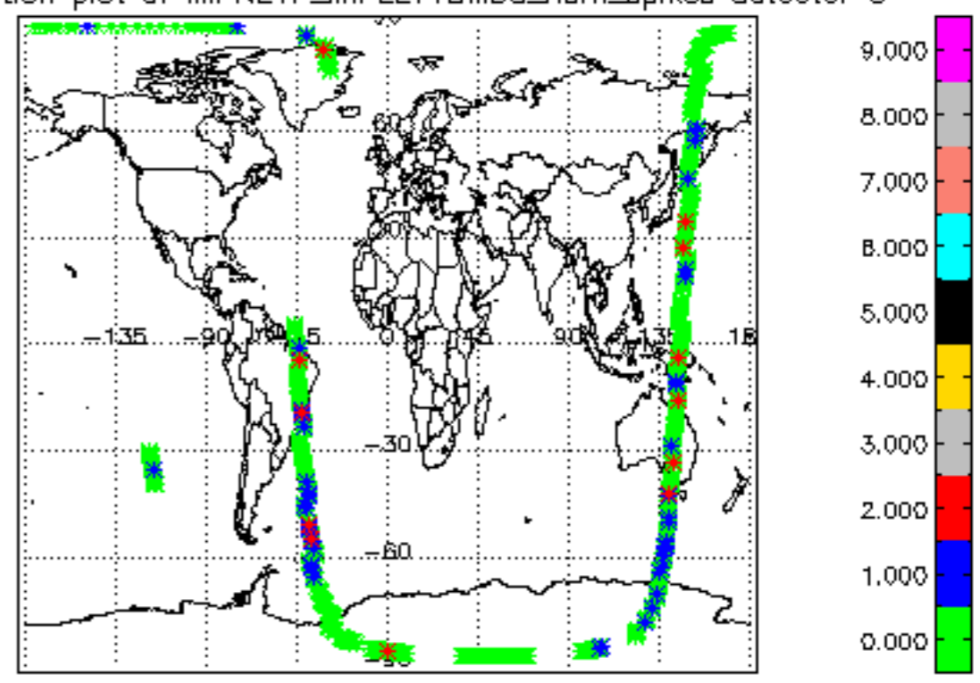
Geolocation plot of MIPNL1P_MIPLEV1BMDS_num_spikes detector C
