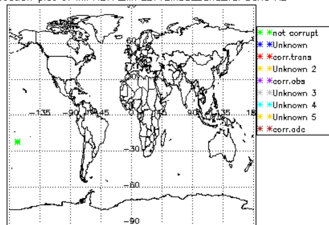
Geolocation plot of MIPNL1P_MIPLEV1BMDS_band_val band AB
