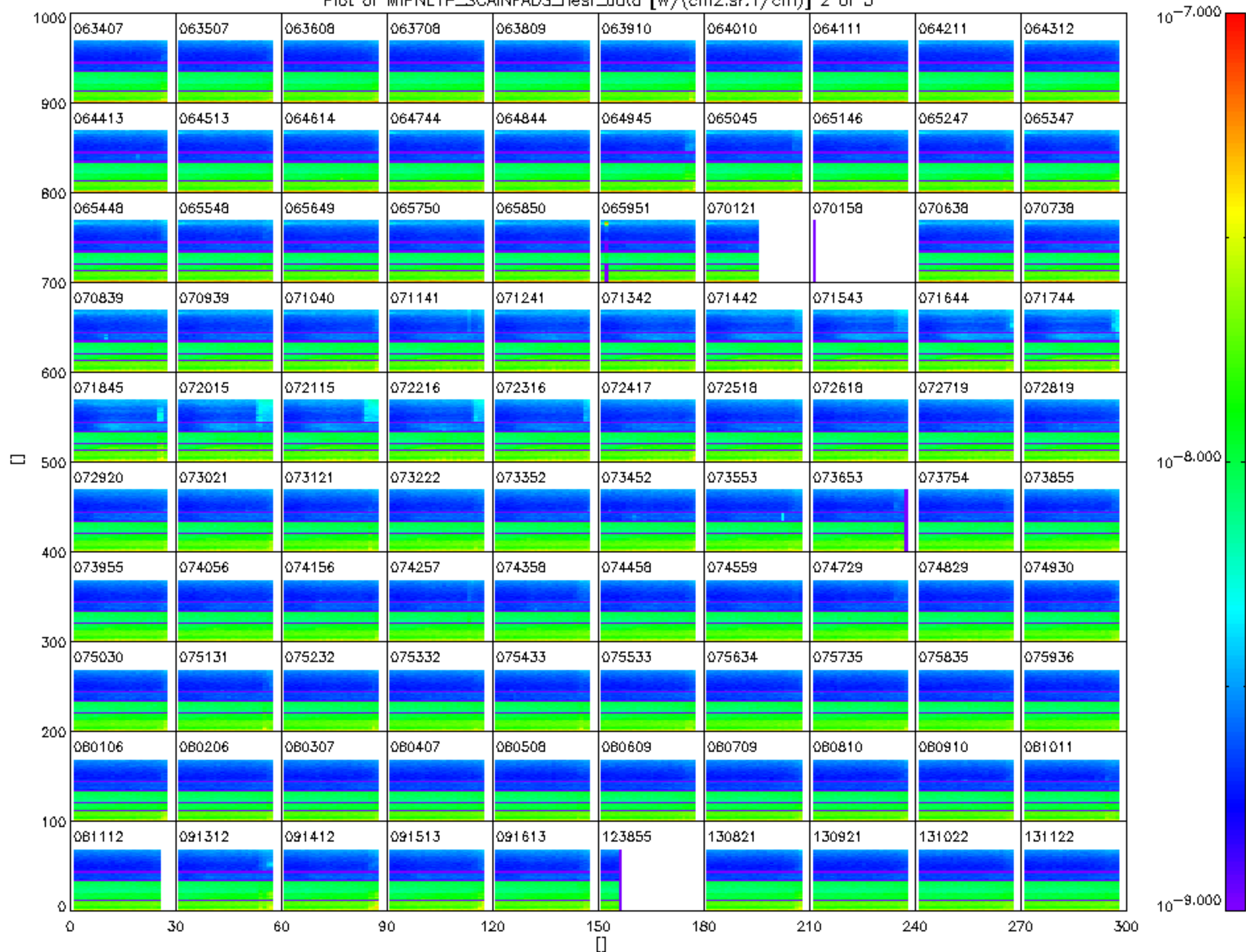
Plot of MIPNL1P_SCAINFADS_nesr_data [W/(cm2.sr.1/cm)] 2 of 5
