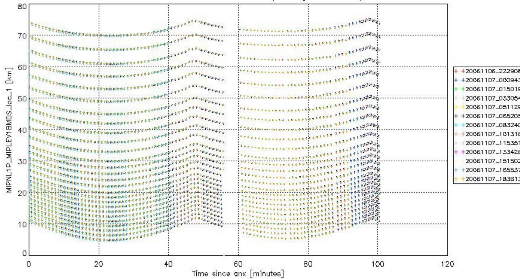
Plot of MIPNL1P_MIPLEV1BMD5_loc_1 against relative time within orbit. The colours indicate distinct orbits (see legend for anx).
