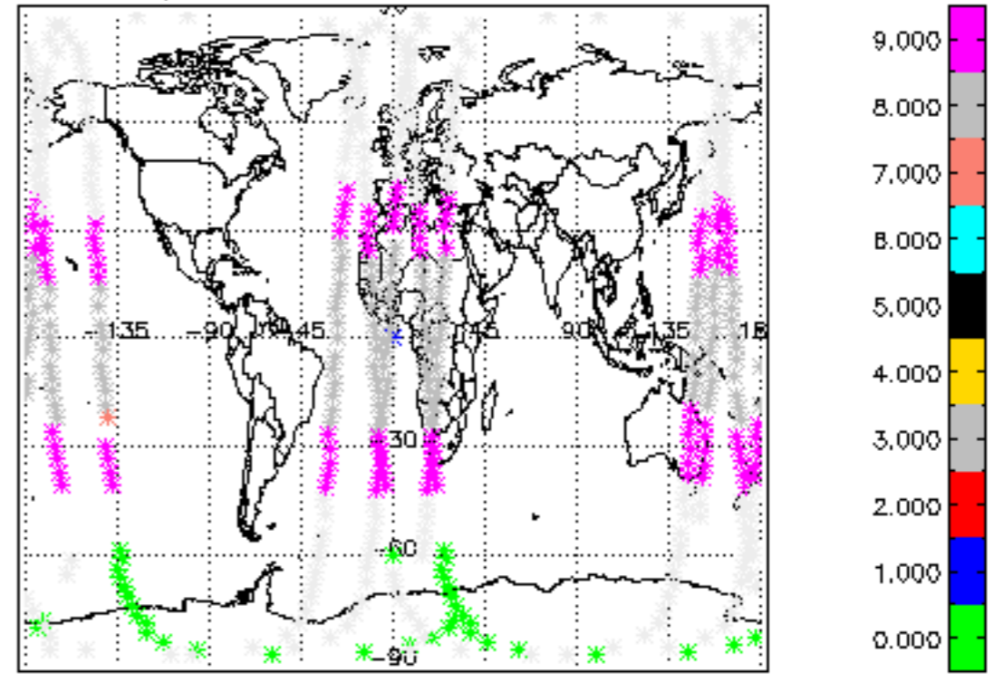
Geolocation plot of MIPNL1P_SUMQUAADS.num_corr_ins
