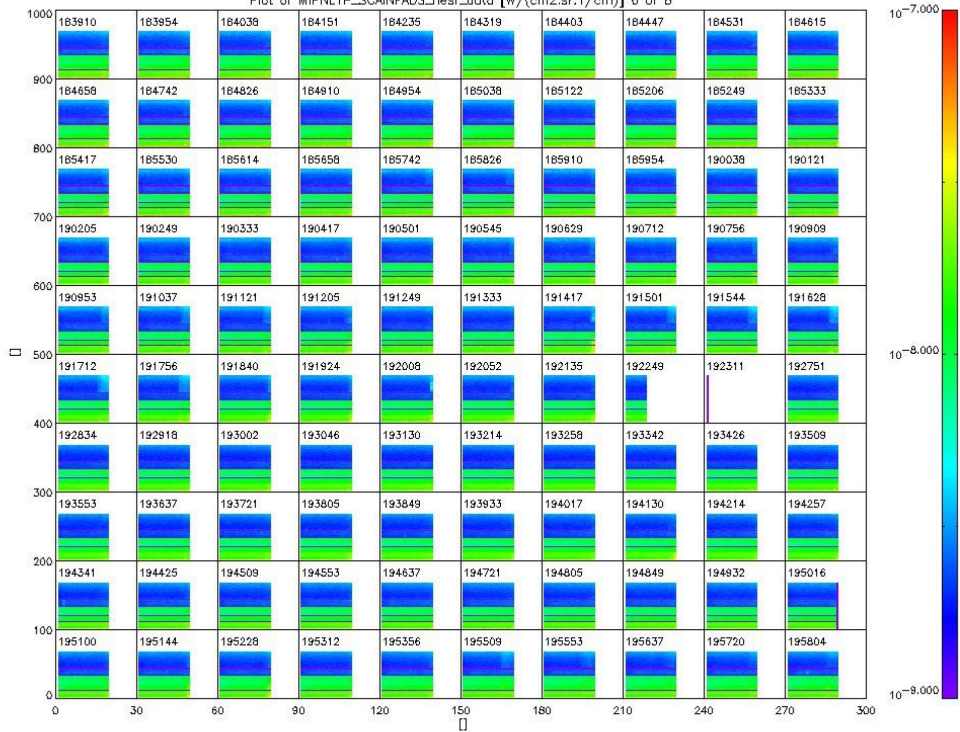
Plot of MIPNL1P_SCAINFADS_near_data [W/(cm 2 .sr.1/cm)] 6 of 8
