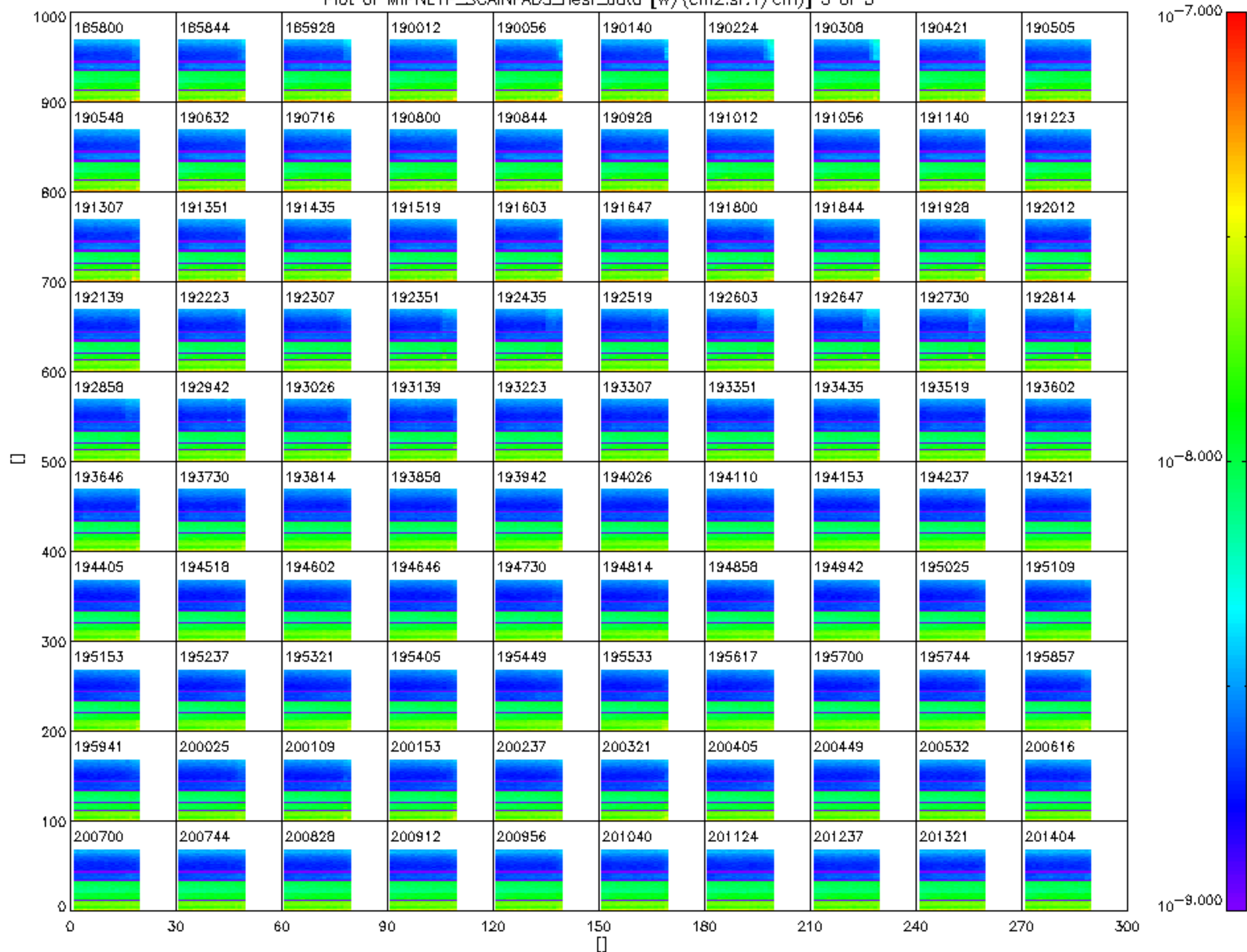
Plot of MIPNL1P_SCAINFADS_nesr_data [W/(cm2.sr.1/cm)] 3 of 5
