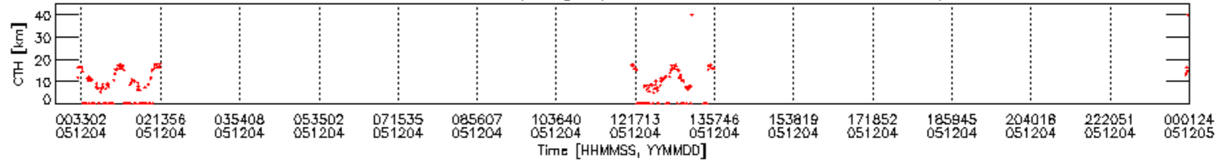
Plot of estimated cloud top height (40.000000 indicates non-nominal scan)
