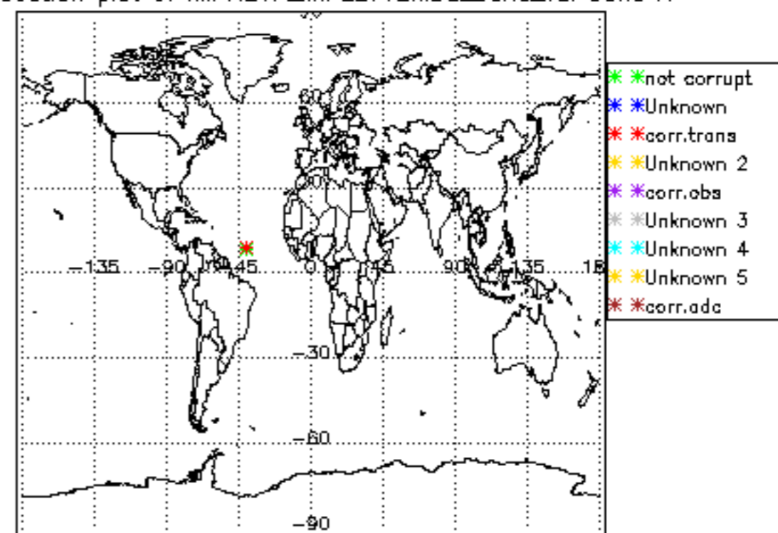
Geolocation plot of MIPNL1P_MIPLEV1BMDS_band_val band A
