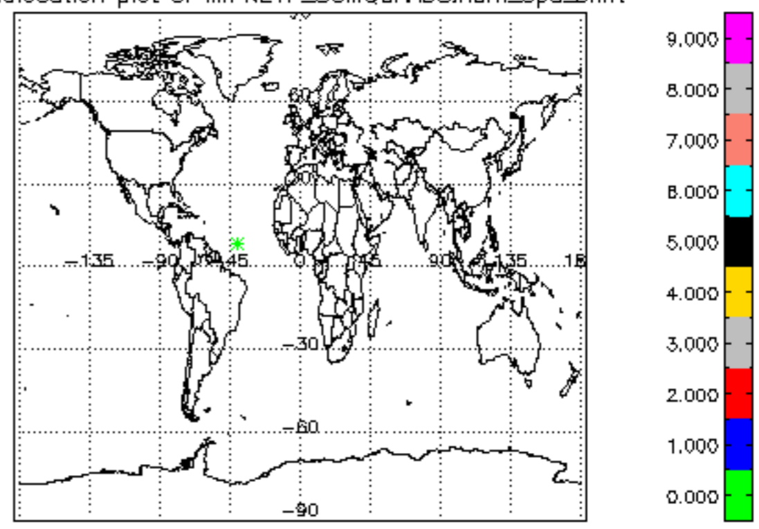
Geolocation plot of MIPNL1P_SUMQUAADS.num_opd_shift
