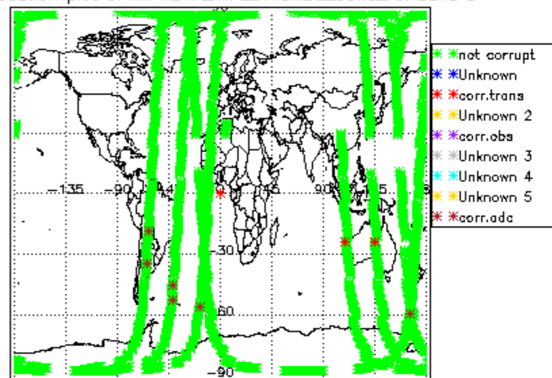
Geolocation plot of MIPNL1P_MIPLEV1BMDS_band_Lval band D
