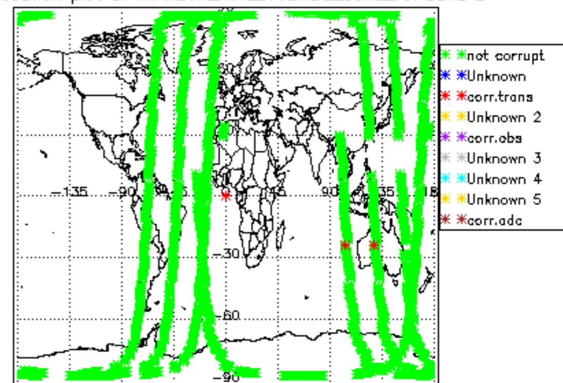
Geolocation plot of MIPNL1P_MIPLEV1BMDS_band_Lval band B
