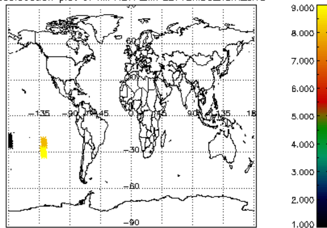
Geolocation plot of MIPNL1P_MIPLEV1BMDS_num_errs
