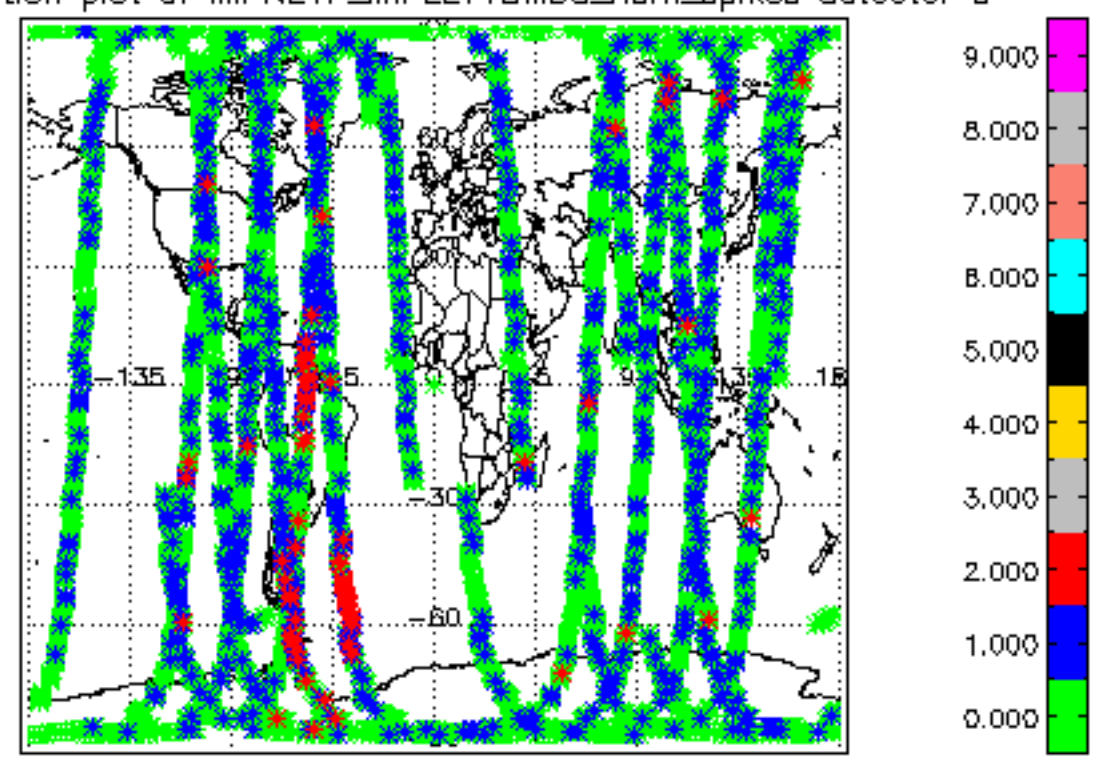
Geolocation plot of MIPNL1P_MIPLEV1BMDS_num_spikes detector D
