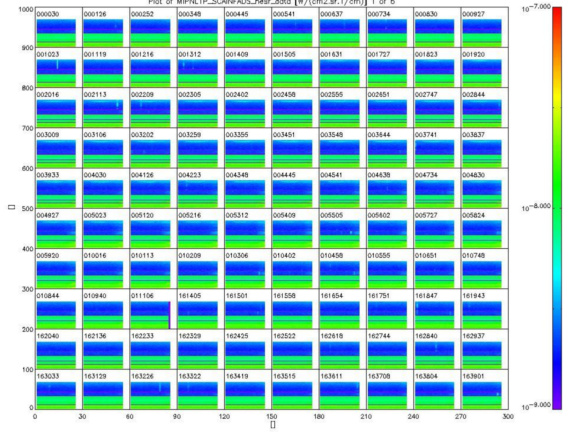
Plot of MIPNL1P_SCAINFADS_near_data [W/(cm2.ar.1/cm)] 1 of 6
