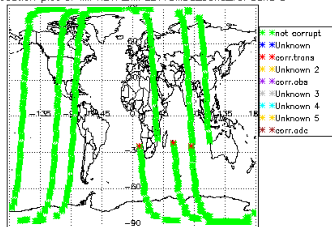
Geolocation plot of MIPNL1P_MIPLEV1BMDS_band_val band D
