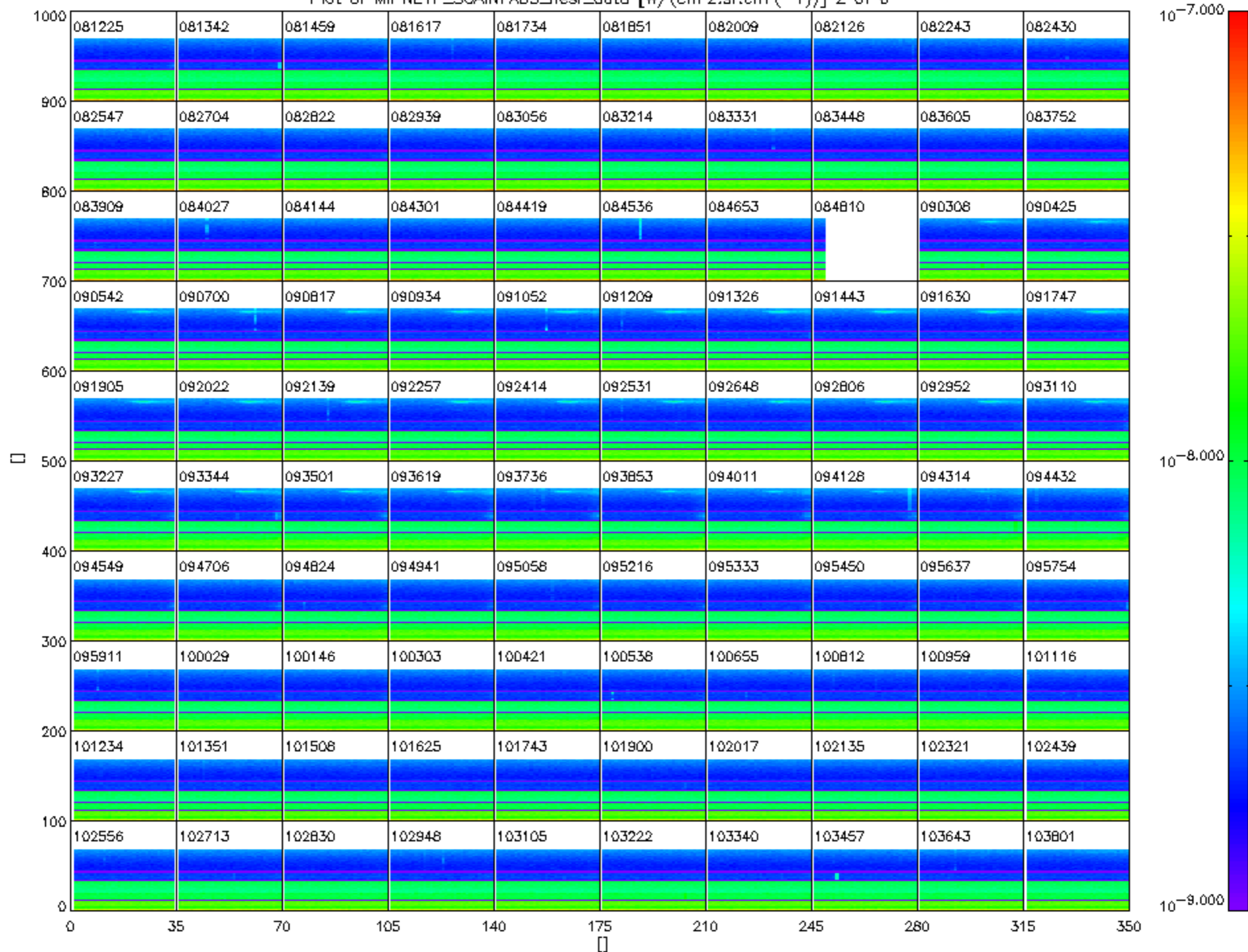
Plot of MIPNL1P_SCAINFADS_nesr_data [W/(cm 2 .sr.cm -1 )] 2 of 6
