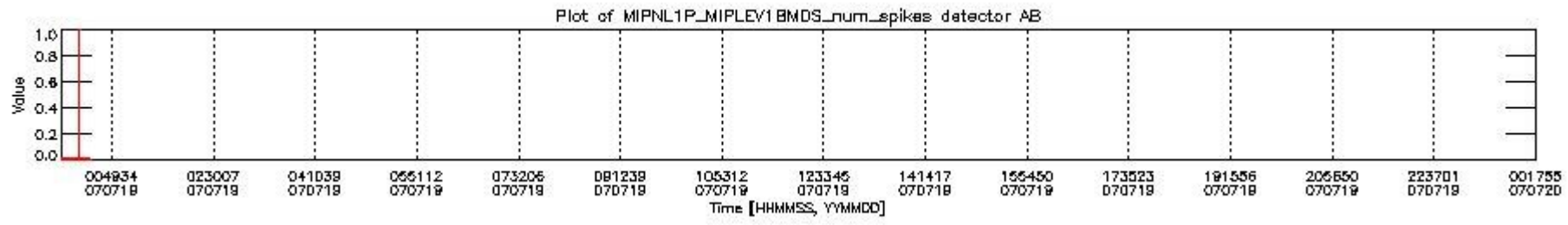
mipas_daily_report_level1_OFI_MIPAS_4_67_P_20070719_20.PNG
