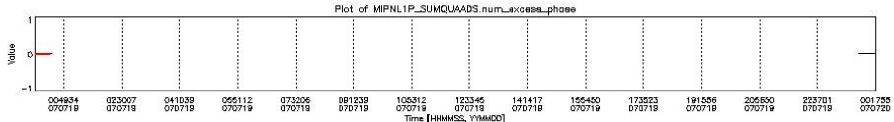
mipas_daily_report_level1_OFI_MIPAS_4_67_P_20070719_8.PNG
