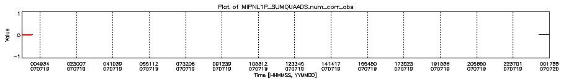
mipas_daily_report_level1_OFI_MIPAS_4_67_P_20070719_6.PNG
