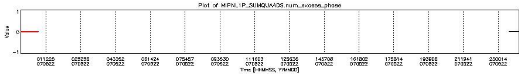
mipas_daily_report_level1_OFI_MIPAS_4_67_P_20070522_8.PNG
