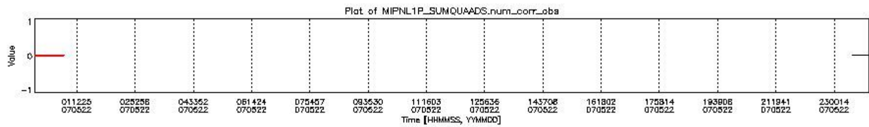
mipas_daily_report_level1_OFI_MIPAS_4_67_P_20070522_6.PNG
