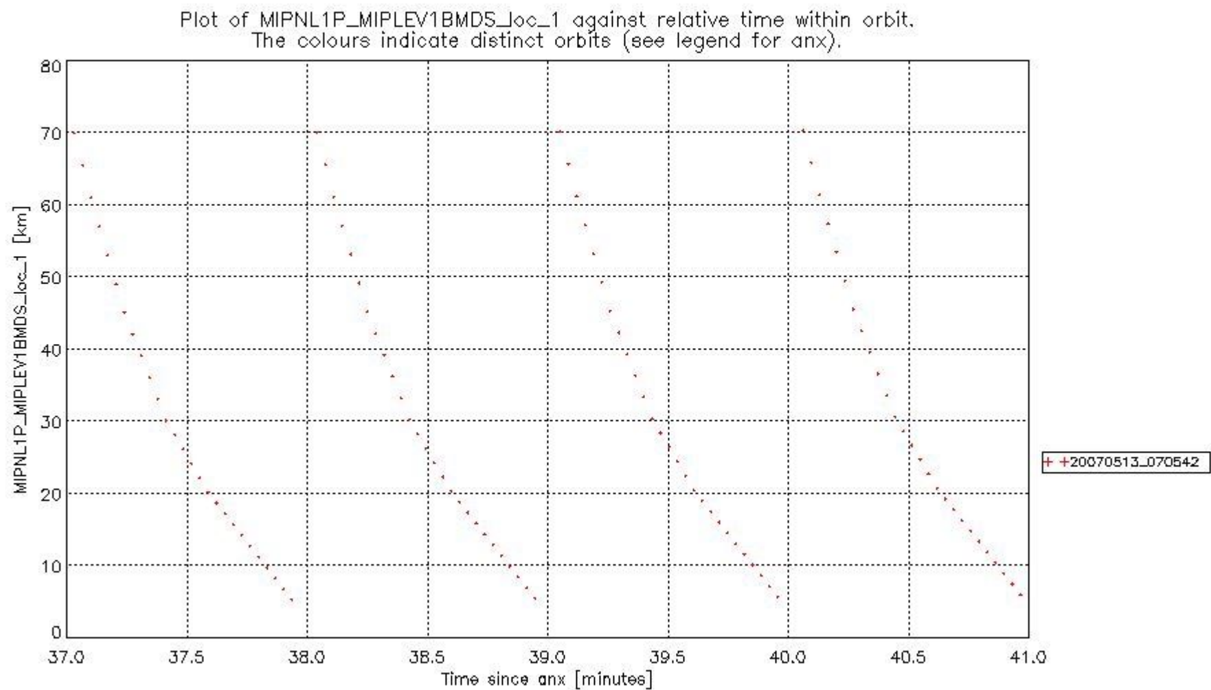
mipas_daily_report_level1_OFL_MIPAS_4_67_P_20070513_50.PNG
