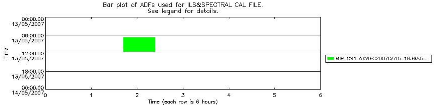
mipas_daily_report_level1_OFI_MIPAS_4_67_P_20070513_53.PNG
