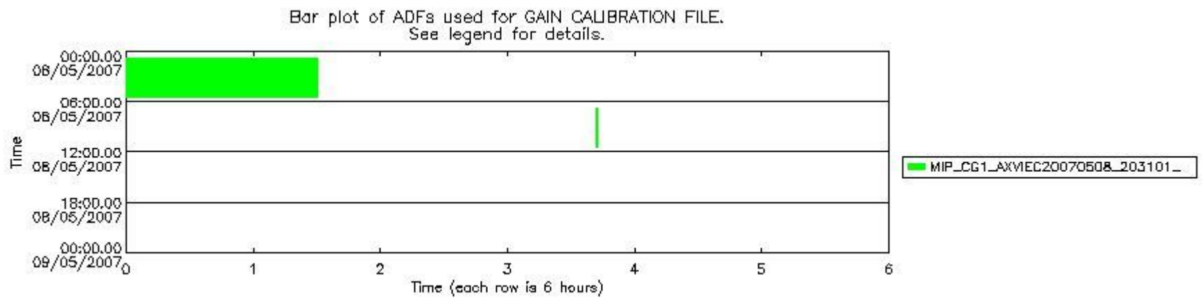
mipas_daily_report_level1_OFL_MIPAS_4_67_P_20070508_54.PNG
