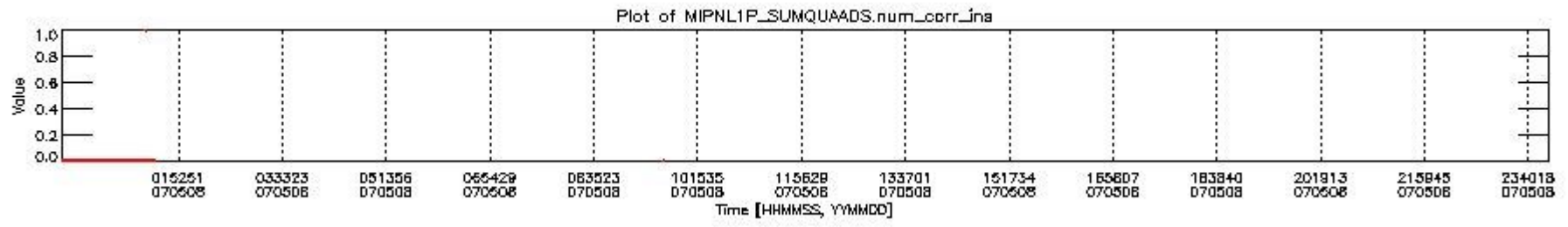
mipas_daily_report_level1_OFI_MIPAS_4_67_P_20070508_4.PNG
