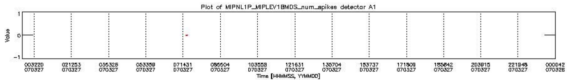
mipas_daily_report_level1_OFL_MIPAS_4_67_P_20070327_16.PNG
