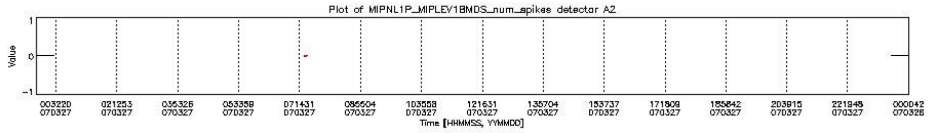
mipas_daily_report_level1_OFL_MIPAS_4_67_P_20070327_18.PNG
