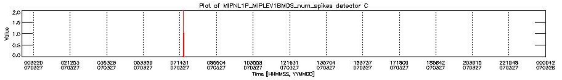
mipas_daily_report_level1_OFL_MIPAS_4_67_P_20070327_24.PNG
