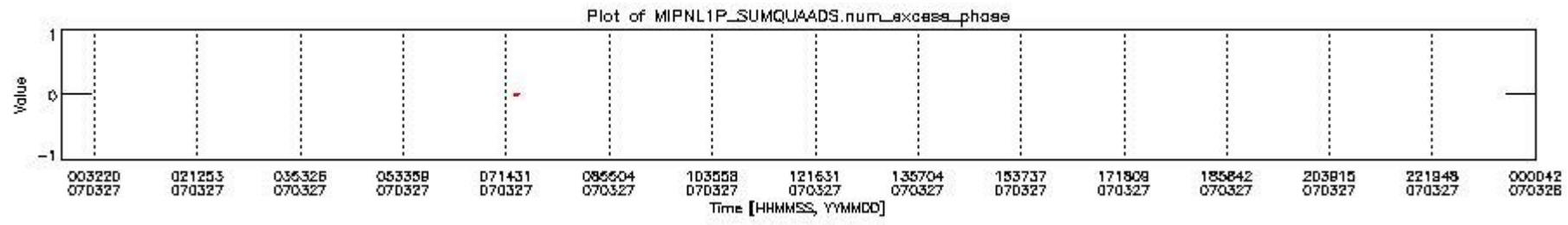
mipas_daily_report_level1_OFI_MIPAS_4_67_P_20070327_8.PNG
