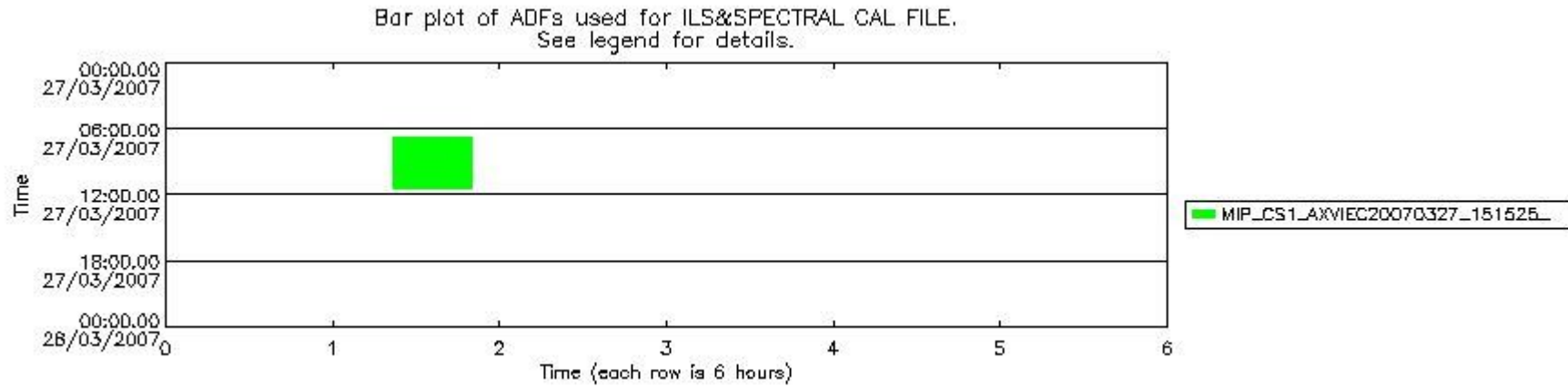
mipas_daily_report_level1_OFI_MIPAS_4_67_P_20070327_53.PNG
