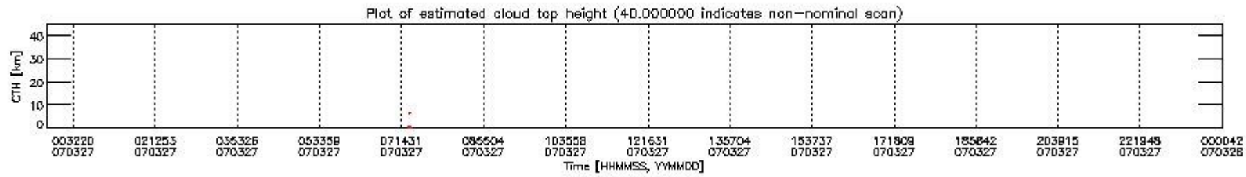
mipas_daily_report_level1_OFL_MIPAS_4_67_P_20070327_51.PNG
