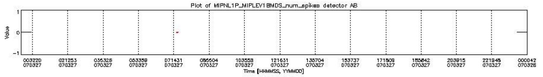
mipas_daily_report_level1_OFL_MIPAS_4_67_P_20070327_20.PNG
