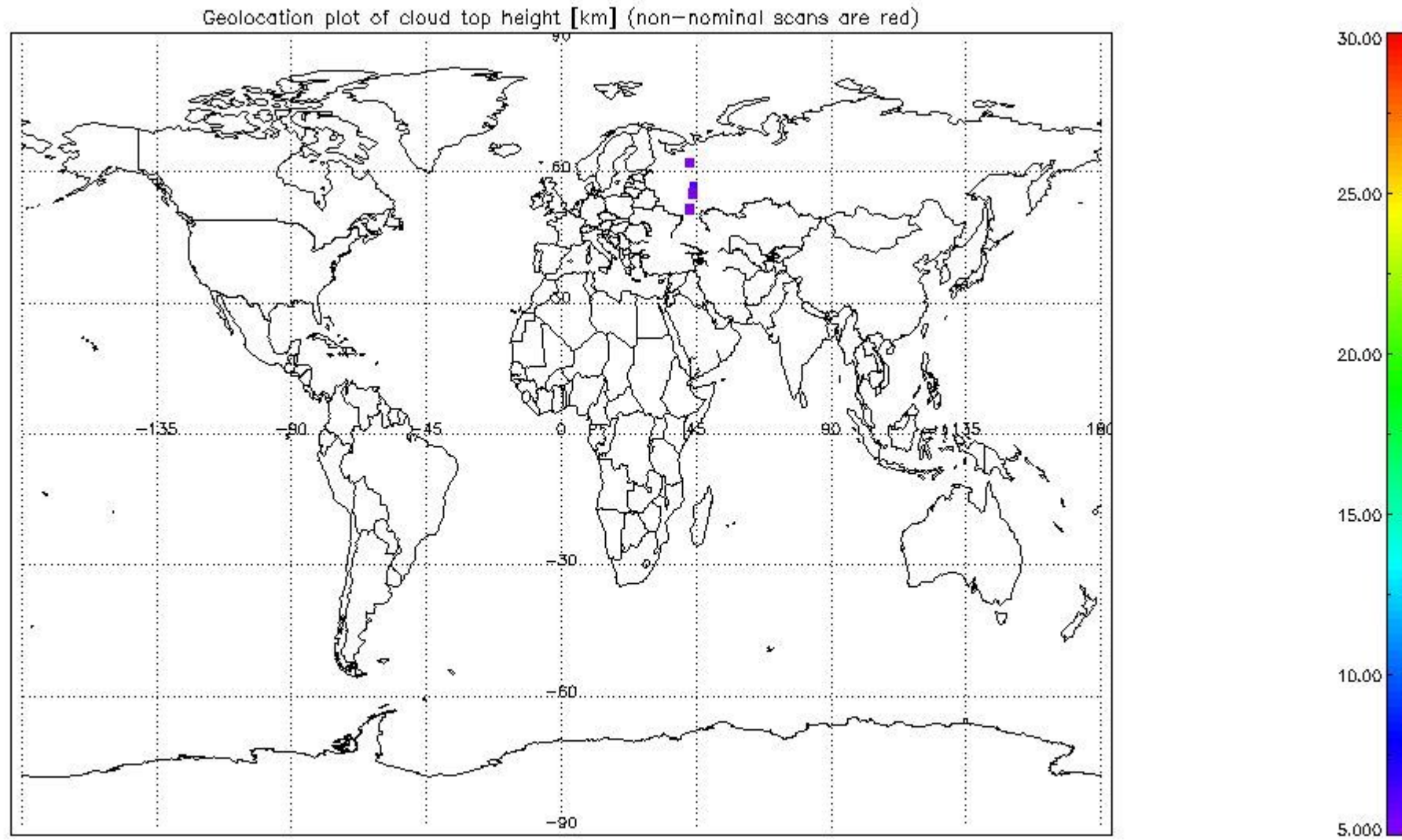
mipas_daily_report_level1_OFL_MIPAS_4_67_P_20070327_51.PNG
