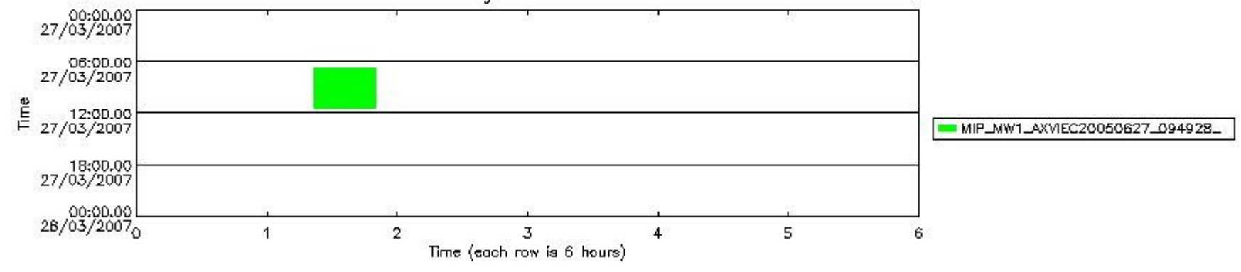
mipas_daily_report_level1_OFL_MIPAS_4_67_P_20070327_58.PNG
