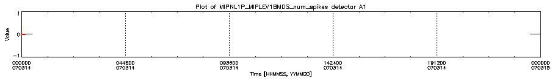
mipas_daily_report_level1_OFL_MIPAS_4_67_P_20070314_16.PNG
