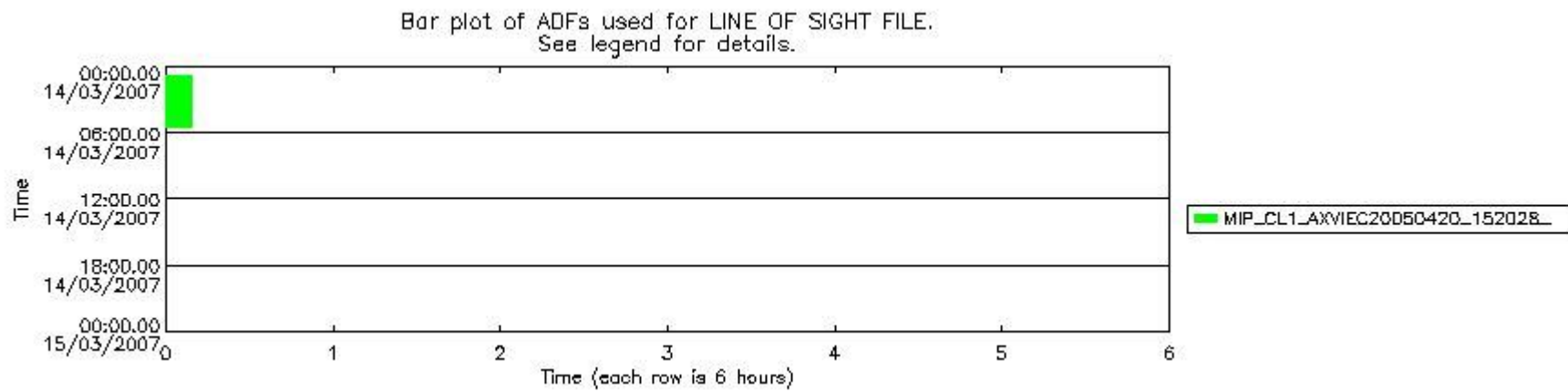
mipas_daily_report_level1_OFL_MIPAS_4_67_P_20070314_57.PNG
