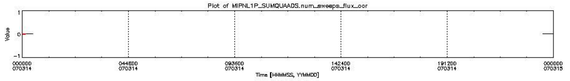
mipas_daily_report_level1_OFL_MIPAS_4_67_P_20070314_12.PNG
