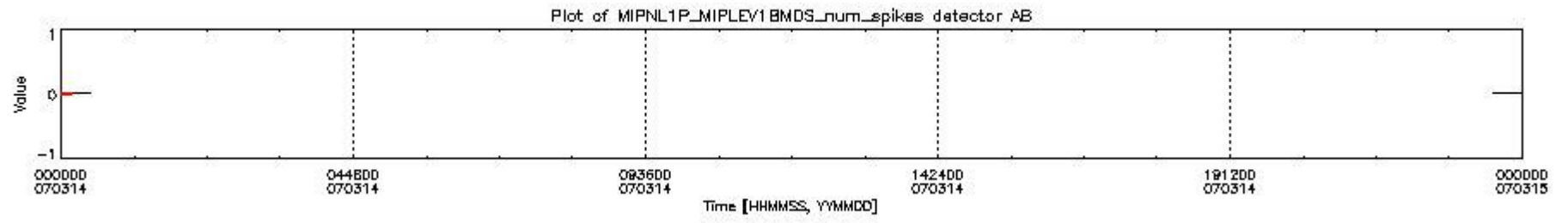
mipas_daily_report_level1_OFL_MIPAS_4_67_P_20070314_20.PNG
