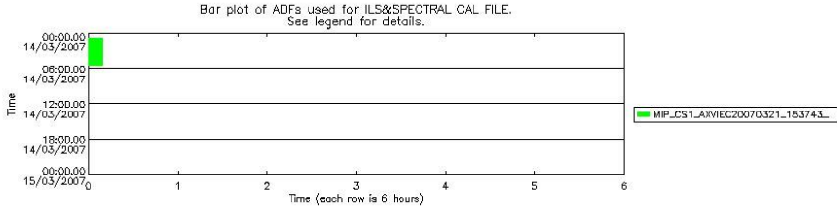
mipas_daily_report_level1_OFL_MIPAS_4_67_P_20070314_55.PNG
