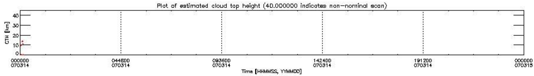
mipas_daily_report_level1_OFL_MIPAS_4_67_P_20070314_53.PNG
