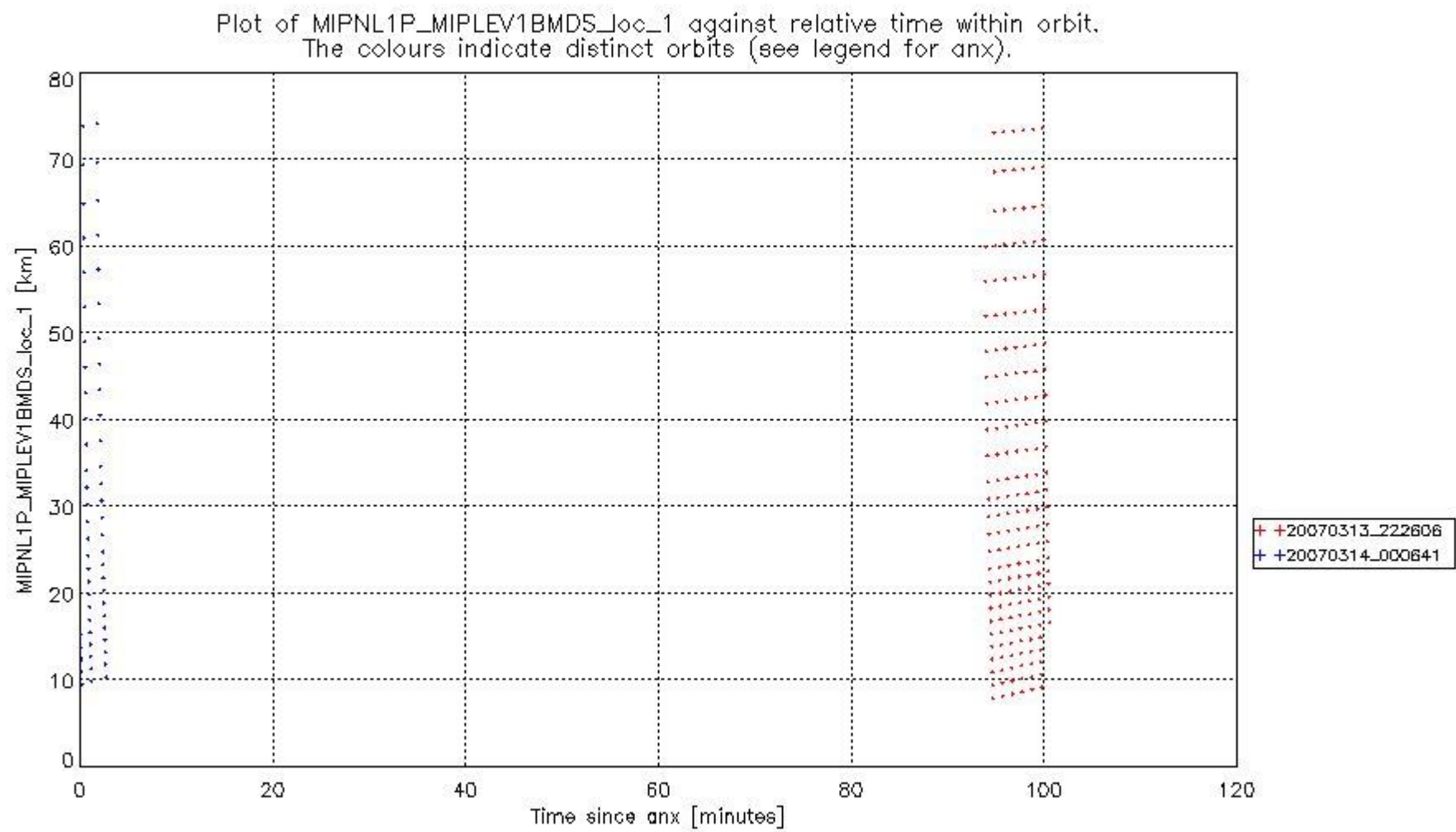
mipas_daily_report_level1_OFL_MIPAS_4_67_P_20070314_52.PNG
