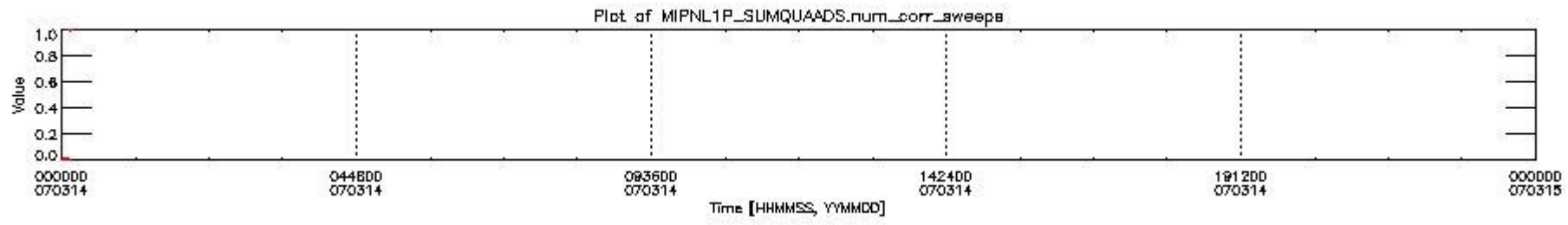
mipas_daily_report_level1_OFI_MIPAS_4_67_P_20070314_2.PNG
