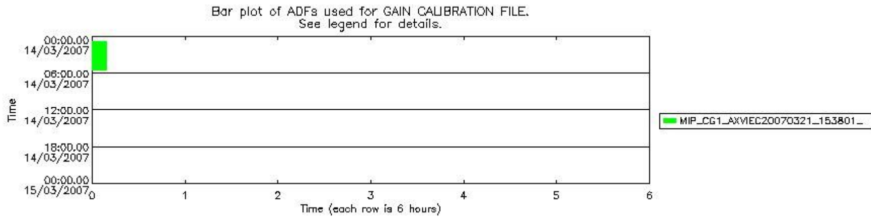
mipas_daily_report_level1_OFL_MIPAS_4_67_P_20070314_56.PNG
