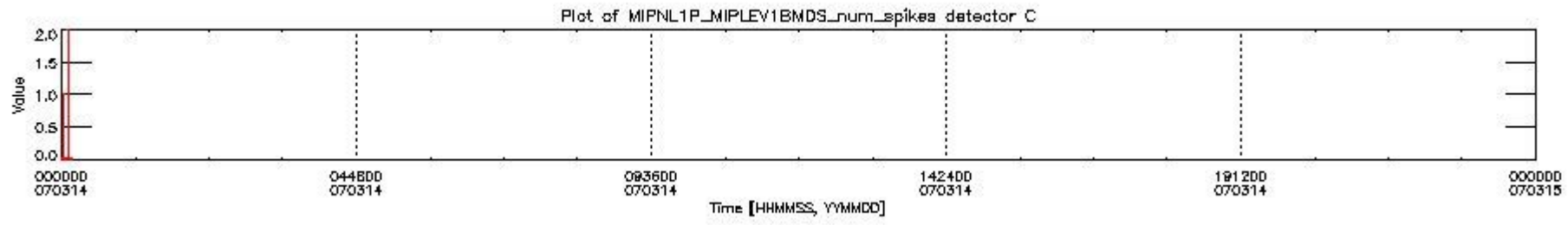
mipas_daily_report_level1_OFL_MIPAS_4_67_P_20070314_24.PNG
