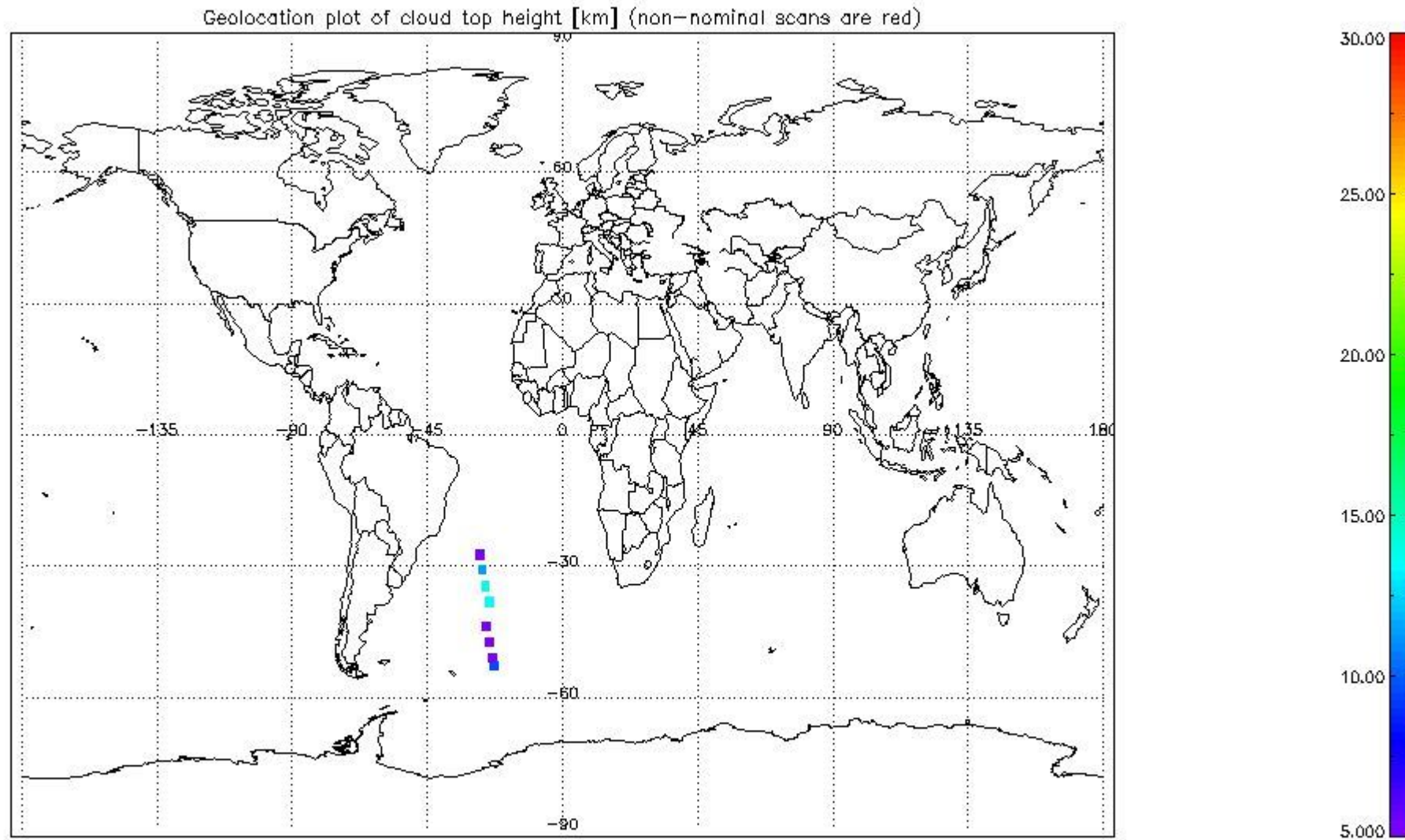
mipas_daily_report_level1_OFL_MIPAS_4_67_P_20070314_53.PNG
