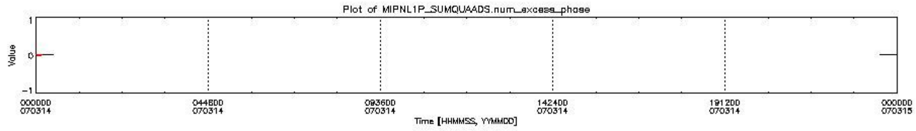
mipas_daily_report_level1_OFI_MIPAS_4_67_P_20070314_8.PNG
